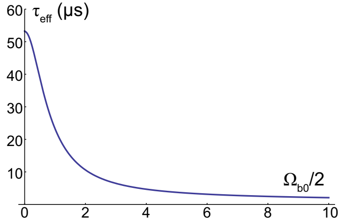
Figure 12.20: Effective susceptibility response time as a function of the blue Rabi frequency. The expression of \tau_{eff} from equation (12.10) is plotted as a function of \frac{\Omega_{b0}}{2} for realistic parameters \Delta = -25 , \delta = 0.3 , \gamma_{13} = 0.15 and \gamma_{33} = 0.0005 (corresponding to a \approx 55 \mu s population lifetime).
