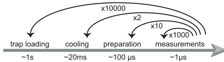
Figure 4.3: Typical sequence behaviour. The measurements themselves are made of short periods ( \sim 1 \mu s ) repeated a large number of times ( \sim 1000 ) which have to be alternated with preparation steps regularly, and maybe integrated into some larger loop of re-cooling the atoms, before having to reload the trap. The generation and data acquisition inside a measurement step must be resolved on \sim 10 ns timescale.
