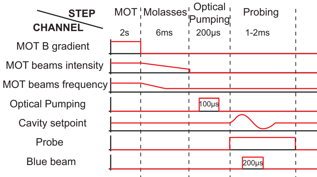
Figure 12.8: Experimental sequence. After trapping the atoms for a few seconds and cooling down to \approx 40 \mu K with optical molasses, they are optically pumped with a 100 \mu s long pulse of intracavity 795 nm light, before the cavity is sent to oscillate. During the first cavity oscillation, in the \approx 200\mu s window in which the transmission line can be observed, the blue beam is shone onto the atoms.
