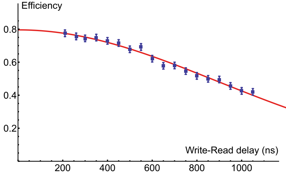
Figure 9.20: Delay dependence of the retrieval efficiency, showing the expected Gaussian Doppler decay.
