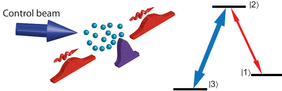
Figure 4: Picture of the propagation of a photon inside a medium as an EIT-polariton. A photon sent in the medium close to the |1\rangle \rightarrow |2\rangle transition, in the presence of the control beam coupling toward the long-lived state |3\rangle , is mapped onto a slow and compressed excitation wave which propagates inside the medium partially carried by the atomic coherences, before exiting it as a photon again.
