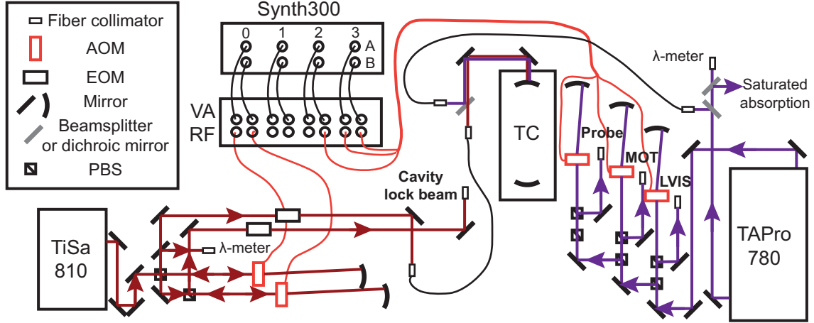
Figure 4.1: Typical setup of beam preparation and control on the laser bench. A typical example is given, restricted to the master laser (TAPro 780) and the 810 nm TiSa, of the way the various beams are prepared, and the use made of RF synthesizers to control AOMs. A locking beam from the 780 laser is used for saturated absorption and locking on the transfer cavity (TC). Various beams (MOT, LVIS, Probe – see next chapter for details) are prepared from the main laser beam, each going through a dedicated AOM. From the 810 TiSa a beam is prepared, shifted by an AOM and modulated by an Electro-Optic Modulator (EOM), then sent to the transfer cavity to lock the laser at an adjustable frequency. The locking beam for the main science cavity (see chapter 6) is produced from this laser, controlled by yet another dedicated AOM. All the AOMs are supplied by digital RF synthesizers (only the Synth300 are shown for the example), which allows us if needed to react dynamically on their frequency and efficiency (analog or digital control, using the variable attenuators VA RF). PBS: Polarizing BeamSplitter.
