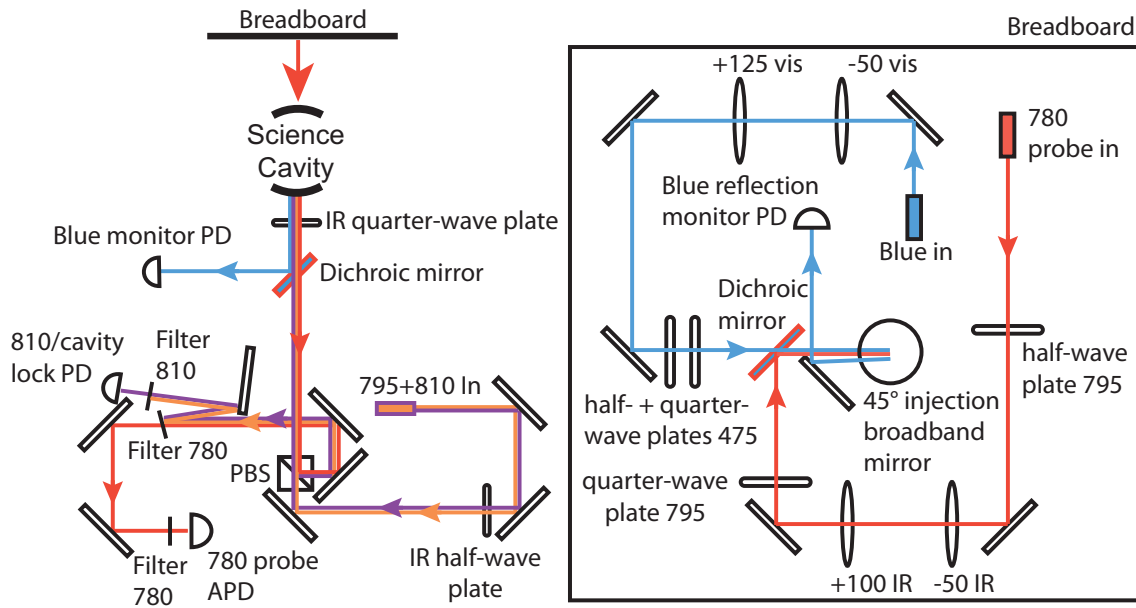
Figure 12.7: Optical layout. Left: Beampaths below the vacuum chamber. The cavity locking beam (810 nm) and the optical pumping (795 nm) are injected through the bottom mirror. A circulator is realized with the PBS and the quarter-wave plate so that light coming out of the cavity is directed towards a different arm. Output light is sorted out by filters, to extract the 810 beam for locking, and the 780 probe transmitted through the cavity to be sent on the APD. The transmitted blue beam is filtered out with a dichroic mirror, and its power can be monitored. Right: Setup on the breadboard, above the cavity and vacuum chamber. The probe and blue beams are mixed together on a dichroic mirror before being injected in the cavity by a broadband mirror (BB1-E02 from Thorlabs) at 45^\circ , through a hole in the breadboard. The blue light reflected by the input viewport of the chamber is sent on a photodiode for monitoring purposes.
