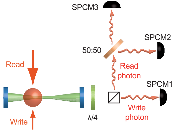
Figure 9.7: Simplified scheme of the experiment in the photon-counting regime.
