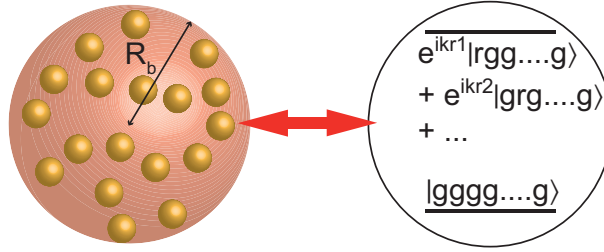
Figure 13.1: Blockaded ensemble acting as an effective two-level system. In the extreme case of an ensemble entirely contained in a blockade sphere of radius R_b , the only two states accessible to the system are the ones where all atoms are in ground state |g\rangle , and the singly-excited state where one Rydberg excitation |r\rangle is shared between all atoms, which keeps a precise phase-matching pattern, allowing for directional light emission.
