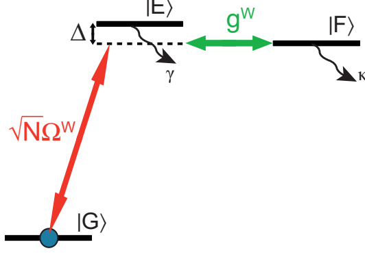
Figure 8.1: \{N \text{ atoms} + \text{cavity field}\} states considered in the treatment of the Write step.
