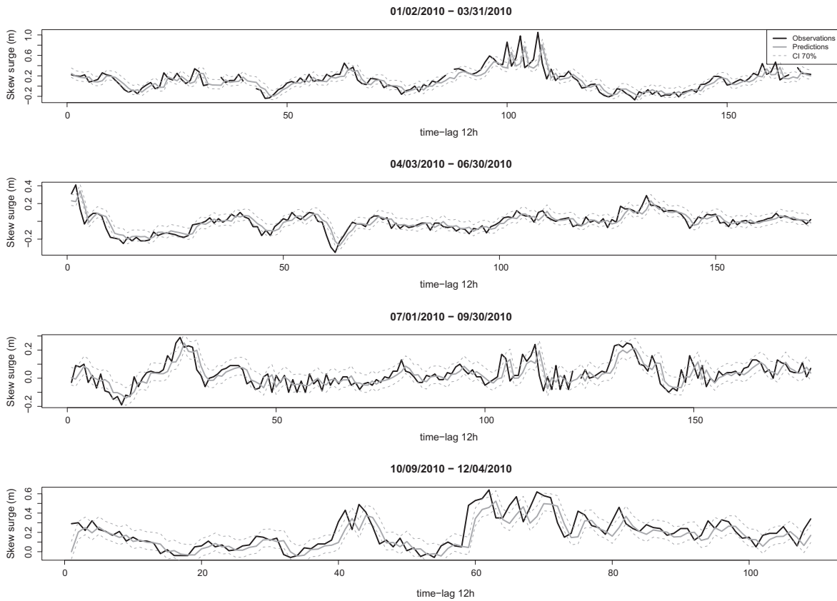
Fig. 13. Optimal one-step ahead forecasts at Saint-Nazaire (France) over the year 2010, with 70% confidence bounds from the NIG distribution of the residuals.
