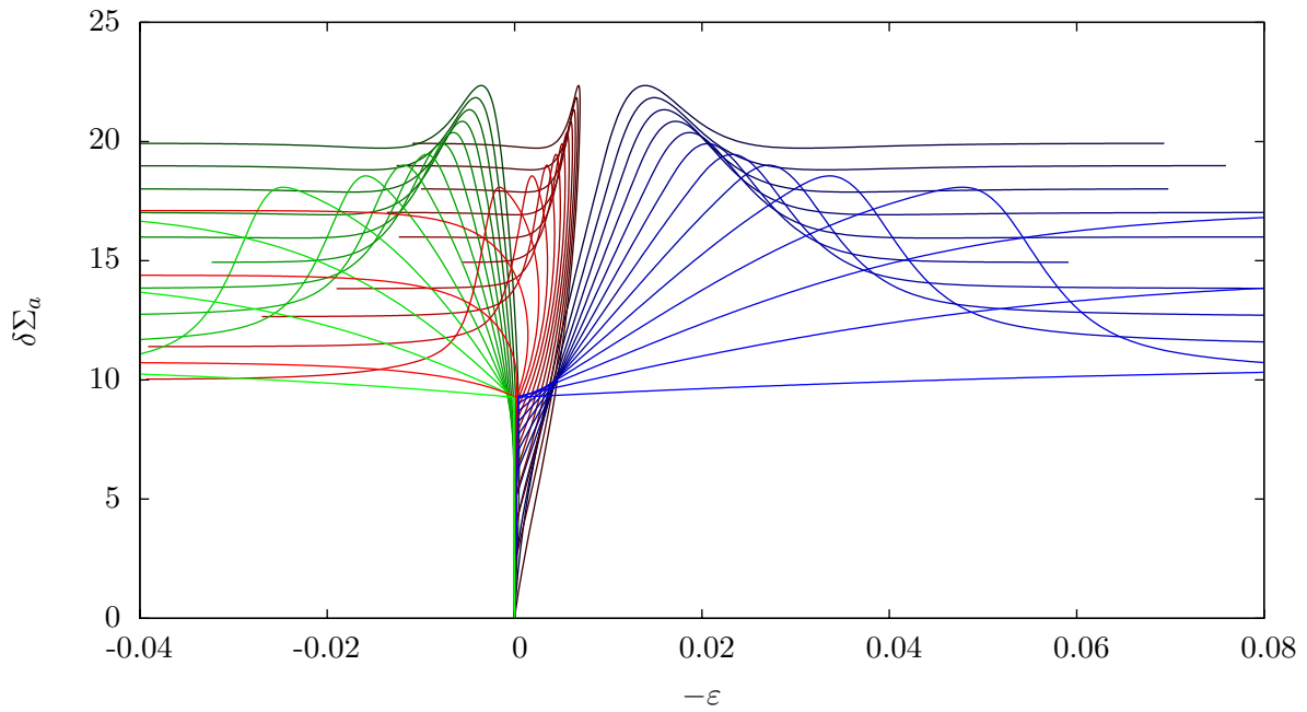
(b) triaxial
