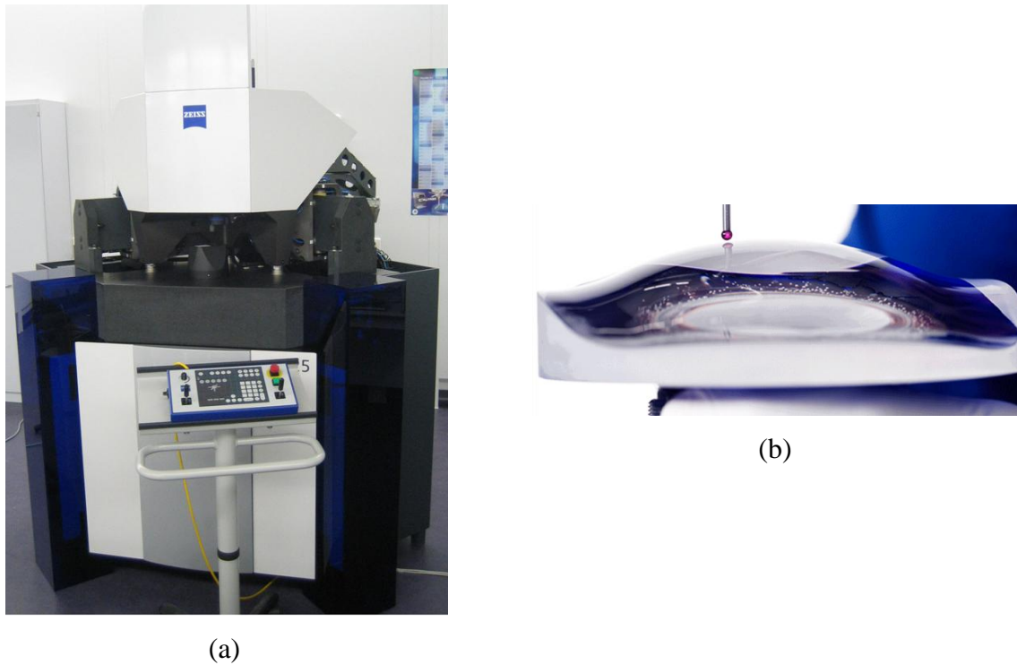
Fig. 32 The F25 \mu CMM. (a) complete apparatus; (b) freeform optical surface measurement using a tactile probe [45].
