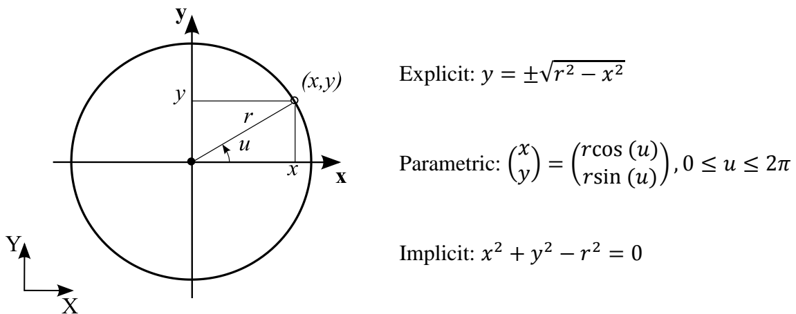
Fig. 144 Explicit, implicit and parametric definitions of a circle.
