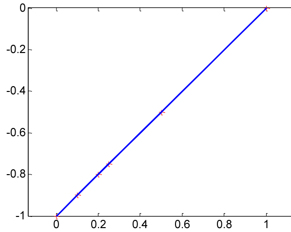
Fig. 113 Degenerate points (red) for a Delaunay triangulation (blue).
