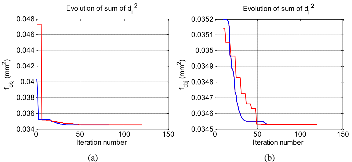
Fig. 91 Evolution of the objective function value through the iterations for the case of \text{TScan}_1 (legend: L-BFGS: blue, LM: red, f_{obj} = \phi ). (a) All iterations; (b) Starting from iteration 10.
