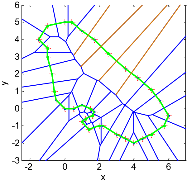
Fig. 140 N.N.I (green) applied on a closed curve represented by the red points. Some bipolar Voronoi edges are highlighted. The reconstruction contains no interior segments.
