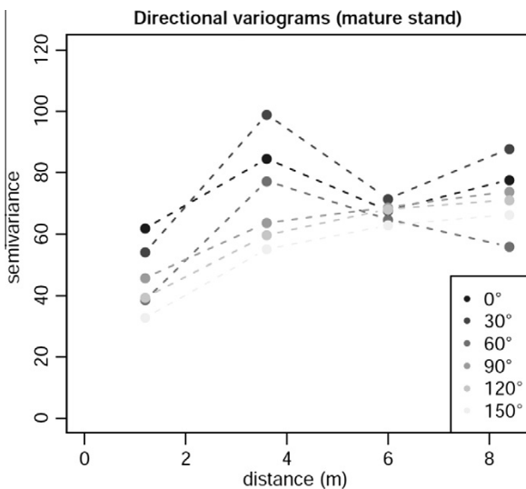
Fig. 5. Directional variograms for six directions in the mature semi-natural stand.
