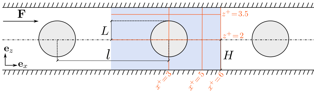
Figure 4.8: Infinite array of cylinders in a channel: sketch of the geometry with l^+ = 6 [30, 78]. The orange lines correspond to the profiles plotted in Figure 4.10 ( x^+ = 3, 5, 6 and z^+ = 2, 3.5 ).
