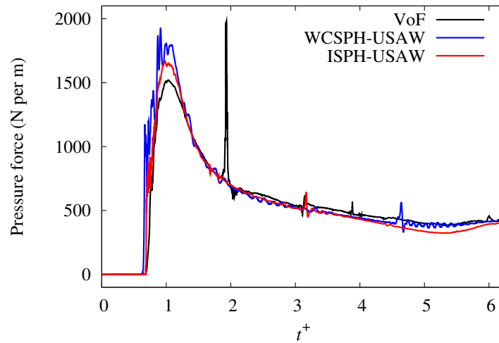
Figure 4.14: Dam-break over a wedge. Comparison of the evolution of the pressure force applied on the left-side of the wedge between VoF (6322 cells), ISPH-USAW (5881 particles) and WCPH-USAW (5881 particles).
