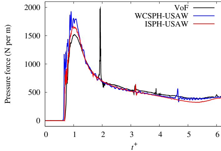
Figure 4.14: Dam-break over a wedge. Comparison of the evolution of the pressure force applied on the left-side of the wedge between VoF (6322 cells), ISPH-USA (5881 particles) and WSPH-USA (5881 particles).
