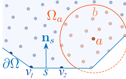
Figure 2.8: Sketch of the continuous medium discretisation with the USAW boundary conditions technique.
