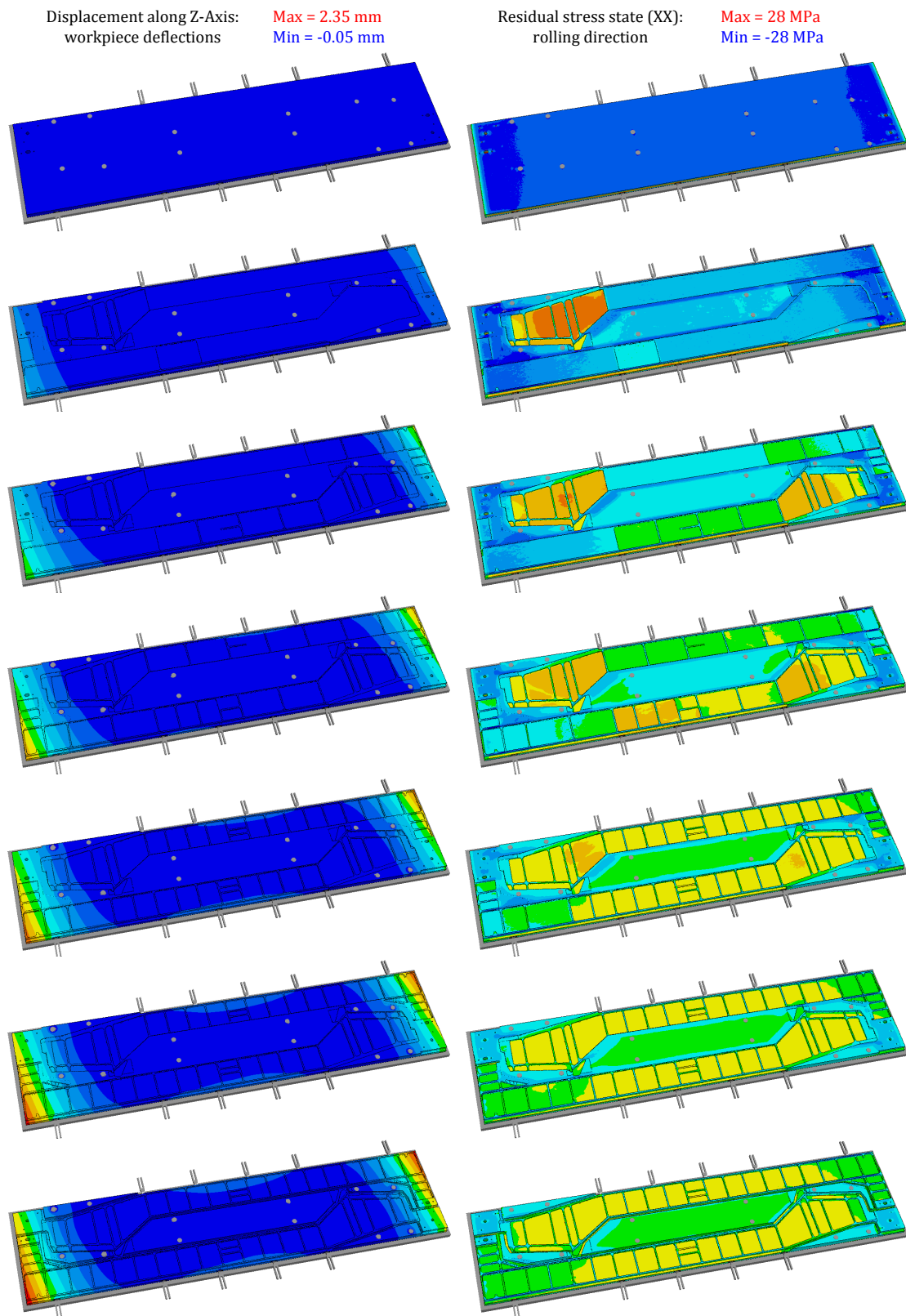
Figure 5.10: Evolution of the deflections and stress state of the workpiece during the first machining step
