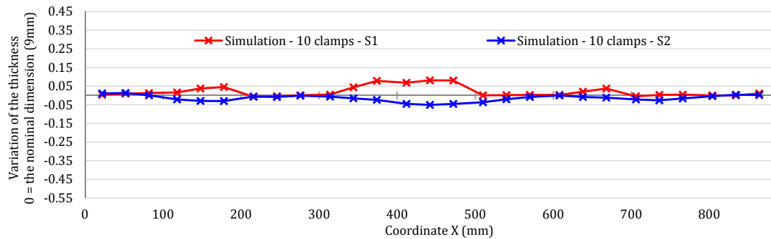
Figure D.4: Thickness variations of the wall with a nominal dimension of 9 mm with the fixture layout with ten clamps and two different machining sequences
