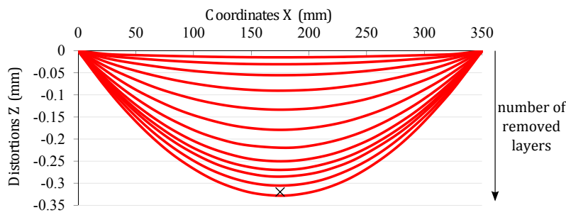
Figure 3.15: Evolution of the curvature of the 70 mm thick specimen during the twelve removals of layers. The cross represents the maximum displacement observed experimentally after the twelfth layer removal.
