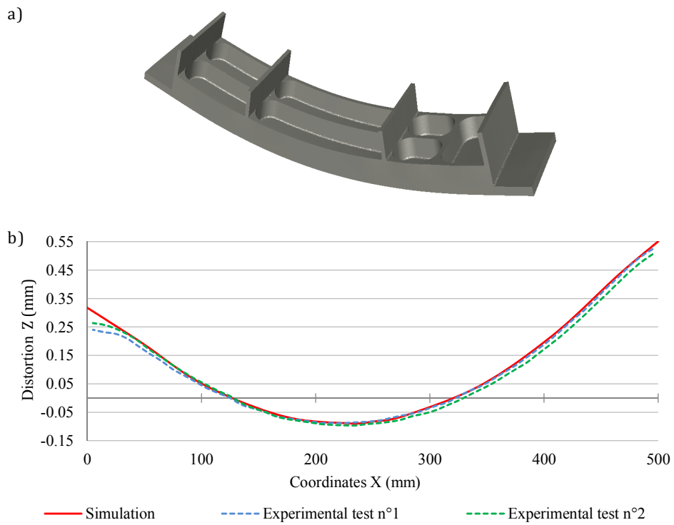
Figure C.3: The post-machining distortion of the part: a) The machined part with amplified distortion ; b) Comparison between experimental and simulation distortion
