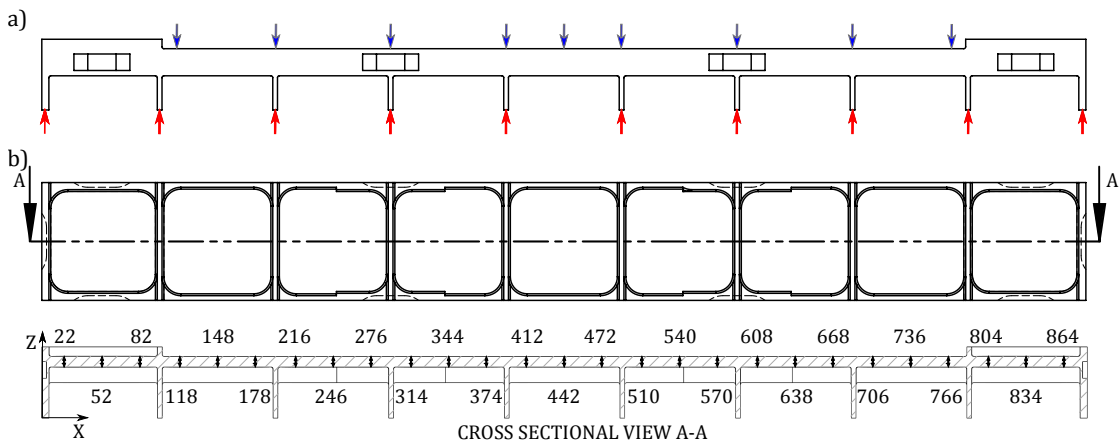
Figure 4.6: Representation of the measurements performed for the machining quality evaluation. The arrows represent the measurement zones: a) Post-machining distortion measurements on the top and bottom surfaces of the part ; b) Coordinates for thickness measurements of the wall with a nominal value of 9 mm
