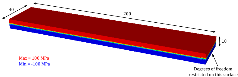
Figure 2.7: The geometry and its initial stress state used for the comparison between FORGE ® and Abaqus
