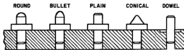
Figure 1.19: Examples of locators [73]
