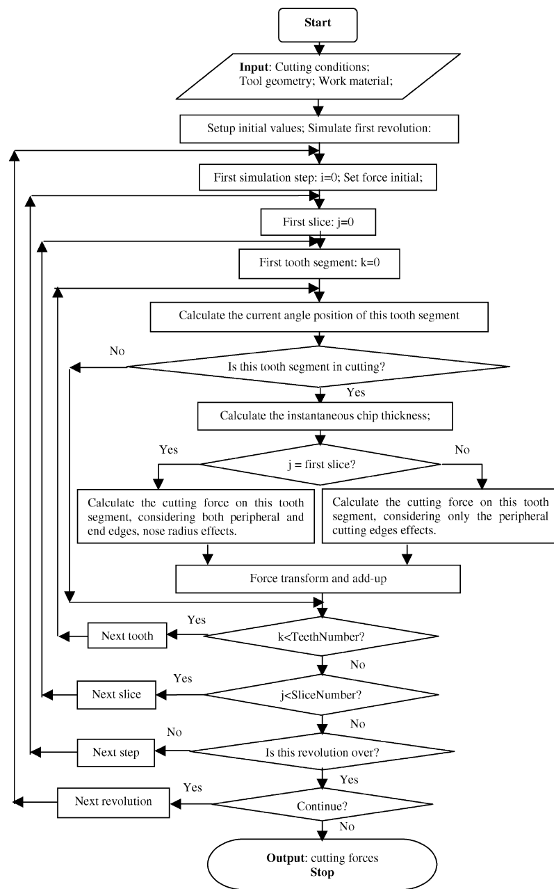
Figure 1.11: Flowchart of the simulation system proposed in [52]
