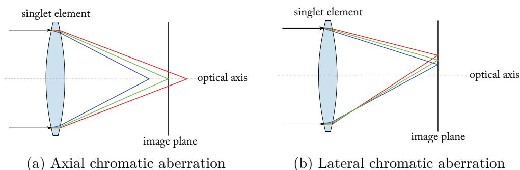
Figure 4.1: Occurrence of axial (a) and lateral (b) chromatic aberrations.
