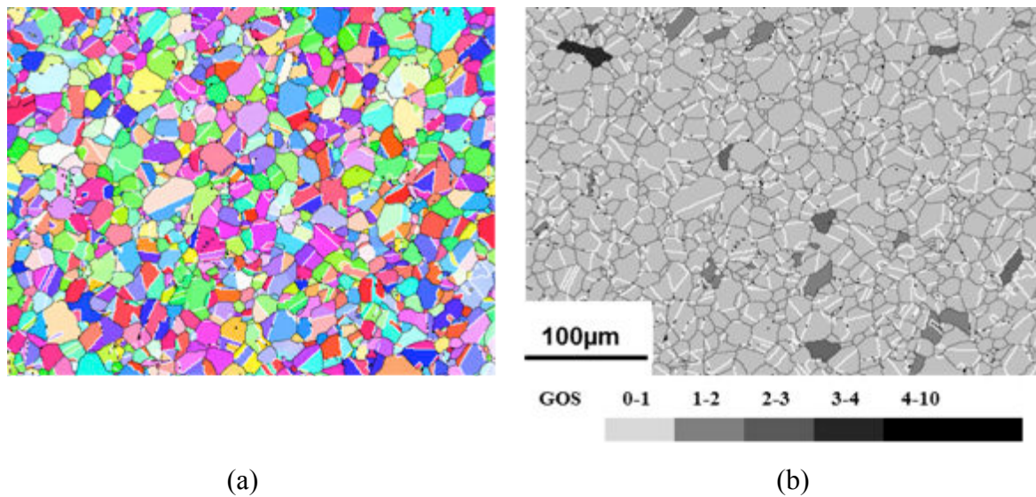
Fig. 2.22. The initial microstructure: a) same colour code as in Fig. 2.21, b) the corresponding Grain Orientation Spread (GOS) map; Grain boundaries in black and twin boundaries \Sigma 3 in white.
