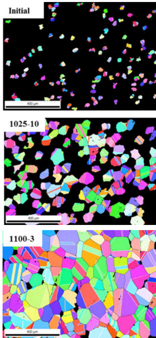
Fig. 2.25. The 100 biggest grains in the microstructures (same colour code as in Fig. 2.20).
