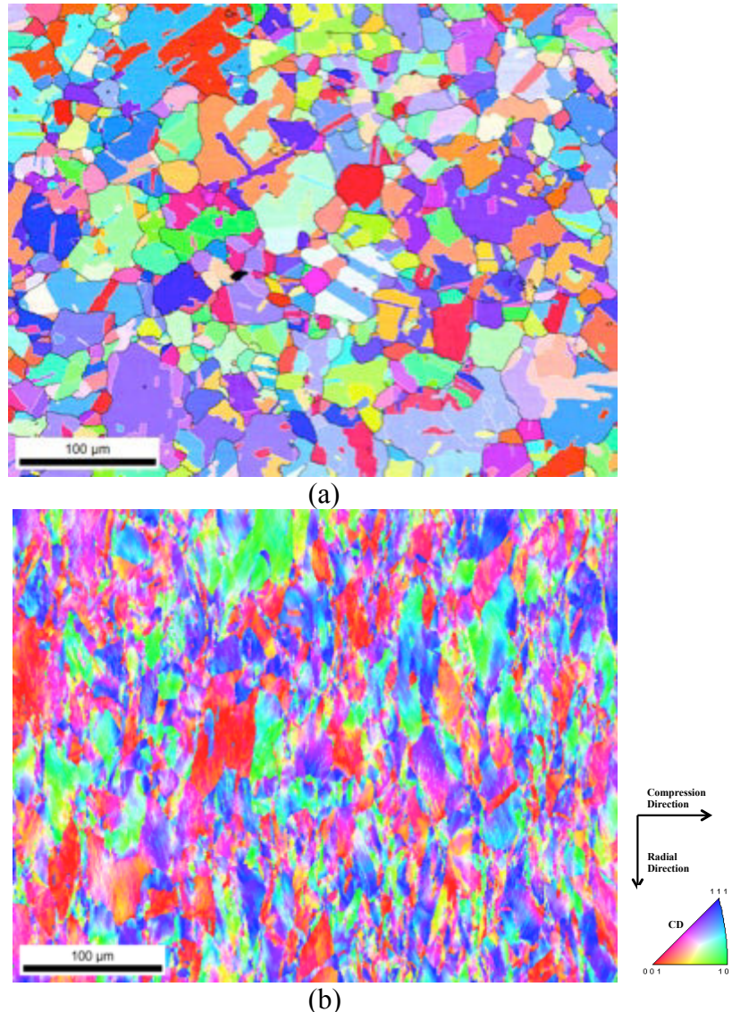
Fig. 3.6. EBSD map of the state of the material before (a) and after (b) 50% height reduction by compression at room temperature.
