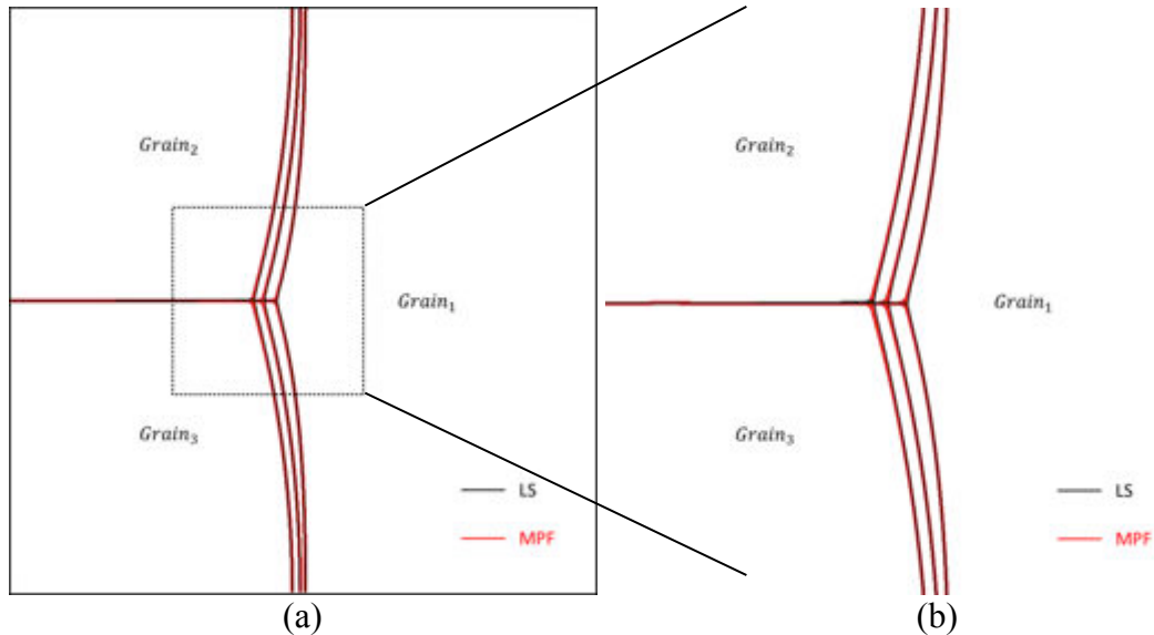
Fig. 6.6. First \gamma -set: (a) comparison between the simulation results obtained by the LS approach ( h_{fine} = 2 \times 10^{-3} \text{ mm} , dt=40\text{s} ) and the MPF approach ( h_{fine} = 1.3 \times 10^{-3} \text{ mm} , dt=2\text{s} ) at t = 16\text{h}40\text{min} , 25\text{h} , and 33 \text{ h}20 \text{ min} ; (b) Zoom of (a) at the triple junction.
