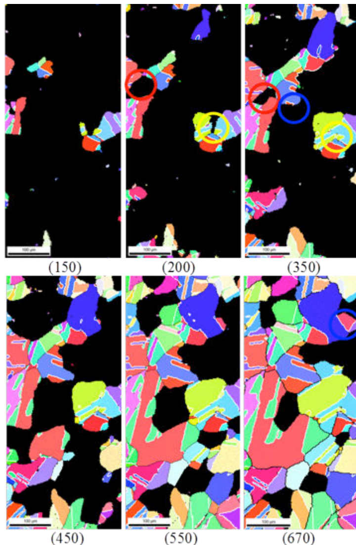
Fig. 2.15. Recrystallized grain evolution in sample 1; cumulative annealing time (s) are indicated below each map (same color code as in Fig. 2.14); white lines denote \Sigma 3 boundaries; black lines denote high angle boundaries defined by a disorientation angle above 5^\circ .
