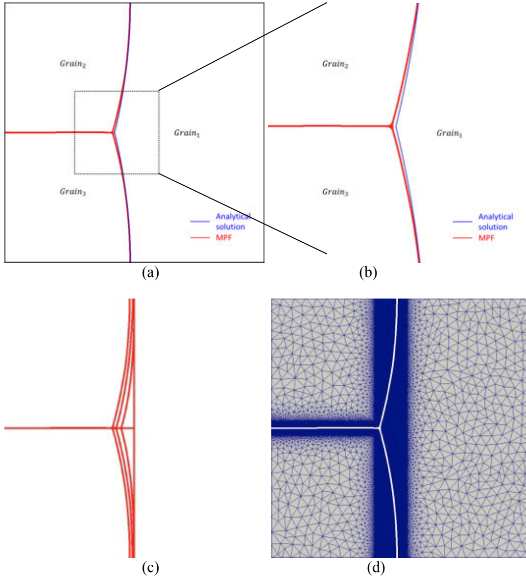
Fig. 6.3. First \gamma -set: solution of the three-grain problem obtained by the MPF approach. System parameters: \lambda = 2 \times 10^{-2} mm , dt = 3s . (a) MPF solution (at t = 33 h20 min ) compared with the analytical solution. (b) Zoom of (a) at the triple junction. (c) Evolution of the simulated structure at t = 16h40min , 25h , and 33 h20 min . (d) Snapshot of the used FE mesh (fixed with h_{fine} = 2 \times 10^{-3} mm , h_{coarse} = 4 \times 10^{-2} mm , E = 0.22 mm ), the profile corresponds to the simulate structure at t=33h20min .
