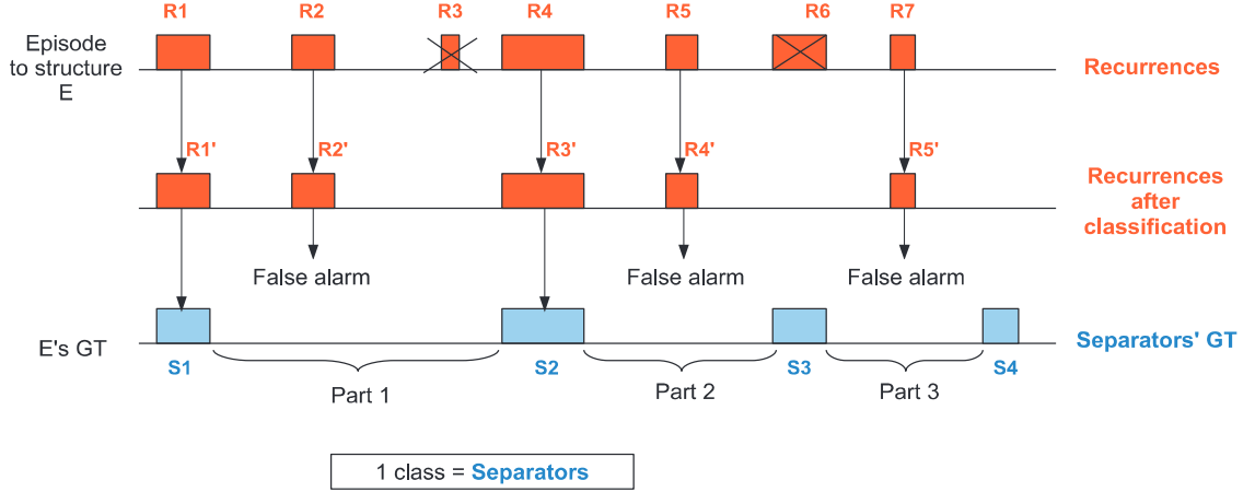
FIGURE 4.5: Separators' Ground-Truth.
