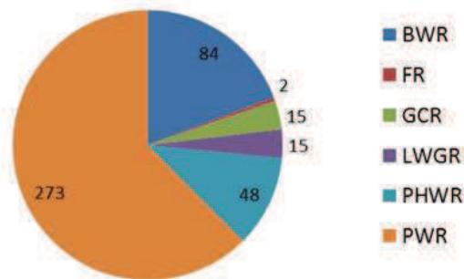
Figure 1: Distribution du type de réacteurs du parc mondial en 2013 (BWR: boiling water reactor; FR: fast reactor; GCR: gas cooled reactor; LWGR: light water cooled, graphite moderated reactor; PHWR: pressurized heavy water reactor; PWR: pressurized water reactor) [AIEA 2013]
