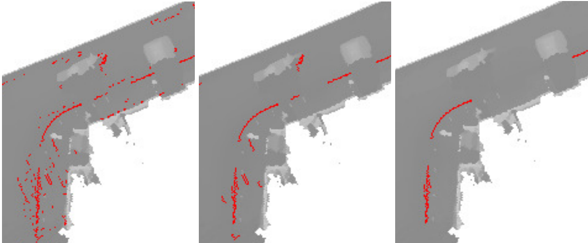
(b) E_{min}=0
