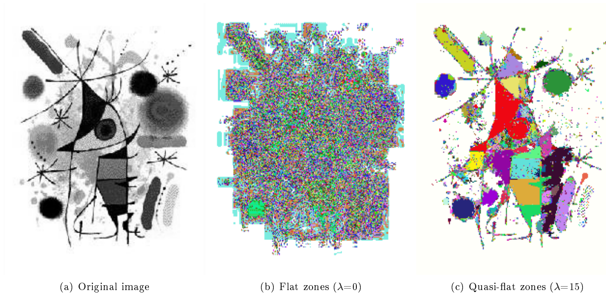
Figure 7.1: Example of flat and quasi-flat zones on a gray level image. Each color represents a segment in the partition. This is very useful for image partition, simplification and segmentation.
