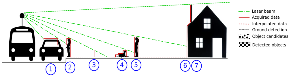
(a) Acquisition scheme and interpolated profile \hat{f} .
