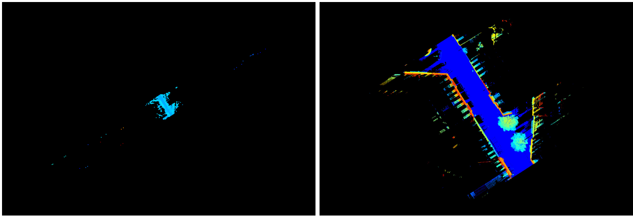
(a) Elevation image from the original point cloud. Image size: 7523 \times 4206 = 31.6 \times 10^6 pixels (b) Elevation image after filtering distant points in the input point cloud. Image size: 1131 \times 952 pixels = 1.1 \times 10^6 pixels
