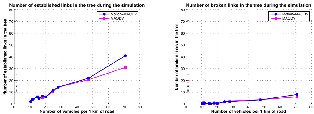
FIGURE 4.17: Number of Established and broken links in the tree during the simulation
