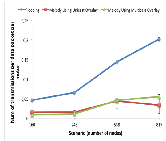
FIGURE 5.9: Number of packet transmissions per Meter
