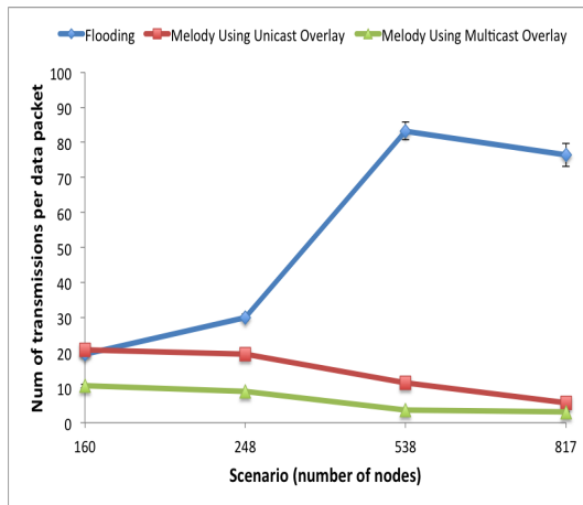
FIGURE 5.8: Number of packet transmissions
