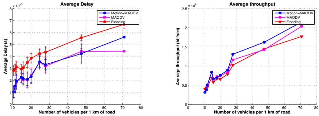
FIGURE 4.15: Average Delay and throughput of MAODV, Motion-MAODV and Flooding
