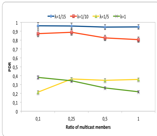
FIGURE 5.11: Packet Delivery Ratio of Melody using Multicast relay path
