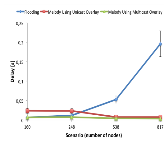
FIGURE 5.13: End-to-End Delay of Melody compared to Flooding
