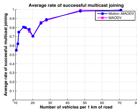
FIGURE 4.16: Average Successful Join Rate of MAODV and Motion-MAODV
