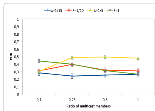
FIGURE 5.10: Packet Delivery Ratio of geographic Flooding per multicast receivers' rate
