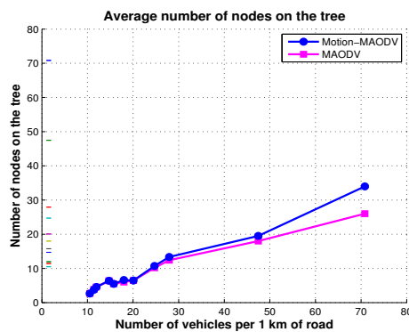
FIGURE 4.18: Average number of nodes on the tree in MAODV and Motion-MAODV
