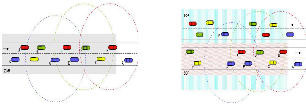
FIGURE 2.7: Zone Of Relevance and Zone Of Forwarding in geocast Type of dissemination
