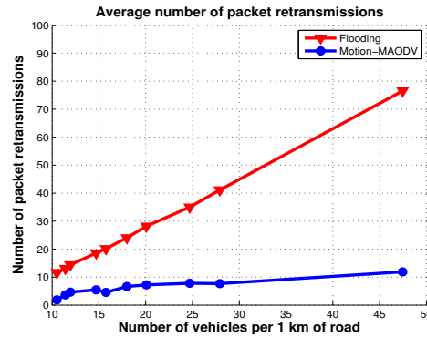
FIGURE 4.14: Average Packet retransmissions of Motion-MAODV and Flooding
