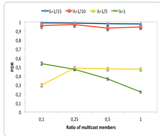
FIGURE 5.12: Packet Delivery Ratio of Melody using Unicast relay path
