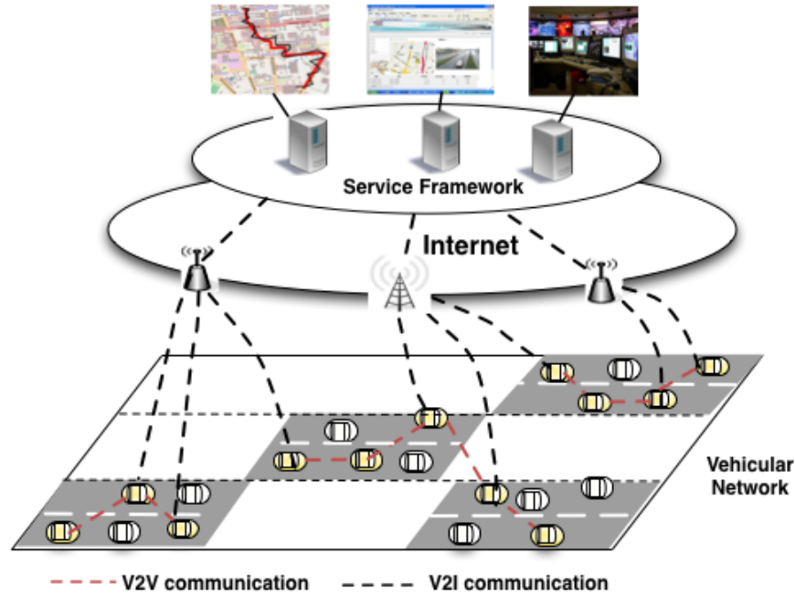
FIGURE 2.2: V2V and V2I communications in vehicular networks
