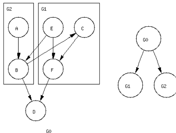
Fig. 6-9 A multilevel graph using sub_graph structure in BGL
