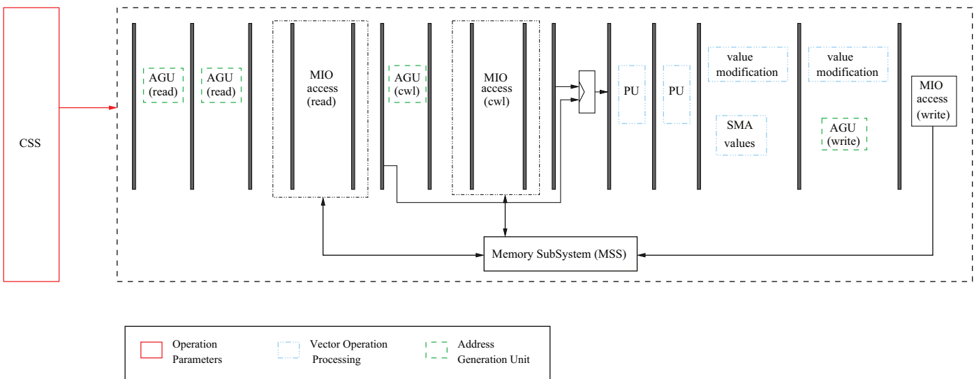
Figure 4.4: C-FEEP Architecture
