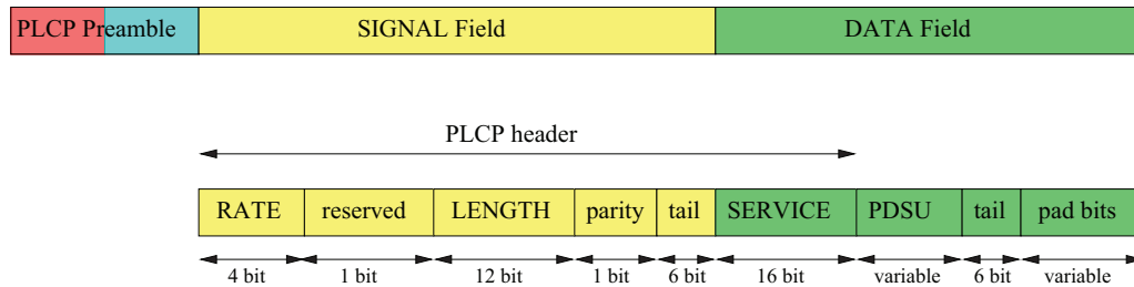
Figure 3.2: IEEE 802.11p Packet Structure
