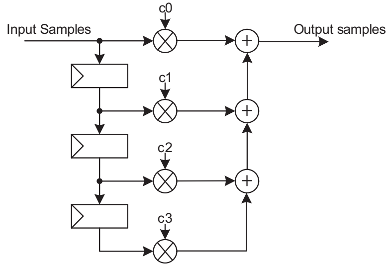
Figure 5.15: Example FIR Filter with 4 Filter Coefficients
