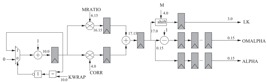
Figure 5.14: Module InterpolationControl
