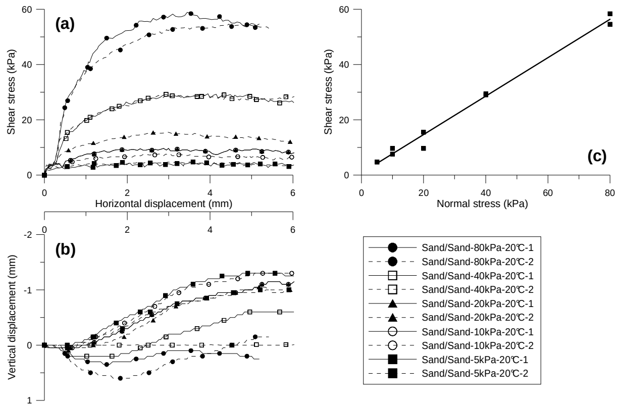
Figure 4.8 Experimental results on Fontainebleau sand at 20^\circ\text{C} : (a) shear stress versus horizontal displacement; (b) vertical displacement versus horizontal displacement; (c) shear strength envelope
