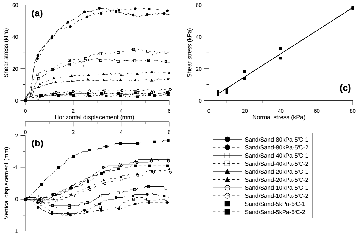
Figure 4.7 Experimental results on Fontainebleau sand at 5^\circ\text{C} : (a) shear stress versus horizontal displacement; (b) vertical displacement versus horizontal displacement; (c) shear strength envelope
