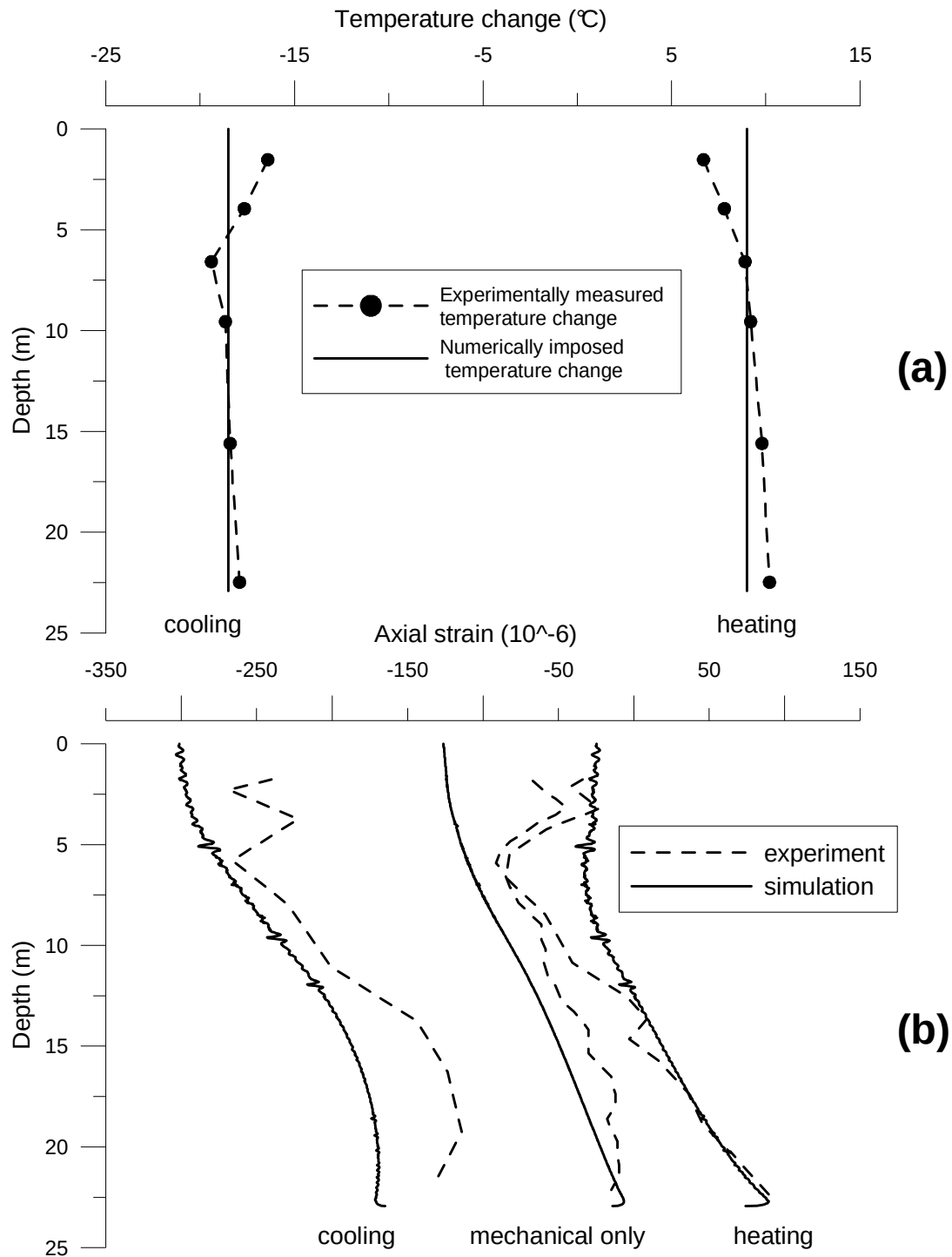
Figure 5.6 Results of London test: (a) profile of temperature along the pile; (b) pile axial strain distribution
