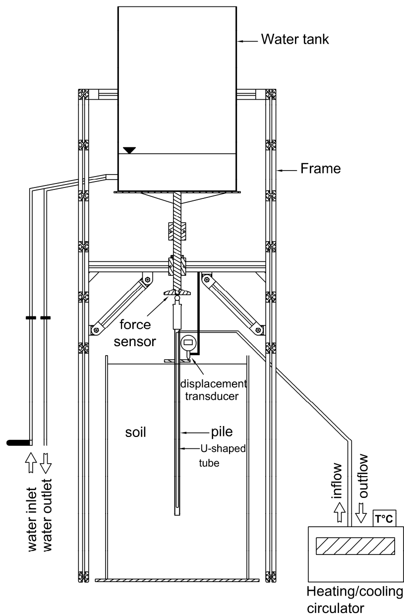
Figure 2.1 Experimental setup
