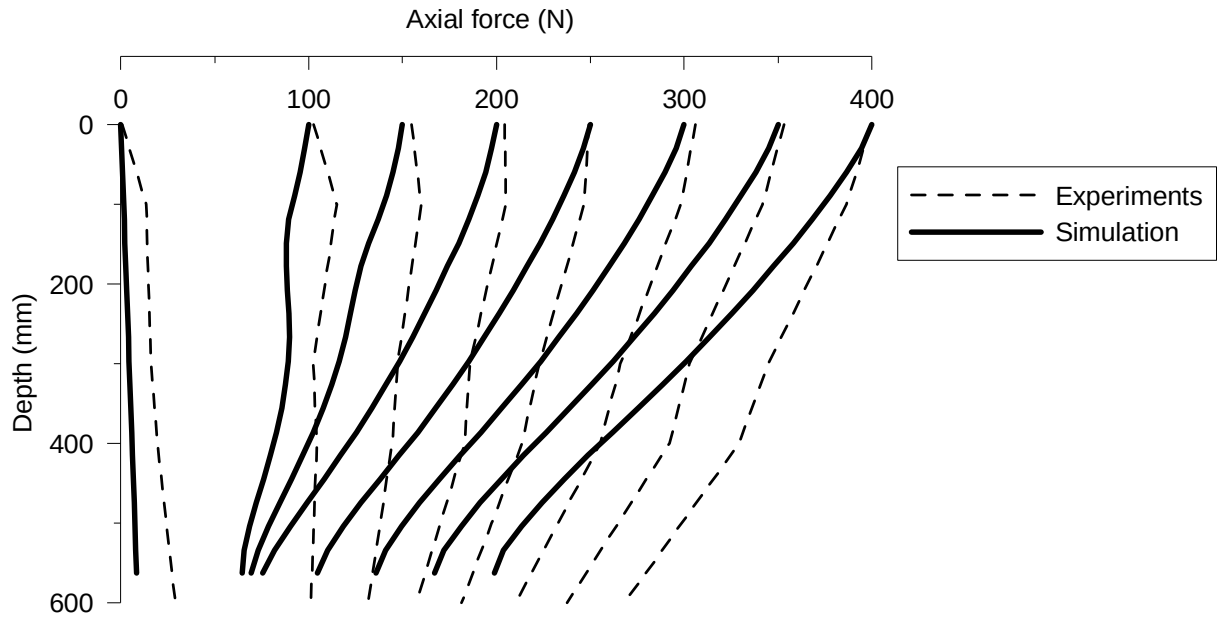
Figure 5.13 Axial force distribution along the pile (test E1)
