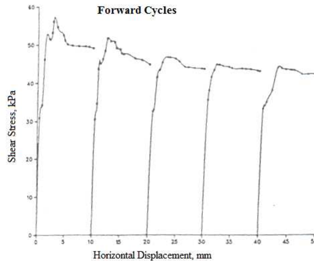
Figure 1.7 Stress-displacement relationship for kaolin/kaolin interface (Rouaiguia, 2010)
