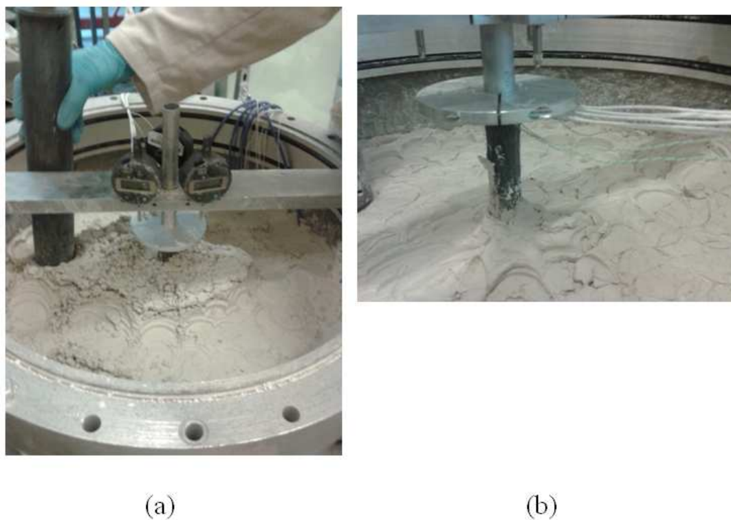
Figure 2.20 (a) Last stages of clayey soil compaction (b) Final soil surface
