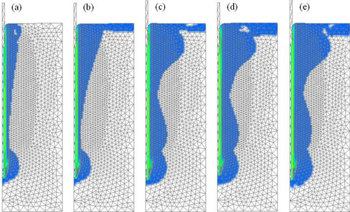
Figure 5.22 Plastic zone evolution under 300 N at the end of : (a) purely mechanical phase (b) first cooling phase (c) first heating phase (d) second cooling phase (e) second heating phase. In all subfigures, the mesh is deformed according to displacements (amplification factor = 500).
