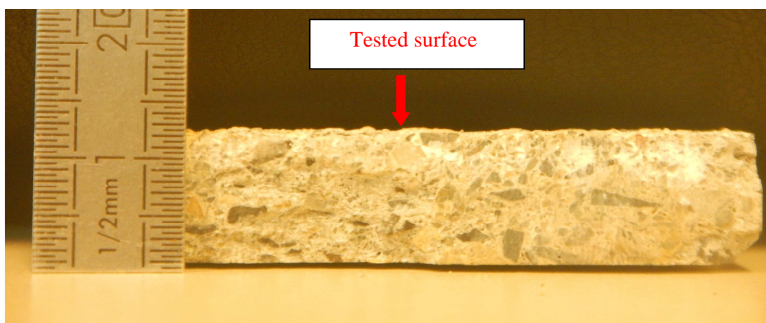
Figure 4.3 Concrete plate used for studying clay/concrete interface
