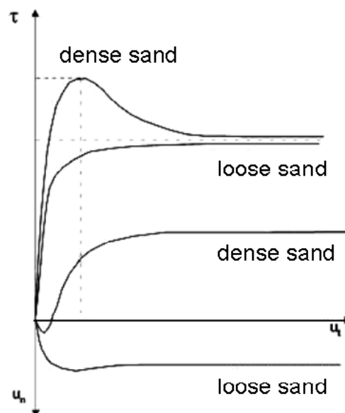
Figure 1.4 Typical interface response (Said, 2006)
