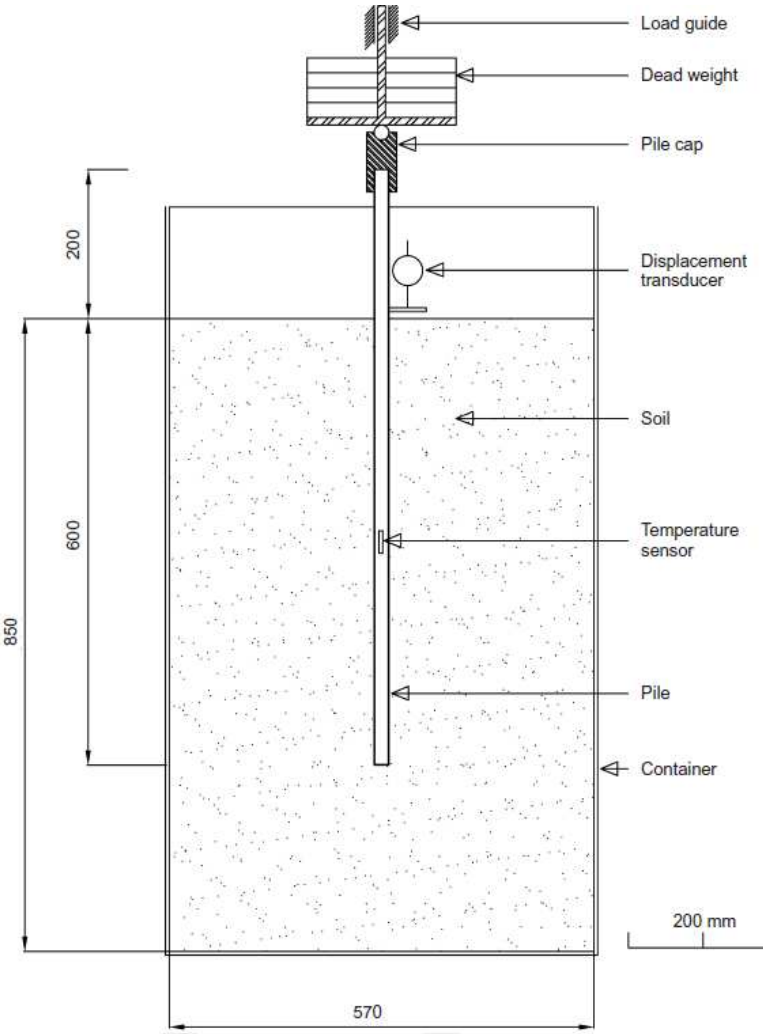
Figure 1.24 Experimental set-up (Kalantidou et al. , 2012)
