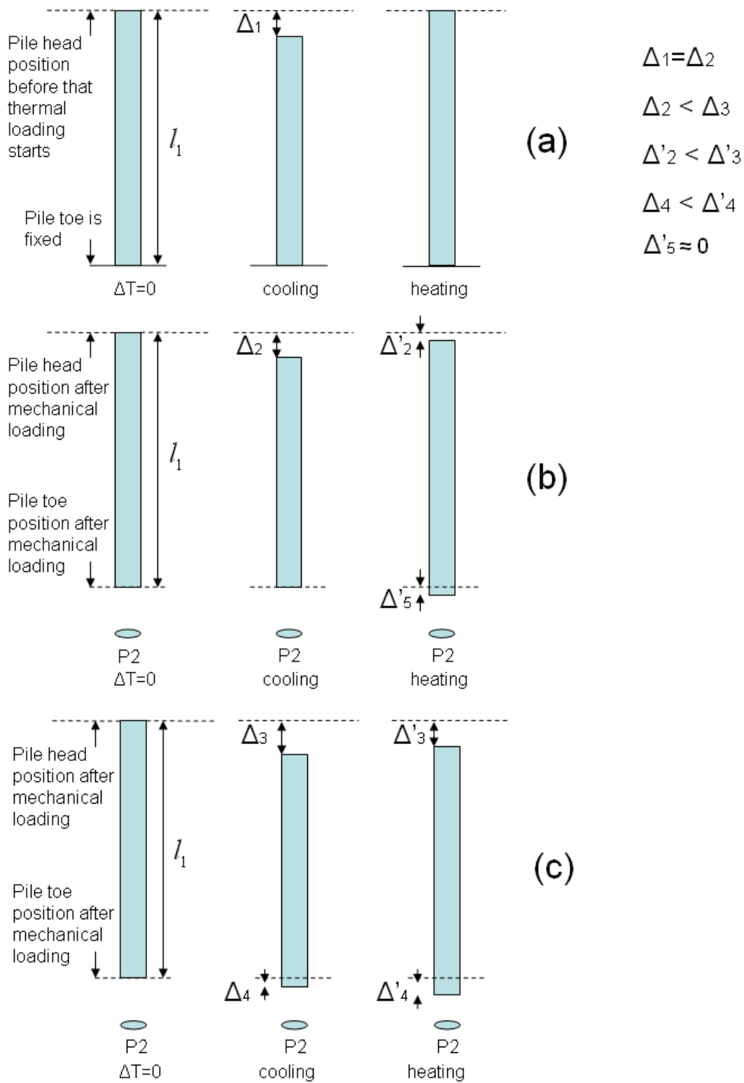
Figure 5.28 Prospective mechanisms for pile behaviour under a load less than 200N and a thermal cycle: (a) a free pile (b) pile in the simulations (c) pile in the experiment
