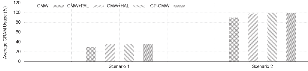
Figure 8.13: The average GRAM usage rate:
