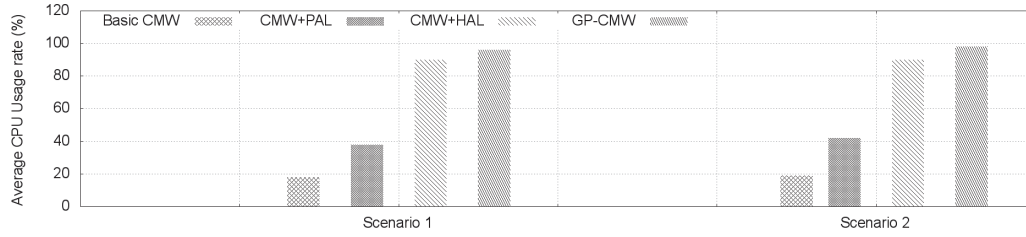
Figure 8.10: The average CPU usage rate:
