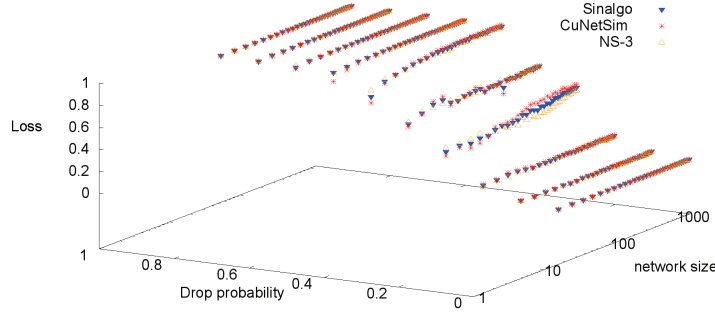
Figure 6.5: End-to-End Packet Loss:
