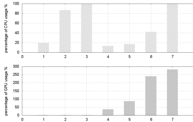
Figure 7.6: The hardware usage rate.
