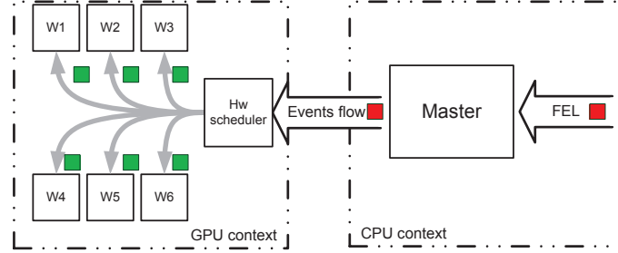
Figure 6.2: Simplified master/workers model that targets GPU execution.
