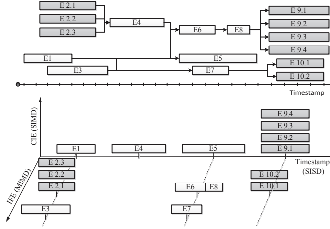
Figure 7.1: Events reordering and storage: top figure schematizes an events dependency diagram while bottom figure schematizes how they will be reordered and stored. Events dependency is transformed to interval.
