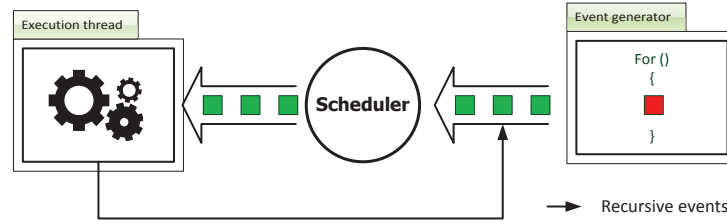
Figure 9.1: Default NS-3 events scheduling approach:
