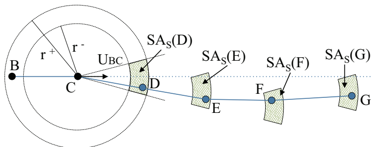
Figure 2.5 – Sample-Based Threshold compression. Using the last two points in the sample ( B and C ) and the user-provided thresholds ( dv and d\varphi ), a safe area ( SA_S(D) ) is calculated for the inspected point D . If the point is within the perimeters of this area, then it is considered as well-predicted and is discarded. Otherwise, the point is inserted into the sample. Figure adapted from [45].
