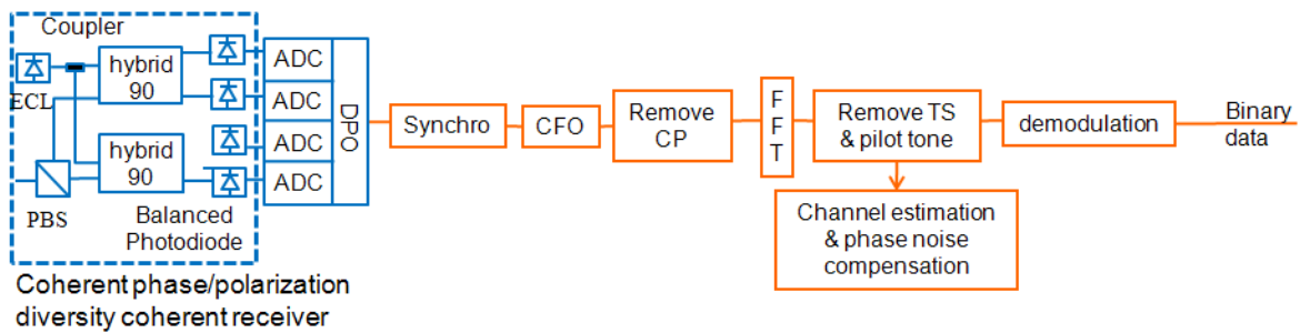
Figure 4-20: Receiver set-up for experimental validation with heterodyne detection.
