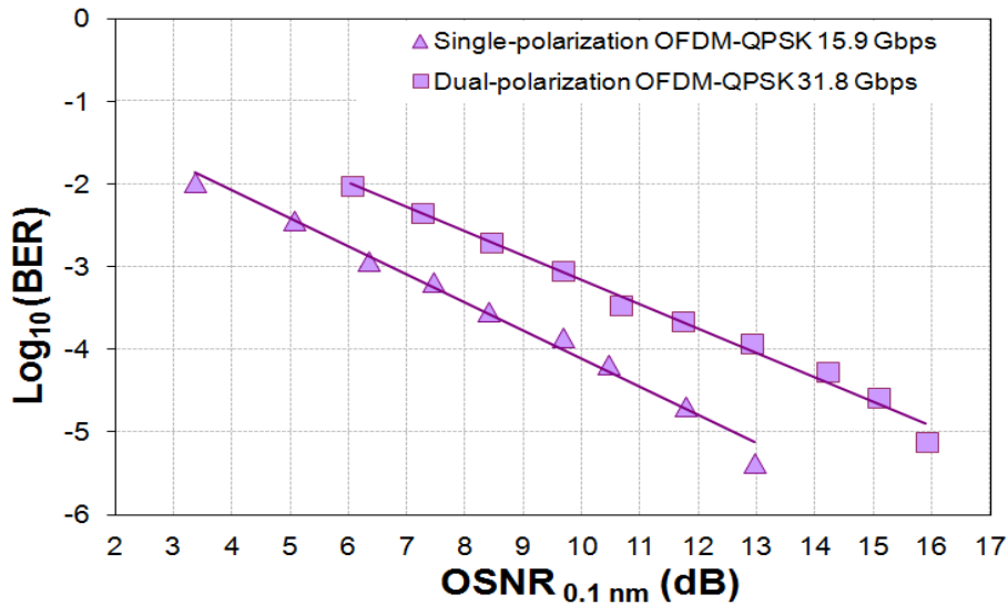
Figure 4-19: BER vs. OSNR for single and dual polarization OFDM signal.
