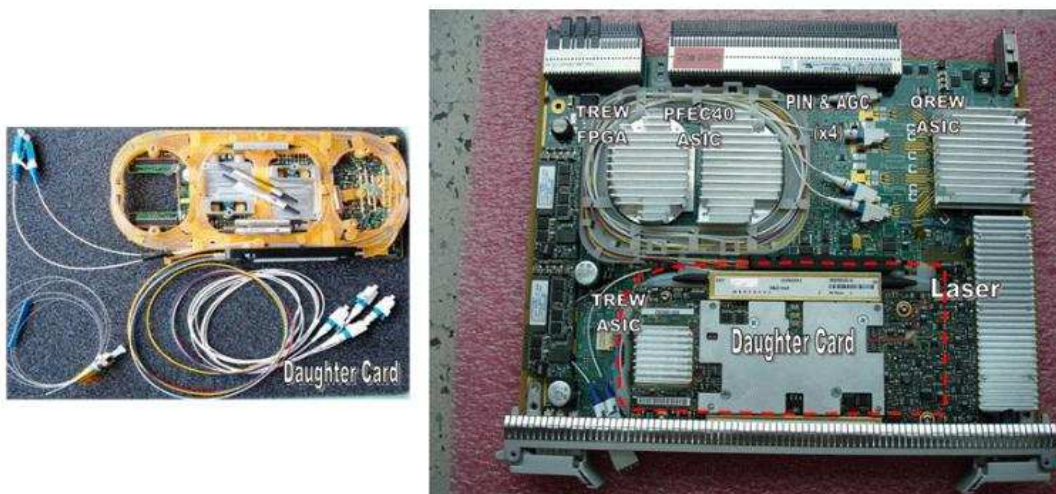
Figure 2-4: 40 Gbps coherent DP-QPSK transceiver card [Sun08].
