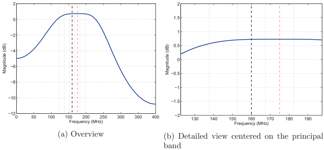
Figure III.20: Frequency response of the STF of the secondary modulator
