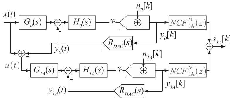
Figure III.22: The general CT MSNBC Architecture
