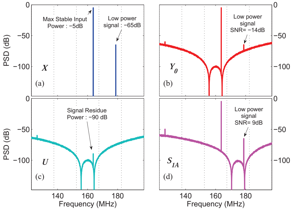
Figure III.16: Simulated output spectra of the architecture
