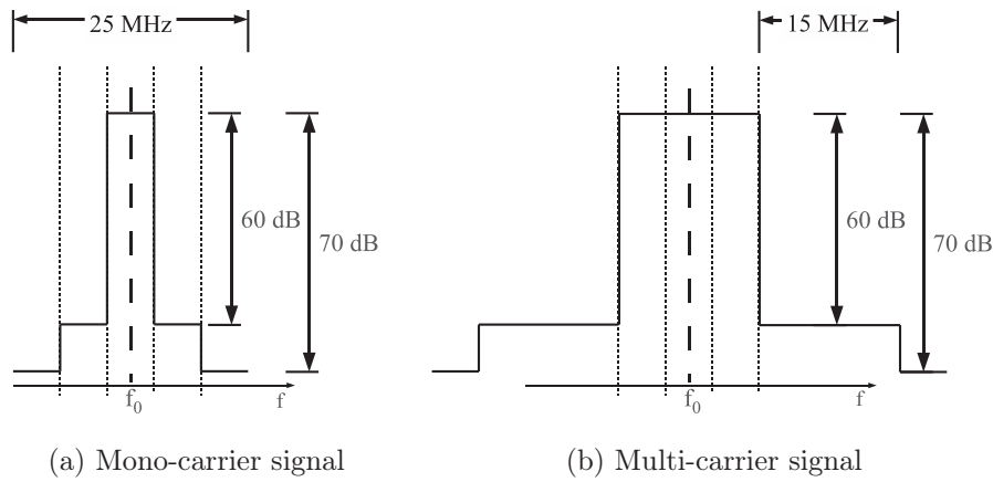
Figure I.18: Expected ACLR Spectrum diagram for the ADC specifications
