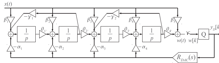
Figure II.10: A 4-th order CT-CIFB modulator
