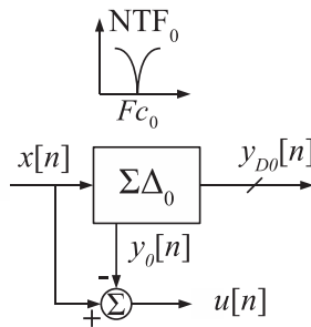
Figure III.6: RSTF definition — General diagram
