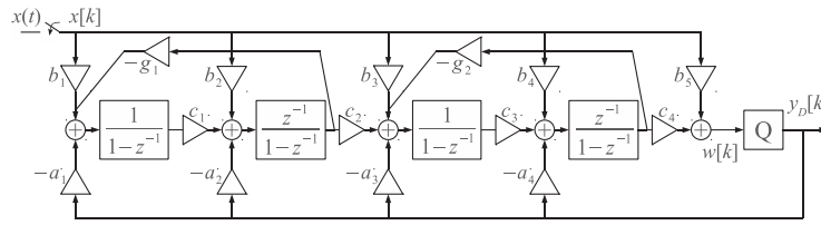
Figure II.9: A 4-th order CRFB modulator
