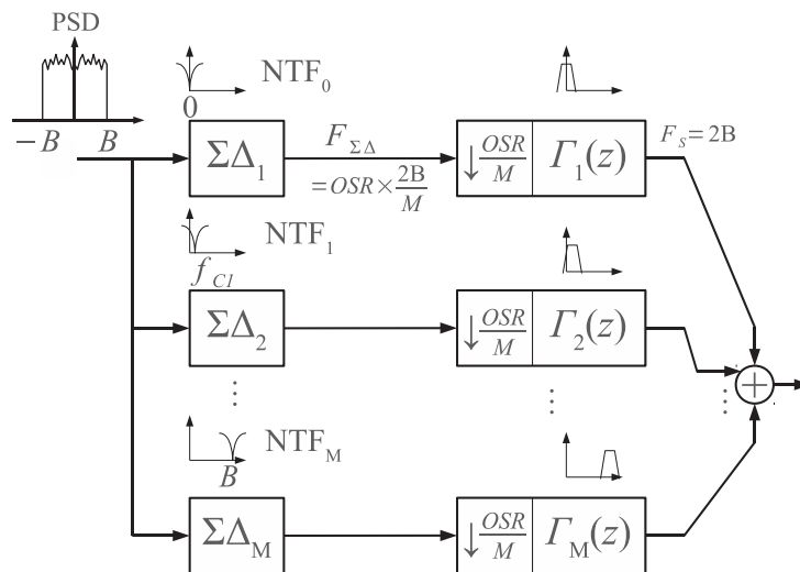
Figure II.16: The Frequency Band Decomposition \Sigma\Delta architecture
