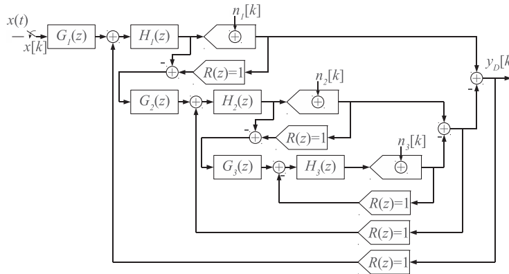
Figure II.14: A Generalized MSCL Modulator
