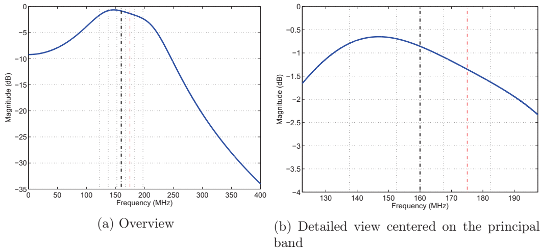
Figure III.24: Frequency response of the estimated STF of the secondary modulator
