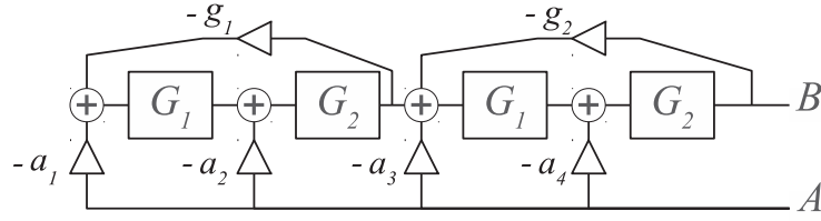
Figure D.2: 4-th order CRFB modulator in open loop configuration for the parameters estimation
