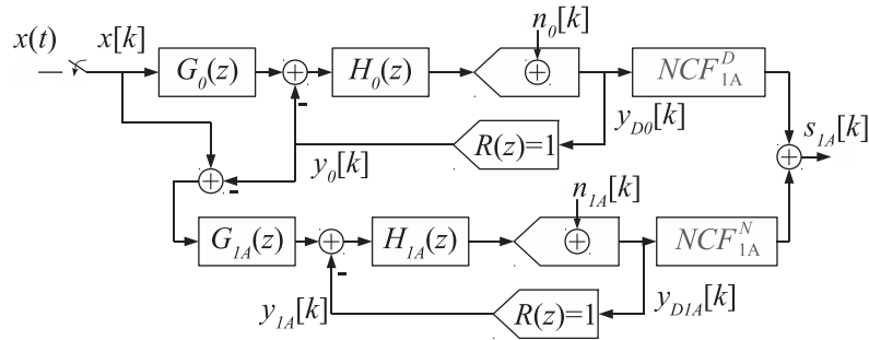
Figure III.18: The general DT MSNBC Architecture
