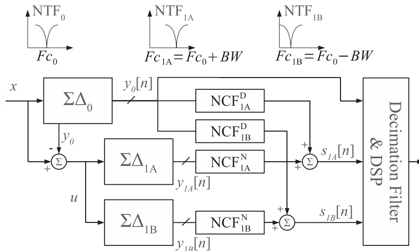
Figure III.17: The general MSNBC Architecture
