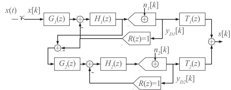
Figure II.11: DT MASH Architecture
