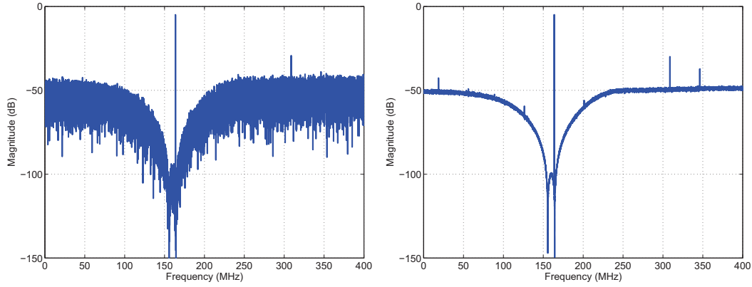
Figure III.26: One realization spectrum — High variance of the Noise PSD Figure III.27: Average spectrum over 100 realization — Low variance of the Noise PSD
