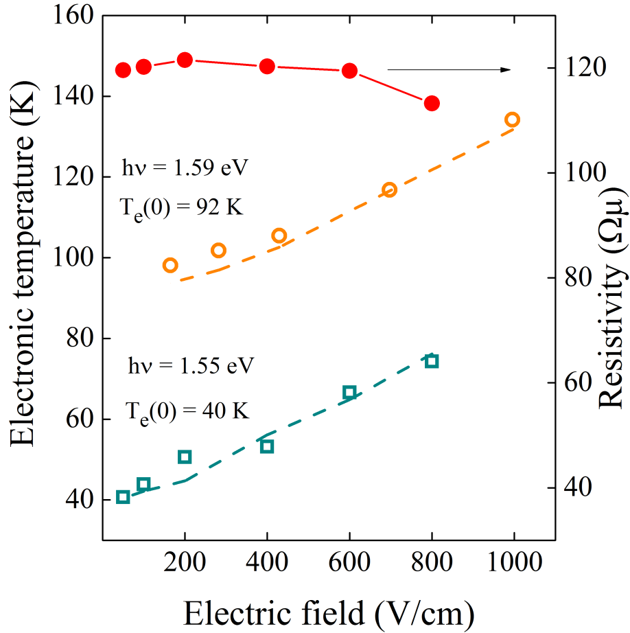
Figure 4.11: Measured T_e as a function of applied electric field for laser excitation energies of 1.55 eV and 1.59 eV, respectively. The increase of T_e as a function of E is well explained by Eq.(4.3) which assumes an energy-independent energy-relaxation time of 1.5 ps (dotted line) and 1.2 ps (solid line) for each case. Also shown (red dots) is the electric field dependence of the resistivity, which confirms that the hole temperature is only weakly affected by the electric field.
