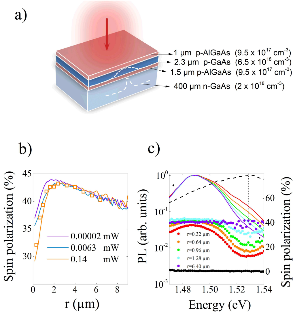
Figure 6.7: a) Schematic of a layered p + -GaAs sample grown on top of a n + -GaAs substrate. The dashed lines represent the photoelectron density at the steady state in the p + -GaAs and in the substrate, where the spin polarization is small. The volume density of impurities in both layers being comparable, luminescence coming from the p + -GaAs layer will be mixed with the one coming from the n + -GaAs Substrate. b) Measured spin polarization profiles at T_L = 15 K. It is seen that a dip near r = 0 exists independently of the degree of degeneracy of the photoexcited electrons, since it is visible at extremely low power excitation. The squares represent the energy-averaged spin polarization calculated from local spectra at P = 0.14 mW. c) Photoluminescence spectra and its energy-resolved spin polarization at P = 0.14 mW for selected values of r . It is observed that with respect to the spectrum far from the excitation spot ( r = 6.4 μm), as r approaches to r = 0 , an excedent of unpolarized luminescence at 1.53 eV is apparent, as can be confirmed with the measured energy-resolved spin polarization (closed circles). The energy of this excedent luminescence corresponds to the measured peak energy of the substrate's luminescence, shown by the dotted black curve, whose degree of circular polarization is near to zero, as shown by the closed black circles.
