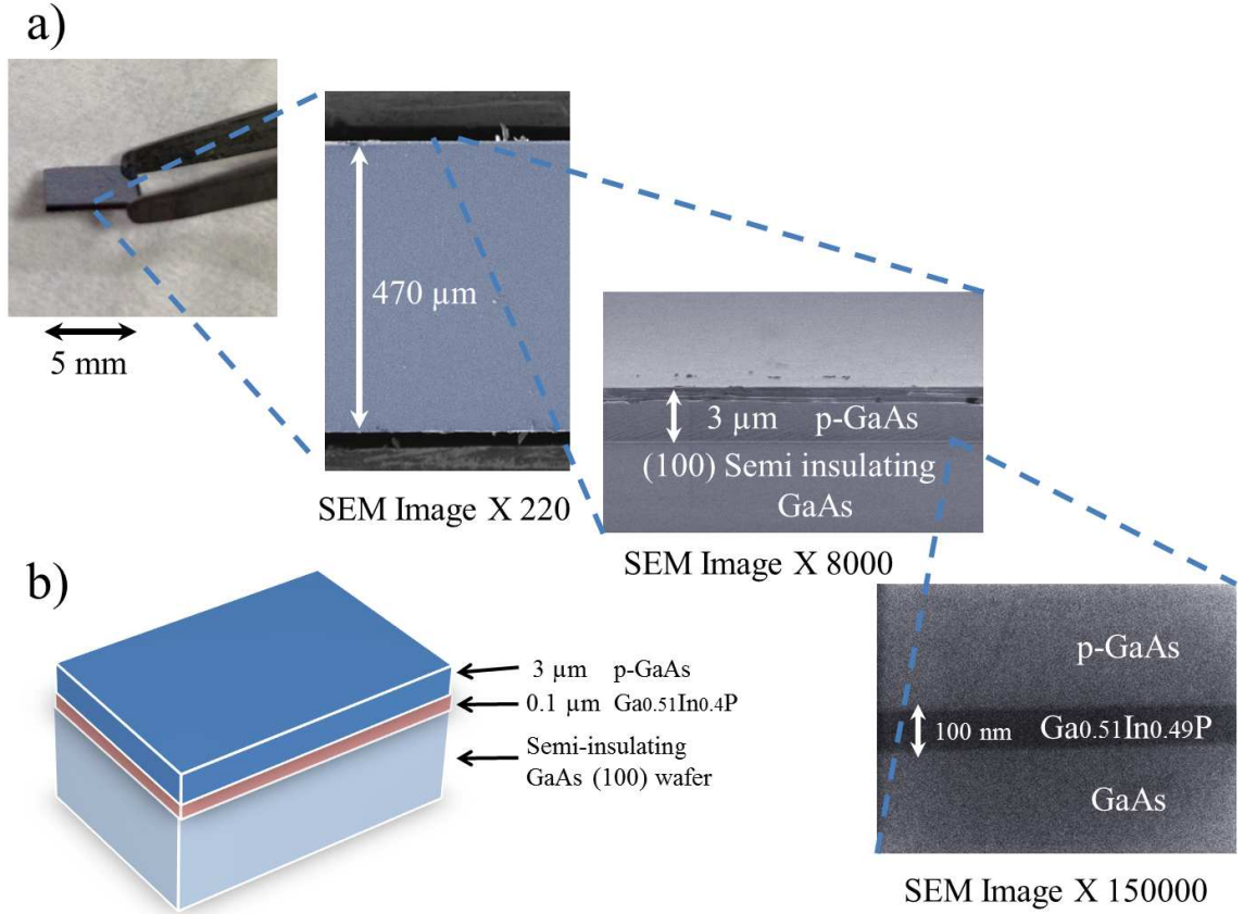
Figure 4.1: a) Optical (left) and SEM images of a p + -GaAs sample grown by molecular beam epitaxy over a semi-insulating GaAs wafer (470 μm). The thickness of the p-region is 3 μm, and a ~ 100 nm thick, Ga 0.51 In 0.49 P barrier was also grown between the substrate and the active layer in order to confine photoelectrons and to ensure a small surface recombination velocity at the back interface. b) Schematic of the layered structure of the sample.
