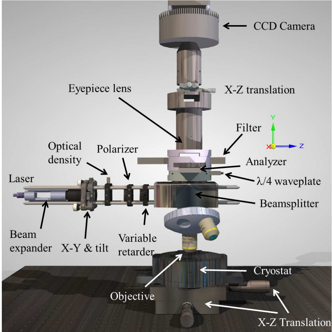
Figure 3.2: Schematic of the microscope used for imaging polarized luminescence. The excitation arm allows for a linearly or circularly-polarized laser beam to be focussed to a diffraction limited Gaussian spot of radius \omega = 0.6 \mu\text{m} by a x50 objective. The luminescence, which is analyzed into its \sigma^+ and \sigma^- -polarization components thanks to the rotation of a \lambda/4 waveplate followed by a fixed analyzer, is imaged with a CCD camera once the laser is properly filtered.
