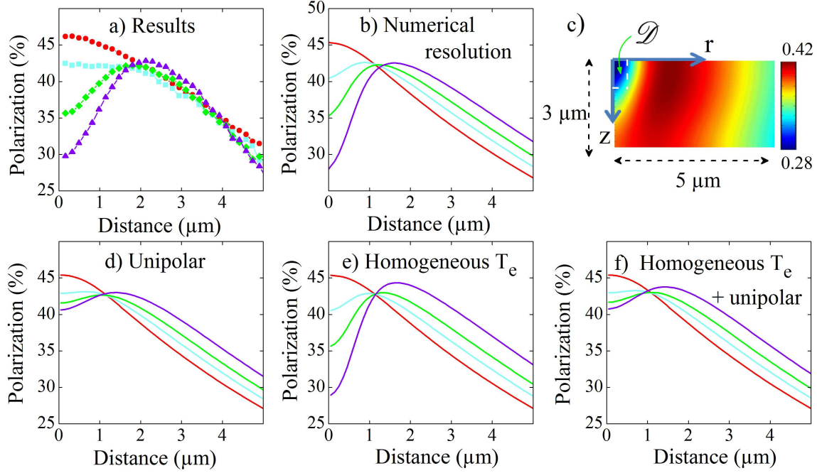
Figure 6.10: Panel a shows the experimental polarization profiles at T = 15 K as a function of excitation power : 28 \mu\text{W} (filled circles), 0.45 \text{ mW} (filled squares), 1.03 \text{ mW} (filled diamonds), 2.55 \text{ mW} (filled triangles). Panels b, d, e and f show with the same symbols, the corresponding calculated profiles. Panel b show calculated profiles including all effects which modify spin transport. Panel c shows the calculated spatial distribution of the polarization for an excitation power of 2.55 \text{ mW} . The profiles of Panel d were obtained in the simplest unipolar case. With respect to Panel b, the profiles of panel d do not consider ambipolar diffusion, those of Panel e do not consider thermoelectric currents, and those of Panel f neglect both ambipolar diffusion and temperature gradients and thus illustrate the conditions of spin-grating experiments.
