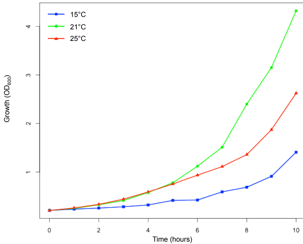
Additional Figure S1: Growth curves of YAAL on YPD at different temperatures. The growth curves at 15°C, 21°C and 25°C are represented in blue with squares, in green with dots, and in red with triangles, respectively.
