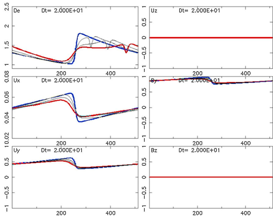
Figure 15. One-dimensional MHD simulation: long time evolution of plasma parameters from the initialization (blue curve, t=0 ) to the last time step (red curve, t=80 ) for the shock initialized alone in the box. Abscissa is the grid point number.
