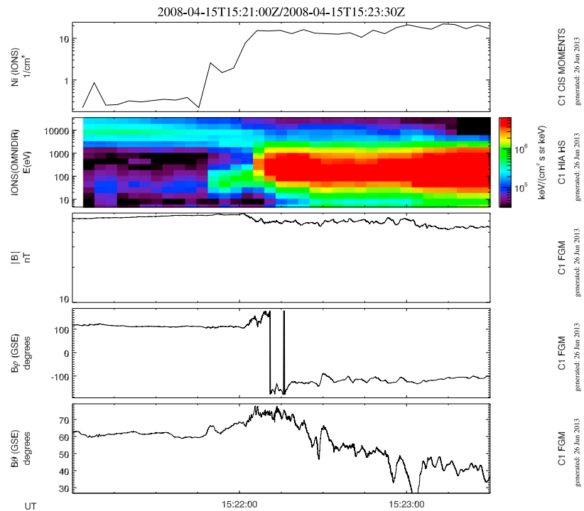
Figure 1. Density, energy spectrogram, and magnetic field (modulus and components \theta and \phi ) observed by Cluster C1 around 15:21 on 15 April 2008. The jump of density, change in plasma energy composition, and rotation of magnetic field show that the satellite is crossing the magnetopause.
