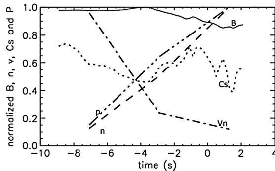
Figure 7. Normalized normal velocity, density, pressure, magnetic field modulus, and slow mode velocity as a function of time for the shock. The normalized quantities are normalized with respect to their maximum values.
