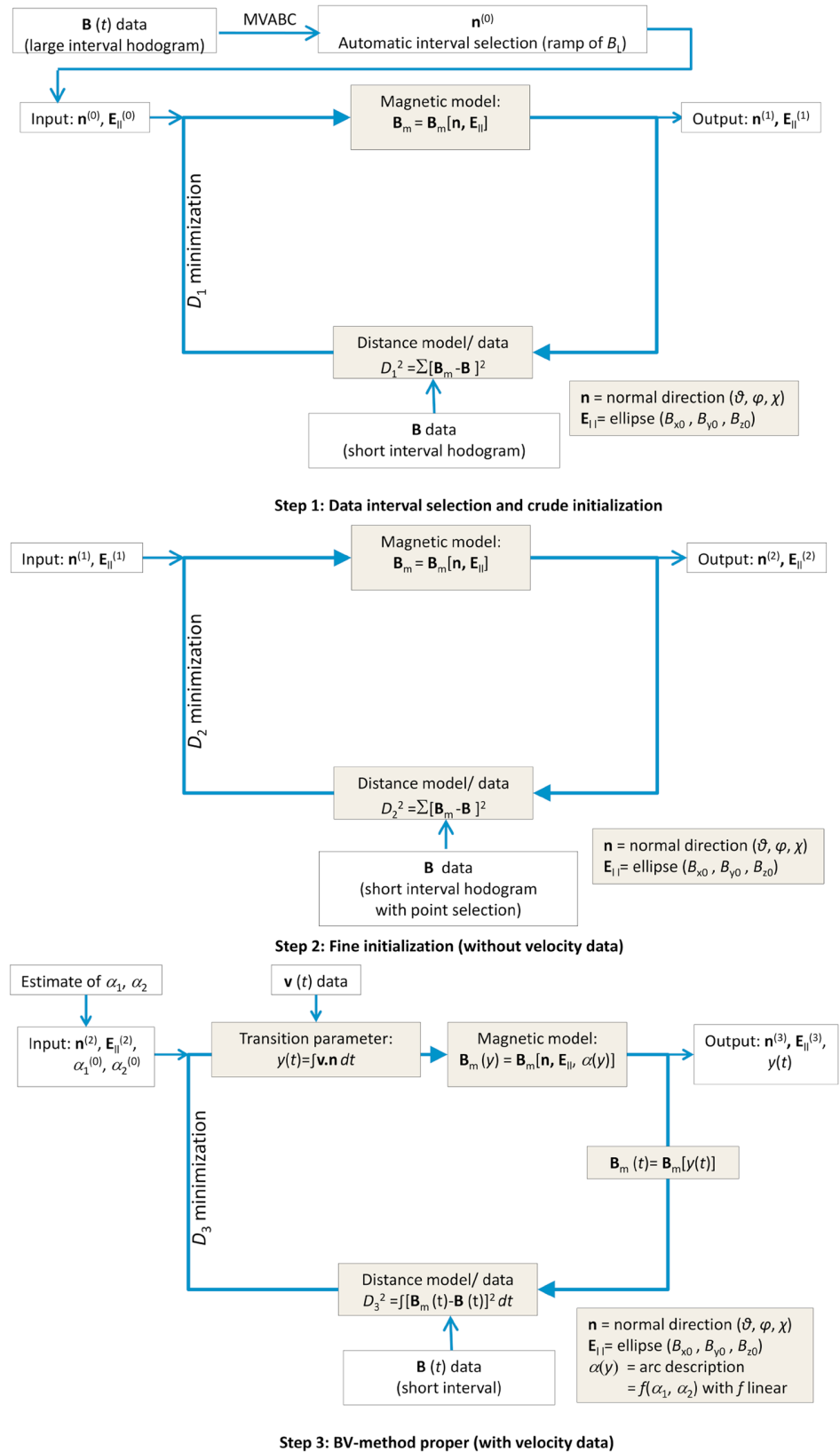
Figure 4. Algorithm used for initialization and BV method. \mathbf{E}_{\parallel} stands for the elliptical form that is determined at each step (characterized by B_{x0}, B_{y0}, and B_{z0} ).
