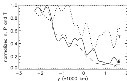
Figure 11. Evolution with normal position of normalized density (to 2.5 \text{ cm}^{-3} ), pressure (to 0.17 nPa), and temperature (to 6 MK) measured by Cluster C3 Cluster Ion Spectrometry instrument for the 3 March 2008 crossing.
