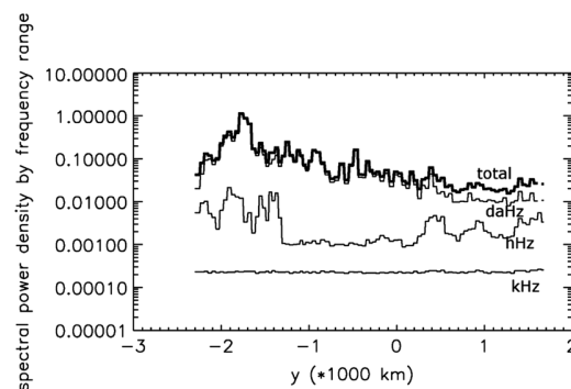
Figure 13. Evolution with normal position of the spectral power density (in nT^2 ) for magnetic field measured by Cluster C3 STAFF instrument. The total spectral power density is the thick line, as the daHz, hHz, and kHz frequency ranges are also represented on the same scale.
