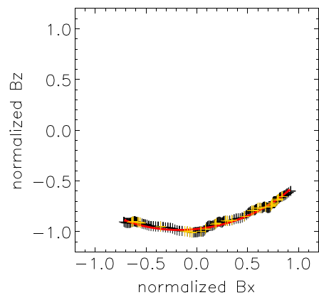
Figure 6. Fit of the hodogram of the magnetic field in the simulation for a virtual satellite crossing far from X point in the numerical simulation. The data are in black, the selected points in yellow, and the fit in red.
