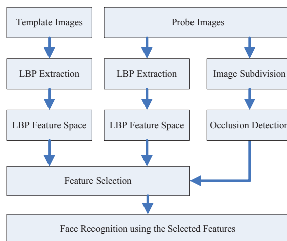
Illustration of the proposed face recognition system.
