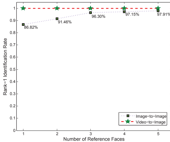
Figure 6.9: Rank-1 identification rates of the “Image-to-Image” approach and the “Video-to-Image” approach based on 1-5 canonical faces ( M=1:5 ) for registration.
