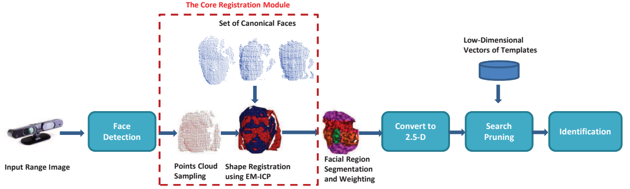
Figure 6.6: System overview.
