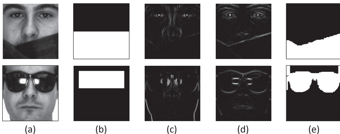
Illustration of the proposed occlusion segmentation: (a) examples of faces occluded by scarf and sunglasses; (b) initial guess of the observation set according to the results from occlusion detection; (c)(d) are the visualization of horizontal and vertical structural prior; (e) the generated occlusion masks.
