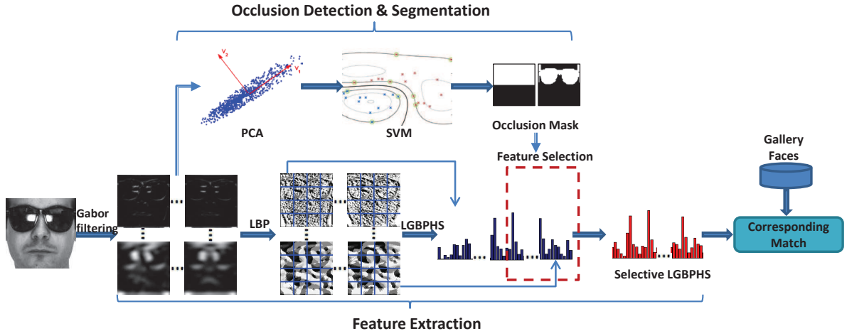
Figure 3.13: Illustration of the proposed selective-LGBPHS approach for face recognition in occluded conditions.
