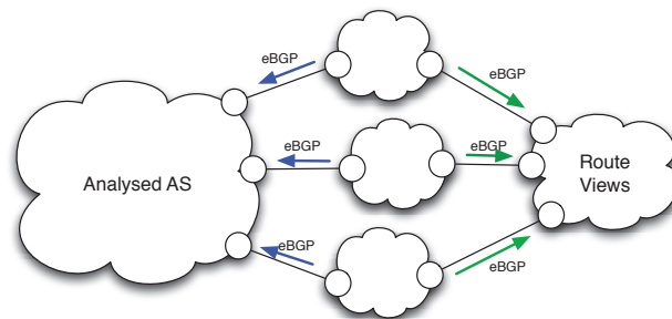
Figure 2.4: Route Views connectivity
