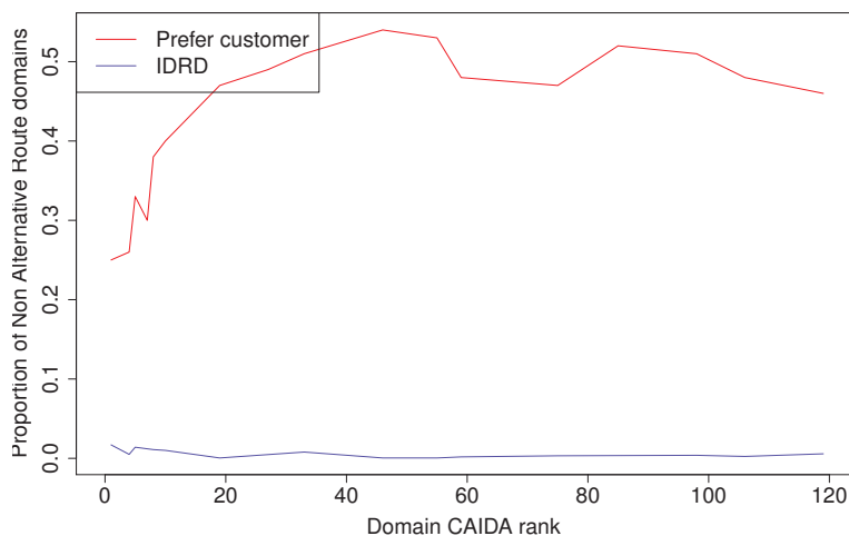
Figure 3.13: Proportion of “no disjoint path” destination ASes.
