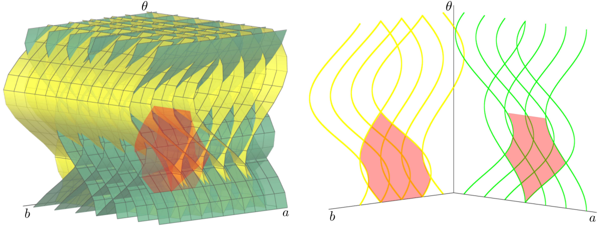
Figure 5.1: Left: the authorised transformations (in red) induced by partial constraints using larger regions of size [-\frac{3}{2}, \frac{3}{2}]^2 , and expressed via “offset” surfaces. Right: their projections to the planes (a, \theta) and (b, \theta) with the associated “offset” curves.
