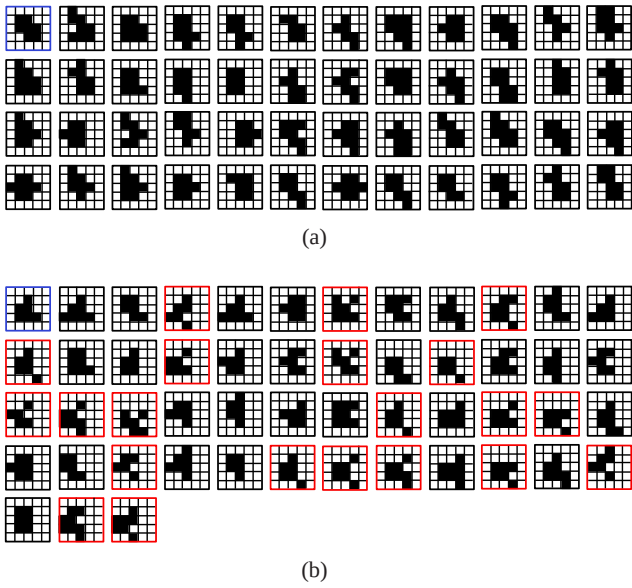
Fig. 15 (a) A topologically invariant 5 \times 5 image (in blue frame), and (some of) its transformations (in black frames). (b) A topologically-variant 5 \times 5 image (in blue frame), and (some of) its simple-equivalent (in black frames) and non-simple-equivalent transformations (in red frames).
