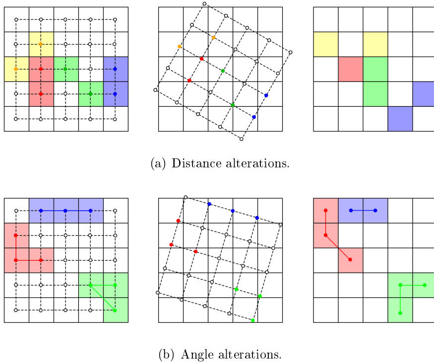
Figure 2.6: Digital rigid transformations do not preserve distances (a) and angles (b). Left column ( \mathbb{S} ): original image with the associated grid. Middle ( \mathcal{T}(\mathbb{S}) ): rigid transformation of the grid defined in the left column, where \mathbb{S} is the support of the image. Right ( T(\mathbb{S}) = D \circ \mathcal{T}(\mathbb{S}) ): result of the induced digital rigid transformation. (a) Two points in red (resp. blue, green and yellow) are considered for distance alterations changing from 1 (resp. 1, \sqrt{2} and \sqrt{2} ) to 0 (resp. \sqrt{2} , 1 and 2). (b) Three points in red (resp. blue and green) are considered for angle alterations changing from \frac{\pi}{2} (resp. \pi and \frac{\pi}{4} ) to \frac{3\pi}{4} (resp. 0 and \frac{\pi}{2} ).
