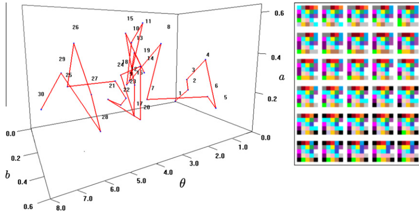
Fig. 17. A discrete transition path of the DRT graph in the parameter space (a, b, \theta) (left) and a sequence of transformed images (right). Each vertex of the path represents a DRT which gives a digital transformed image. The first image corresponds to the identity transformation and the images from left to right and from top to bottom correspond to the vertices ordered in the path.
