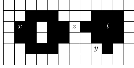
Fig. 3 Examples of simple (\mathbf{x}, \mathbf{y}) and non-simple (\mathbf{z}, \mathbf{t}) points in a binary image. Modifying the value of \mathbf{z} would merge two black connected components, while modifying the value of \mathbf{t} would create a white connected component. In both cases, the homotopy-type of the image would be modified.
