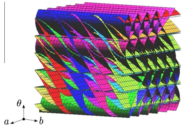
Fig. 4. Discrete rigid transformations (DRTs) are observed as regions separated by tipping surfaces.
