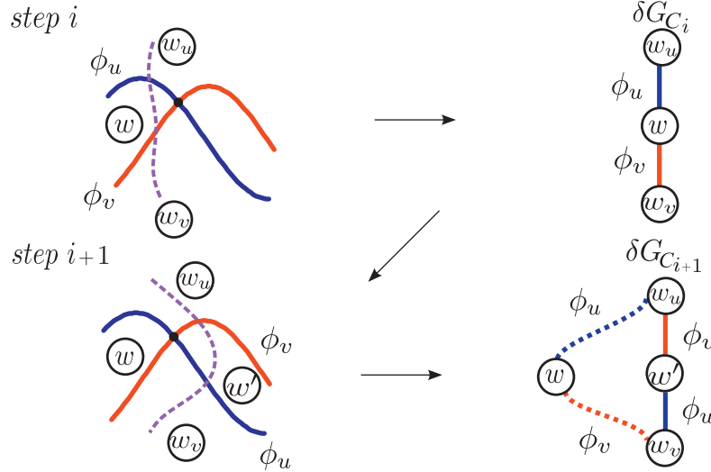
Fig. 11. Illustration of a progress of a cut by which the partial graph \delta G_{i+1}^C is modified from \delta G_i^C in simple case.
