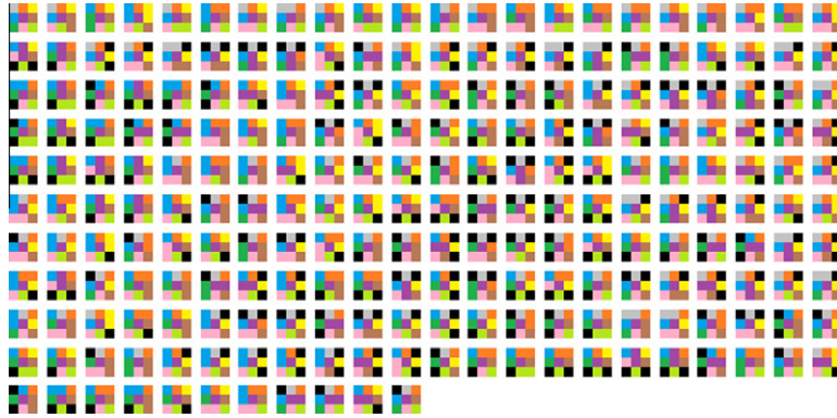
Fig. 16. The 231 images are generated by using the Eulerian model from the part of a DRT graph for a given image of size 3 \times 3 where a, b \in [\frac{1}{2}, \frac{3}{2}] and \theta \in [0, \frac{\pi}{4}] . The first image is the identity transformation. In the transformed images, we do not show pixels that are pushed out of the image support. Also, formerly background pixels are “filled” with a black colour.
