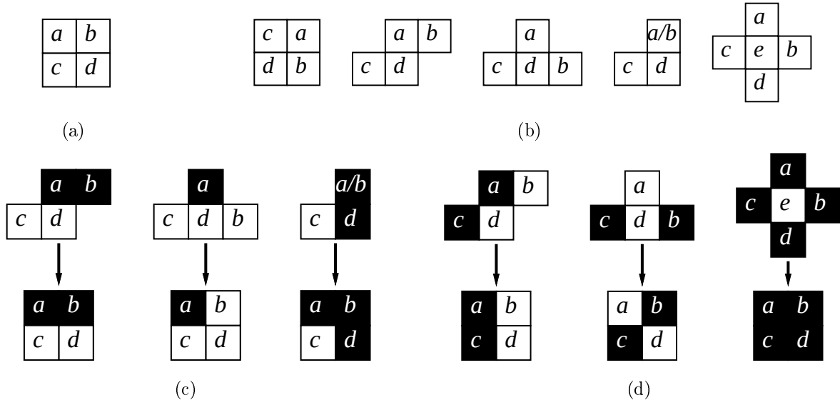
Figure 4.7: (a) A 2 \times 2 pixel sample with values a, b, c, d . (b) All the local pixel configurations (up to rotations and symmetries) leading to the sample in (a) when applying digital rigid transformations. (c) Examples of transformations in which the samples preserve the topology of local pixel configurations. (d) Examples of transformations in which the samples are topologically altered.
