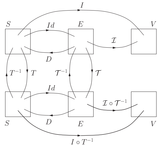
Fig. 1. Geometric transformation and the associated digital image transformation (see text). First row: image support before transformation. Second row: image support after transformation.
