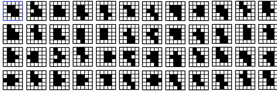
(a) Topologically invariant image.
