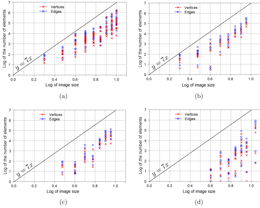
Fig. 18 Experimental results of space complexities of FDRT graphs for two (a), three (b), five (c) and ten (d) pixel-invariance constraints.
