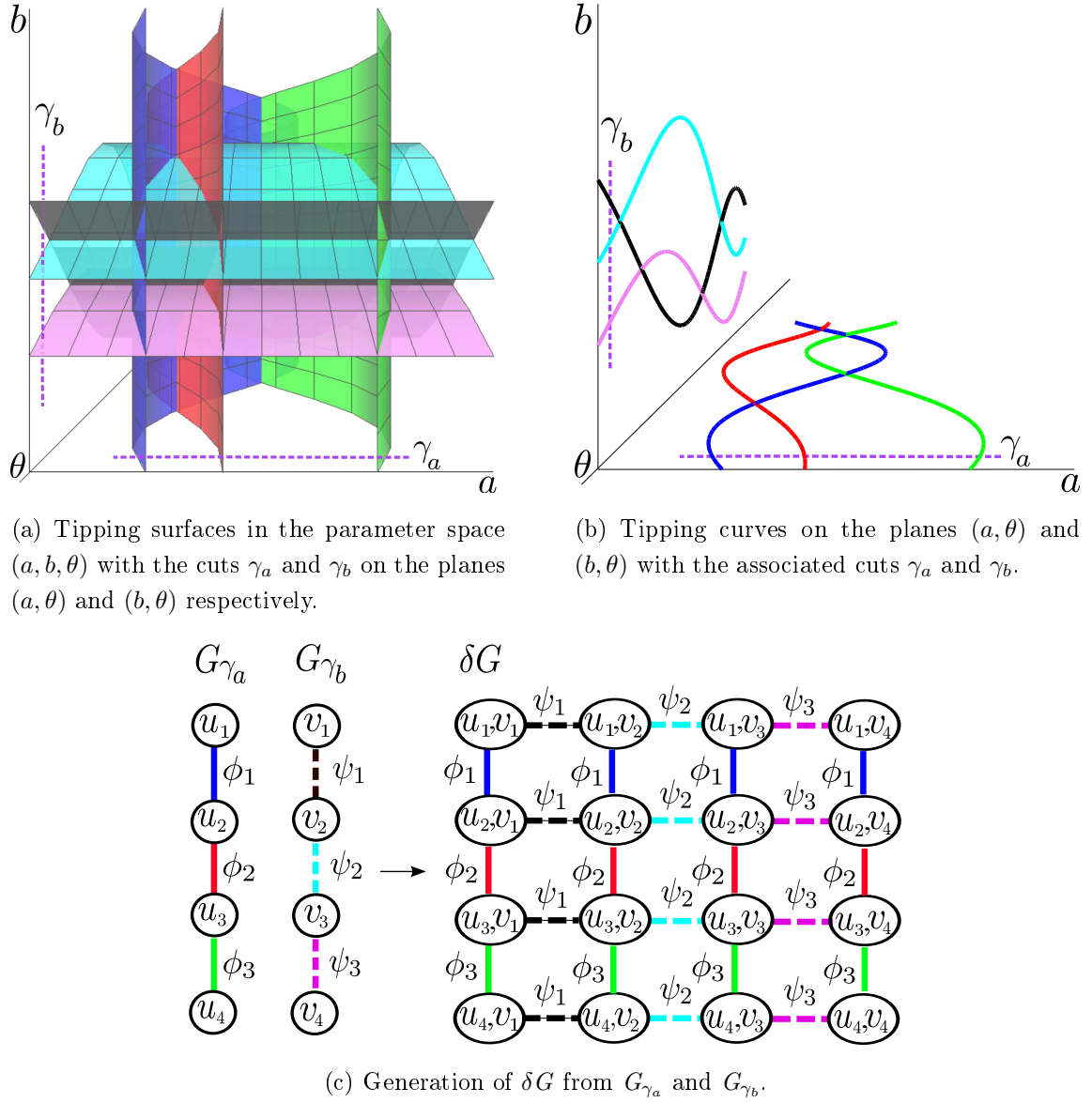
Figure 3.8: Generation of a partial graph \delta G from two graphs G_{\gamma_a} and G_{\gamma_b} associated to cuts \gamma_a and \gamma_b respectively.
