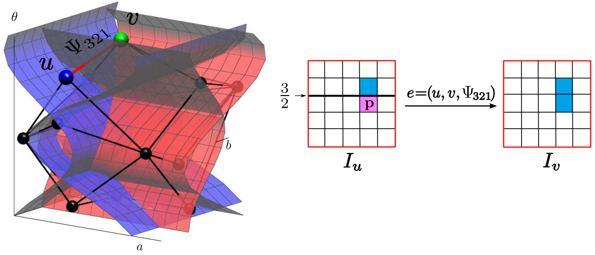
Figure 3.2: Left: subdivision of the parameter space of rigid transformations by tipping surfaces, and the associated DRT graph. Let us focus on the edge e = (u, v, f) (in red) which connects two vertices u and v (in blue and green, respectively), and has the tipping surface \Psi_{321} as label. Right: two digital images I_u and I_v associated to the vertices u and v , respectively. The tipping surface \Psi_{321} encoded on e indicates that the pixel (in rose) \mathbf{p} = (3, 2) will get its value from the one (in blue) after the half-grid line y = 1 + \frac{1}{2} , according to the Eulerian model. Thus, two vertices u and v separated by \Psi_{321} have their associated transformed images I_u and I_v differing only at \mathbf{p} .
