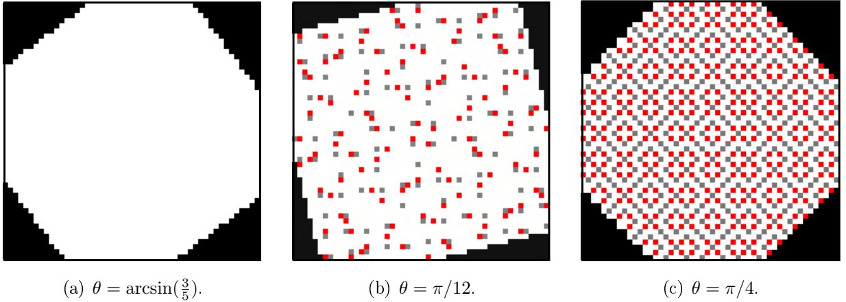
Figure 2.5: Some digital rotations by angles \theta of a white square of size 100 \times 100 . Double pixels are depicted in red, and null pixels in grey.
