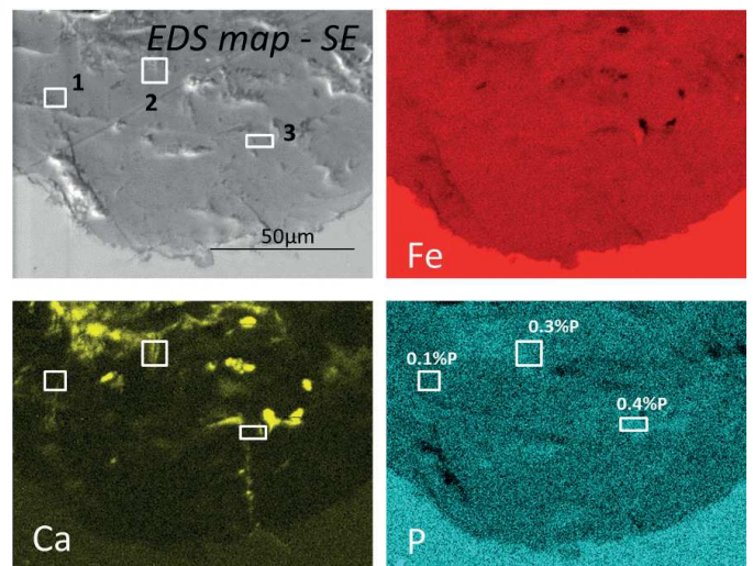
Figure 5: EDS map "B-map1" (15 kV) acquired on sample B. [1]-[2]: zones quantified in table 2. [a]-[d]: \mu\text{RS} spot analyses.
