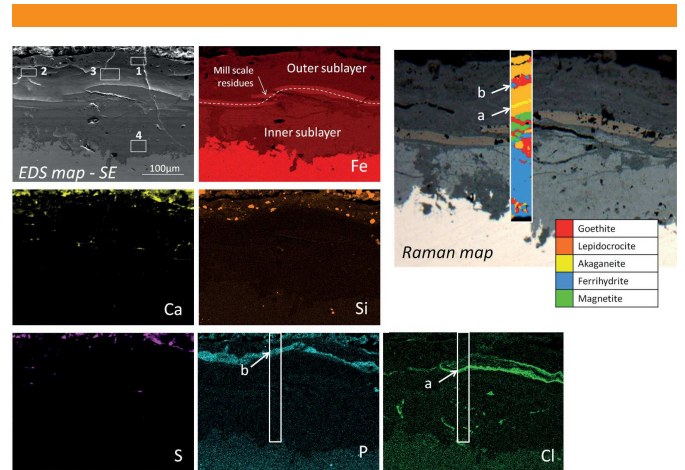
Figure 4: EDS map "A-map1" (15 kV) and \mu\text{RS} map acquired on sample A. [1]-[4]: zones quantified in Table 2. [a]: zone rich in chloride/akaganeite; [b]: zone rich in phosphorus/ferrihydrite.
