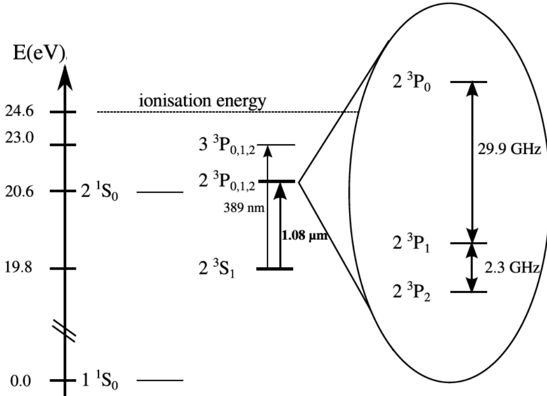
Figure 2.1: Helium 4 atomic structure. Energy level representation of the first excited states of helium atom. The metastable state 2\ ^3S_1 is represented 19.8 eV above the fundamental level and the optical transitions with the excited state 2\ ^3P_{0,1,2} used for cooling and manipulate the metastable state are represented.
