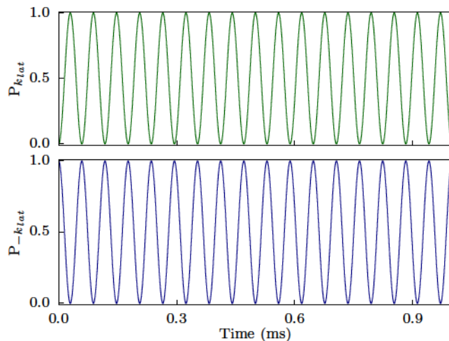
Figure 4.3: Example of a Rabi oscillation. Rabi oscillation of the population between the quasi-momenta +k_{lat} and -k_{lat} for a lattice depth of V_0 = 0.8E_{lat} . The initial quasi-momentum q_0 is equal to -1k_{lat} such that the probability to diffract to q_0 + 2k_{lat} = k_{lat} is maximum.
