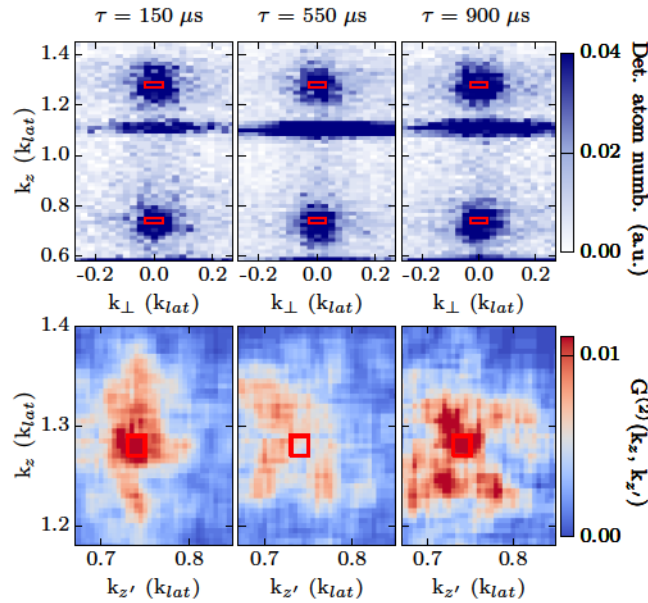
Figure 5.11: 2D determination of the optimised centred analysis \{k_a, k_b\} . Upper panels, from left to right, 2D momenta distribution for the detected atom number on the yz -plane, integrated over a length of 0.048 k_{lat} along the x -axis, for \tau = 150, 550, 900 \mu\text{s} . Bottom panels, from left to right: 2D cross-correlation between momentum k_z, k_z' for an integration volume of \Omega_V = [0.048^2 \times 0.028] (k_{lat}^3) for \tau = 150, 550, 900 \mu\text{s} . The red shaded square correspond to the integration length on the longitudinal z -axis. The bin size is of 0.014 k_{lat} on both axis.
