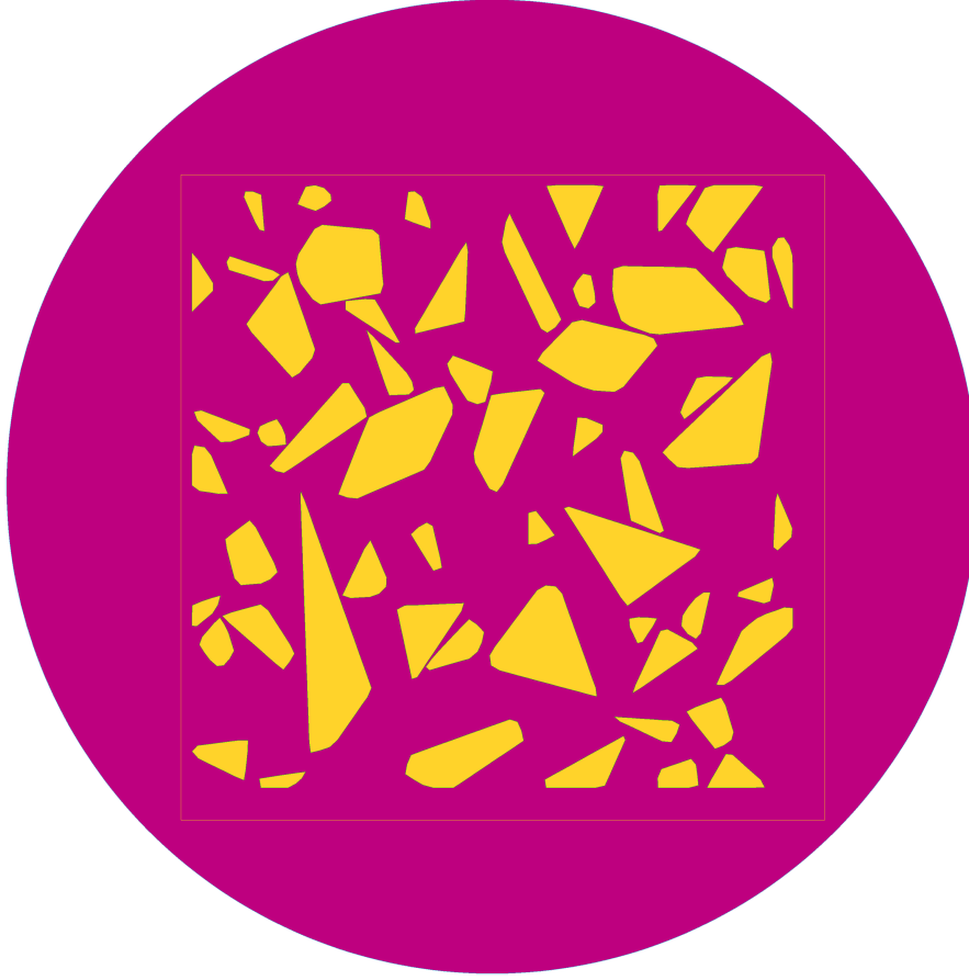
Figure 5.7: The index of refraction used for the simulation
