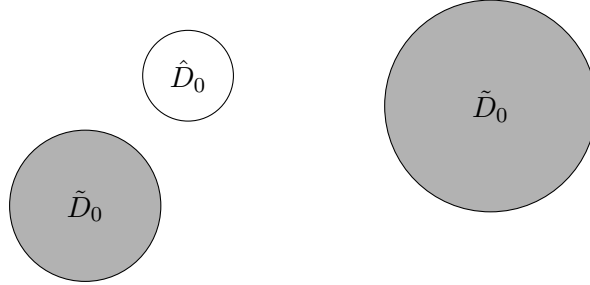
Figure 3.1: Sketch of a possible configuration for D_0 (the part \tilde{D}_0 is shaded).
