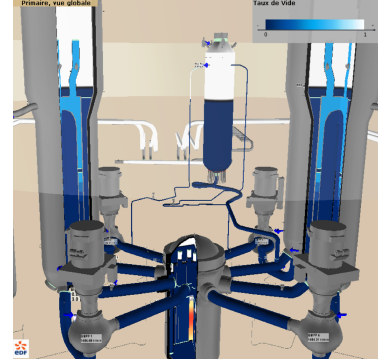
FIGURE 2. 3D view of a PWR primary coolant. The core vessel in the center is about four meter high by four meter wide. Pressurized water circulates at about 17 m/s, at 155 bar pressure and 300^{\circ}\text{C} temperature.
