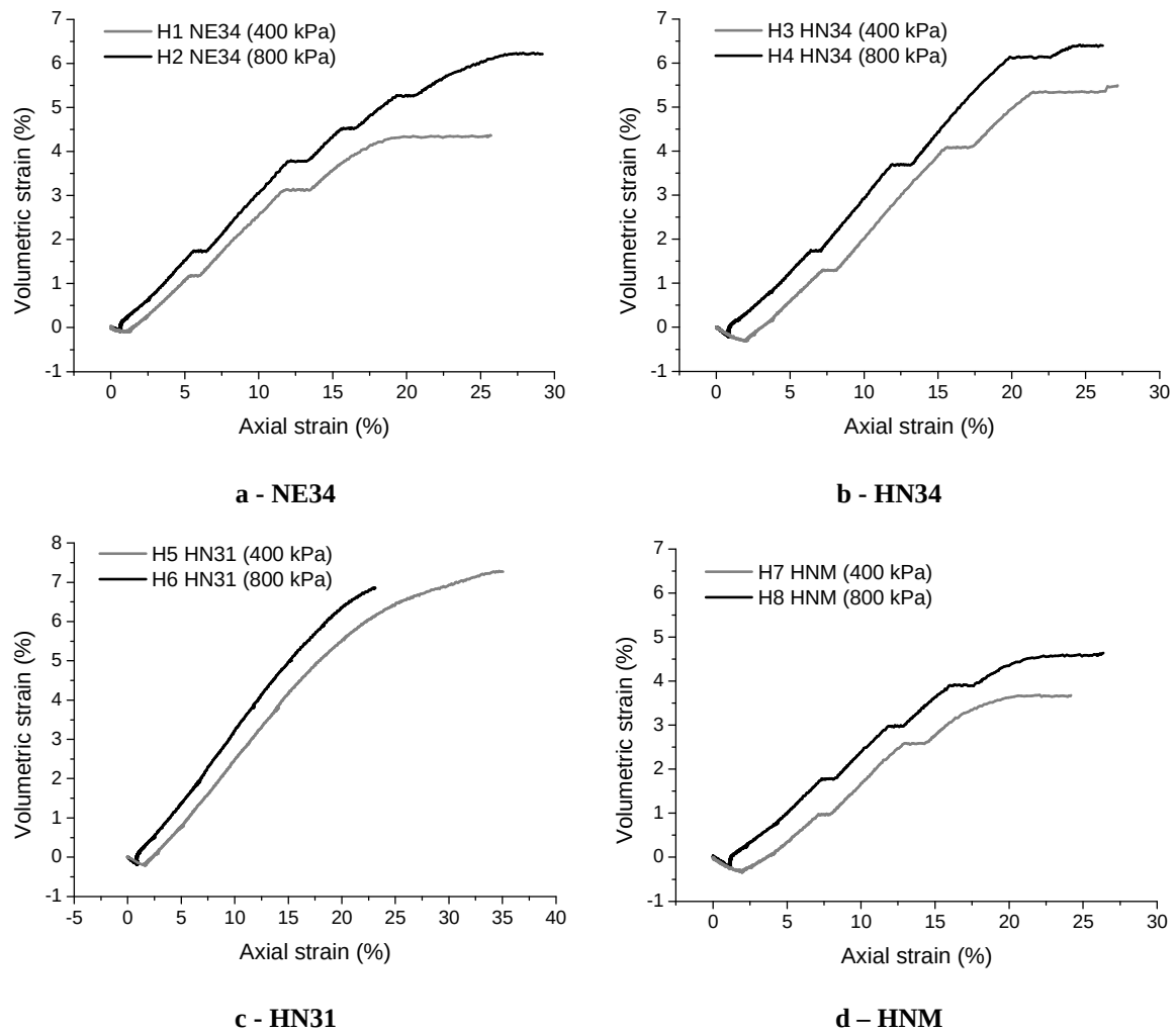
Figure 11- Volumetric strain – axial strain curves for all specimens subjected to a horizontal path for two confinement pressures of 400 kPa and 800 kPa
