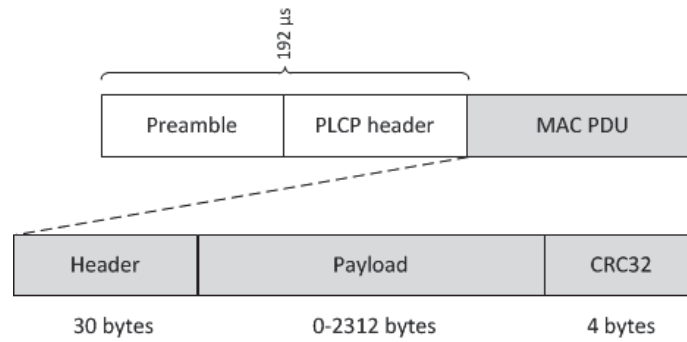
Figure 5.6: Composition of a 802.11 Wi-Fi frame taken from [279].
