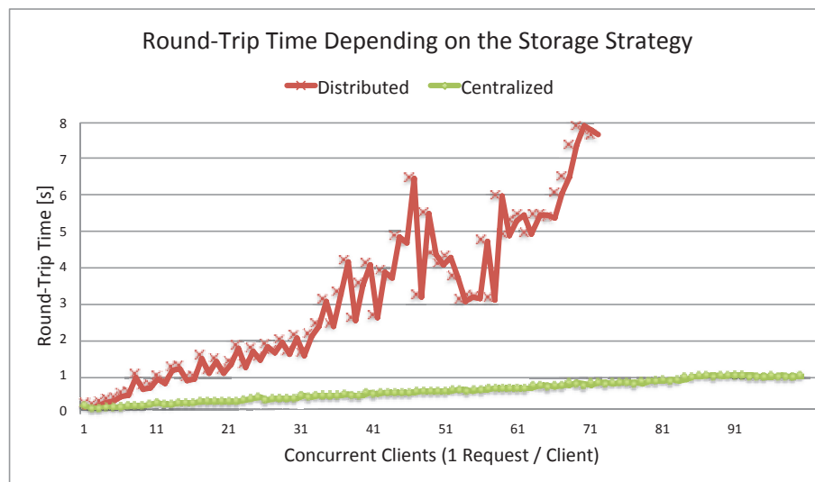
Figure 4.32: Round-trip time for up to 100 concurrent clients sending GET requests for retrieving historical data directly on a centralised sink or with the cloud-like storage.
