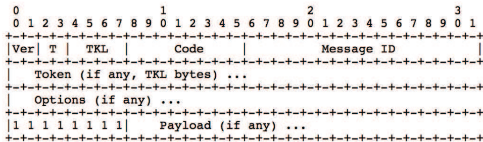
Figure 3.6: A CoAP message can be in the best case only four bytes long, as represented in [155].
