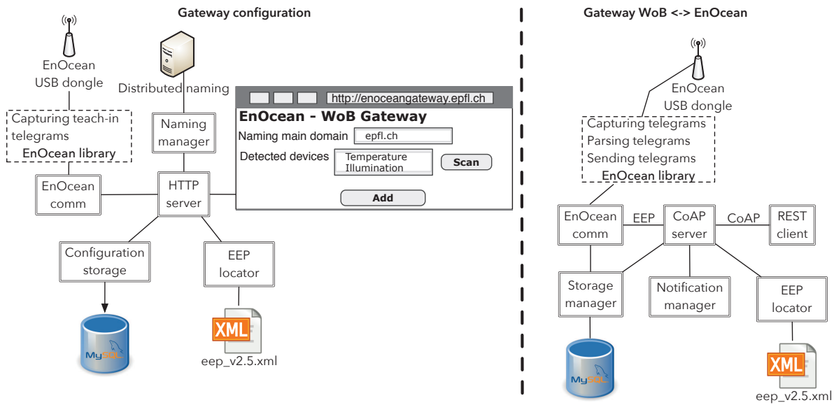
Figure 5.4: Overall EnOcean-WoB gateway architecture illustrating the logical modules for two scenarios: gateway configuration (left part) and gateway normal operation (right part).
