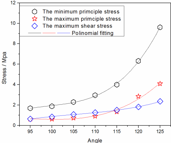
Fig. 6:8 The maximum local stress under the influence of inclined angle
