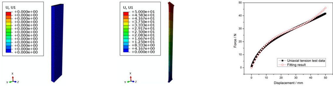
(a) Uniaxial tension test
