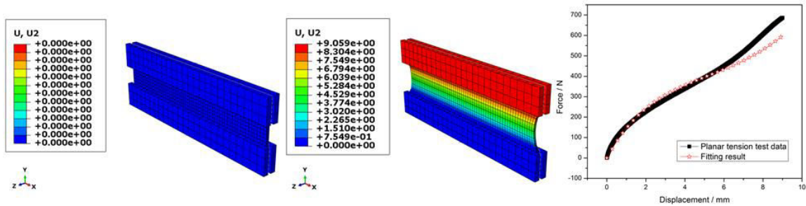
(c) Planar tension test
