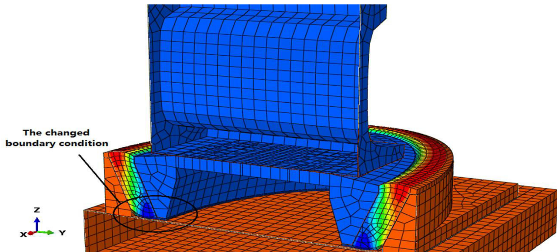
(b) The changed boundary condition
