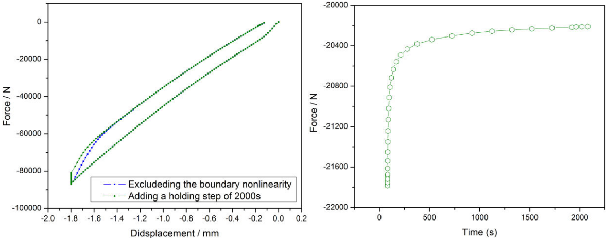
(a) With and without the holding step (b) Time-force relationship during the holding step
