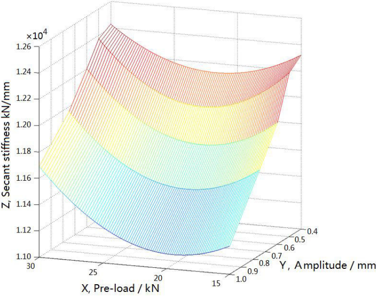
Fig. 2:17 Preload-and-amplitude dependent properties
