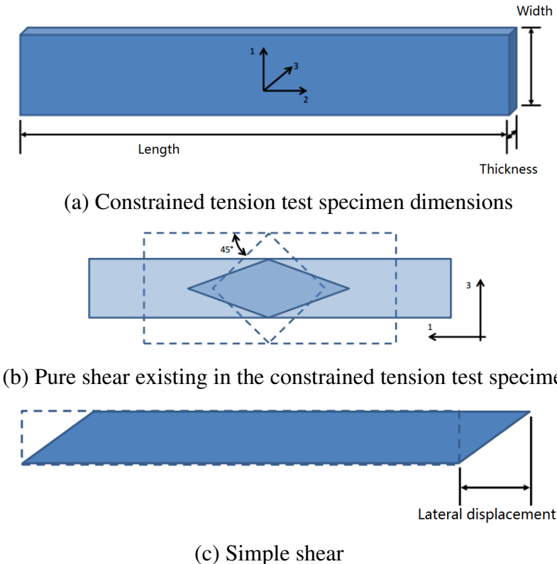
Fig. 4:4 Planar tension test equals to pure shear test by uniaxial constrained tension [166]
