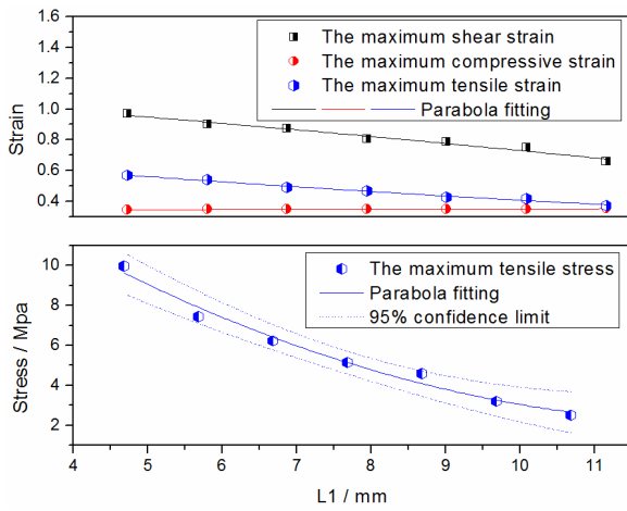
(a) Loaded vertically
