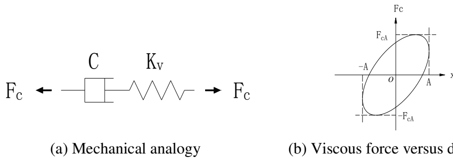
Fig.3:11 Mechanical analogy of linear viscous damper and the calculated hysteresis loop
