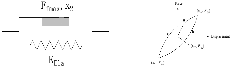
(a) Mechanical analogy of smooth friction model (b) Hysteresis loop of various amplitudes
