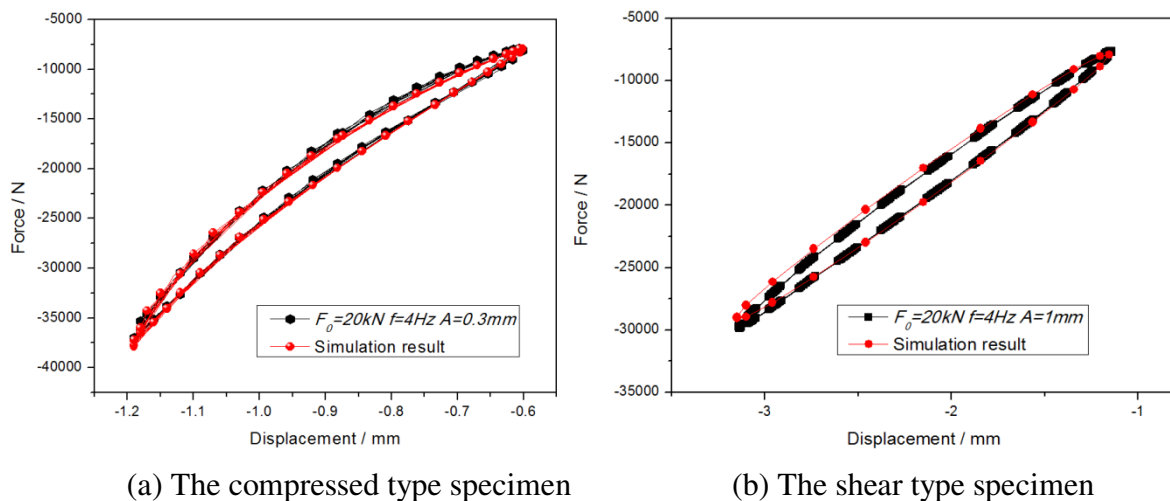
Fig. 5:27 Calculated hysteresis loops compared with the measurement
