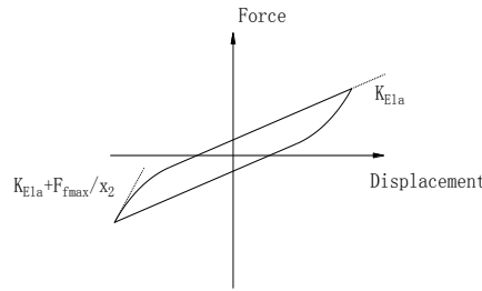
(c) Typical displacement-force curve with large amplitude displacement
