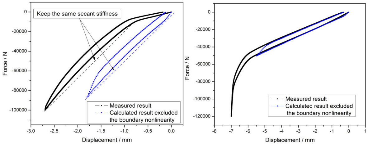
(a) The compressed type specimen (b) The shear type specimen Fig. 5:11 Calculated results when boundary nonlinearities are excluded
