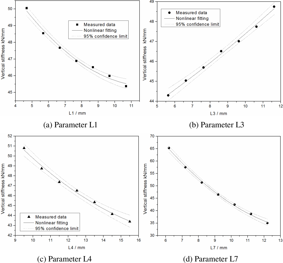
Fig. 6:14 Parameter influenced vertical stiffness of the compressed type fastening system
