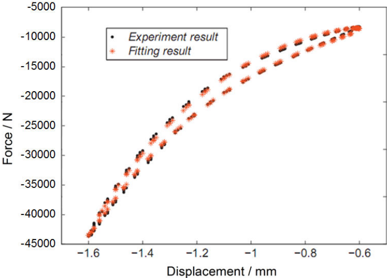
Fig. 3:2 Measured and calculated hysteresis loop of the compressed type fastening system when f=6 Hz and A=0.5mm
