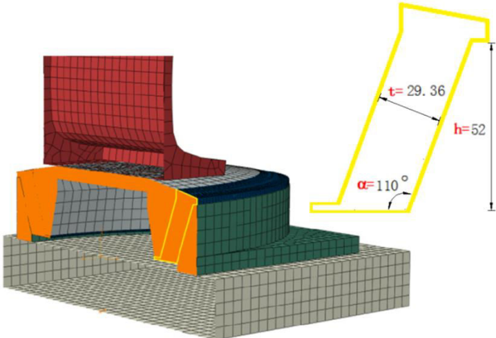
(a) The shear type fastening system
