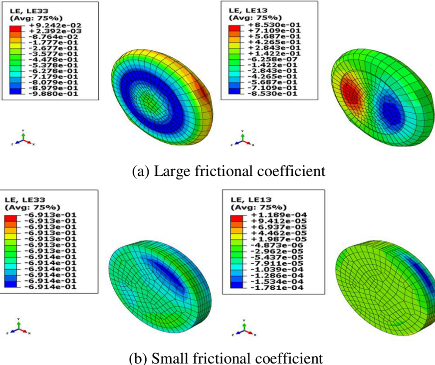
Fig. 5:13 Influences of boundary constraint on the shear and compression strain
