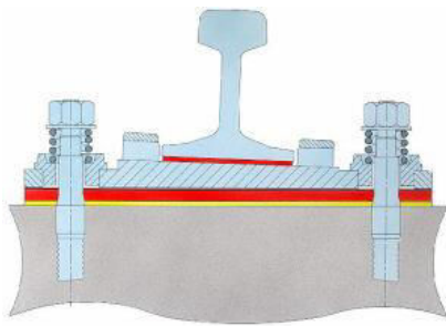
(a) Fastening system with resilient pads from Tiflex of UK (rail pad and baseplate pad)
