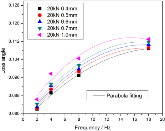
(c) Frequency dependent loss angle
