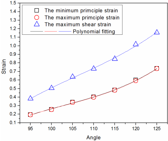
Fig. 6:7 The maximum local strain under the influence of inclined angle
