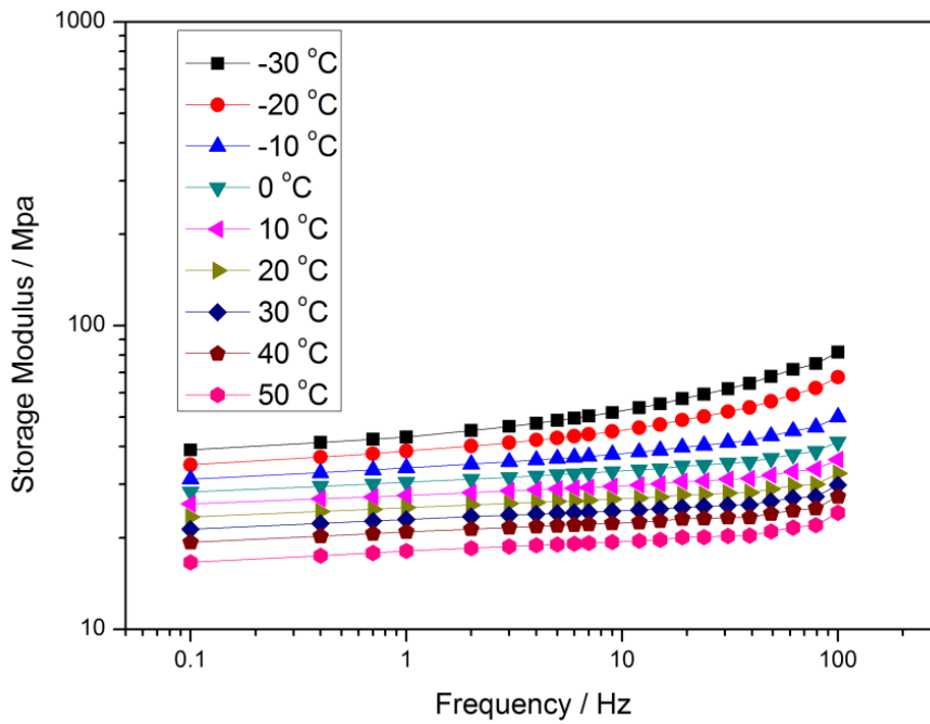
(a) Frequency-dependent storage modulus
