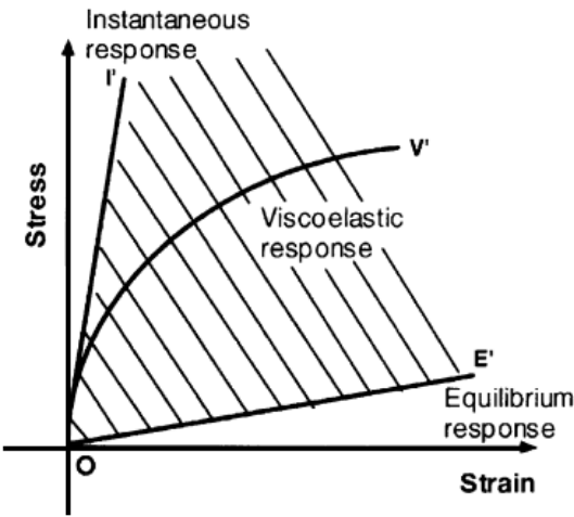
Fig. 5:26 Typical responses of a viscoelastic solid
