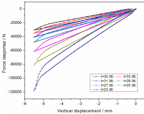
(a) Quasi-static loops
