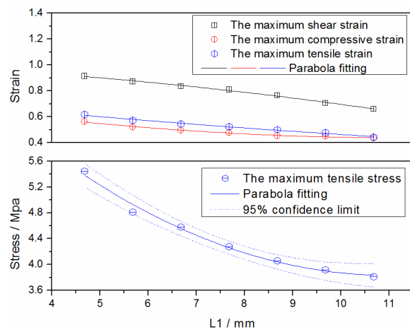
(b) Loaded laterally
