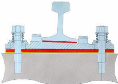
(a) Fastening system with resilient pads from Tiflex of UK (rail pad and baseplate pad)
