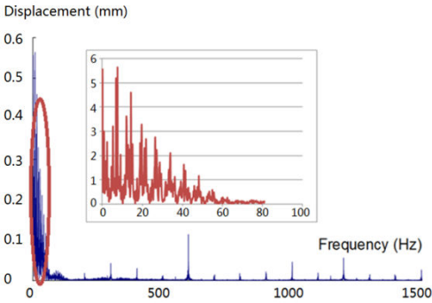
(c) Testing results
