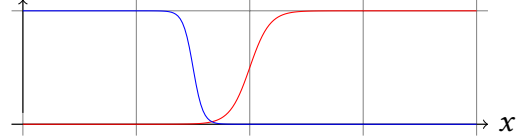
Figure 2.6.20: Graph of l_{xh}_{[1,3]} and h_{xl}_{[1,2]}
