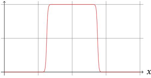
Figure 2.6.19: Graph of lil_{[1,3]}
