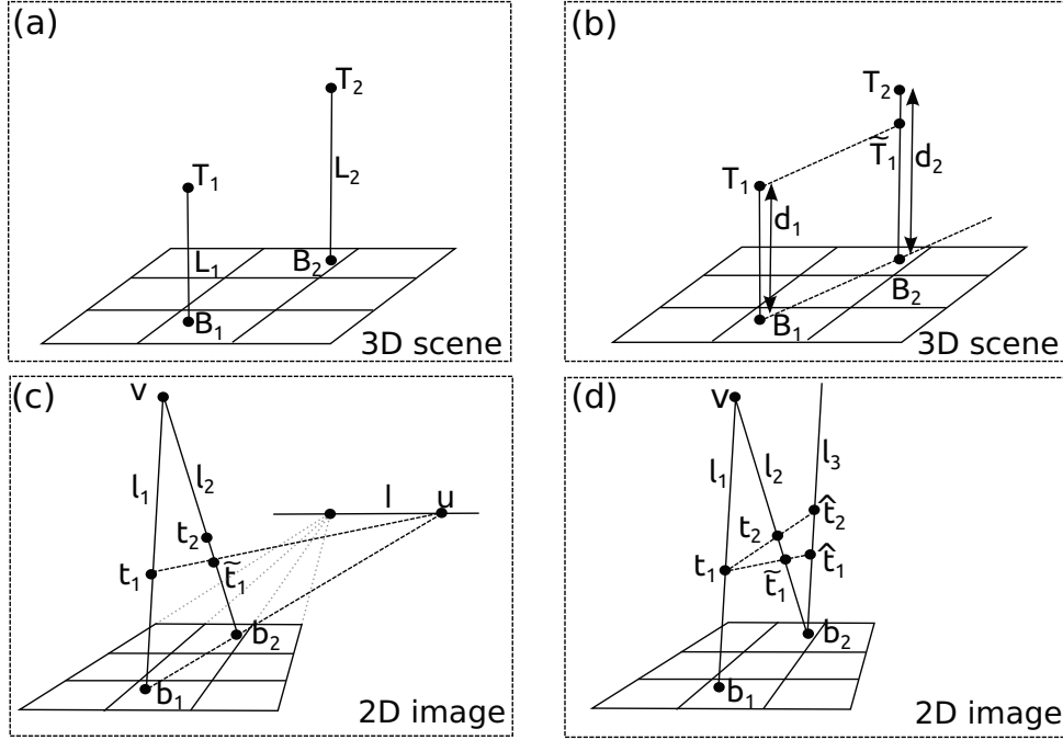
Figure 3.6: The image shows an illustration of how to compute length ratios of parallel scene lines. (a) Vertical lines segments L_1 and L_2 have length d_1 and d_2 respectively, their base points ( B_1 and B_2 ) are on the ground plane. Thanks to the information within the scene we can compute the length ratio d_1 : d_2 . (b) In the scene: L_1 segment's length may be transferred to L_2 by constructing a line parallel to the ground plane that generates the point \tilde{T}_1 . (c) l is the ground plane vanishing line, and v the vertical vanishing point, and u is the horizontal vanishing point. Thanks to this information we can establish the correspondences of points in one segment onto the other one ( \tilde{t}_1 ). (d) The line l_3 is parallel to l_1 in the image. After construction of the points \hat{t}_1 and \hat{t}_2 we obtain the distance ratio d(b_2, \hat{t}_1) : d(b_2, \hat{t}_2) (that is the computed estimate of the ratio d_1 : d_2 ).
