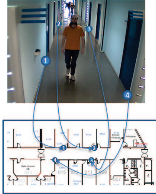
Figure 5.2: The image shows an example of point correspondences needed to compute the homography mapping which allows the transformation from the image space to the map plane. It is important to choose features that are shared between the two modalities.
