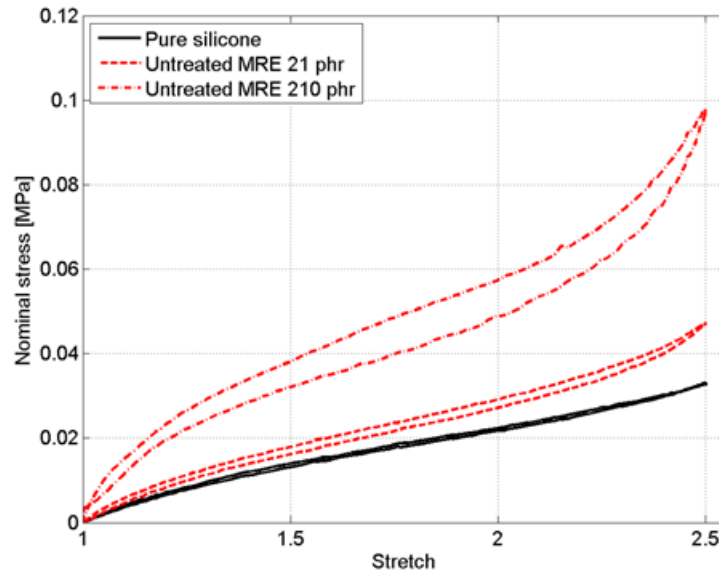
Figure 2.15: Stabilized hysteretic loop (shifted back to the origin) for pure silicone, 21 phr and 210 phr MRE samples.
