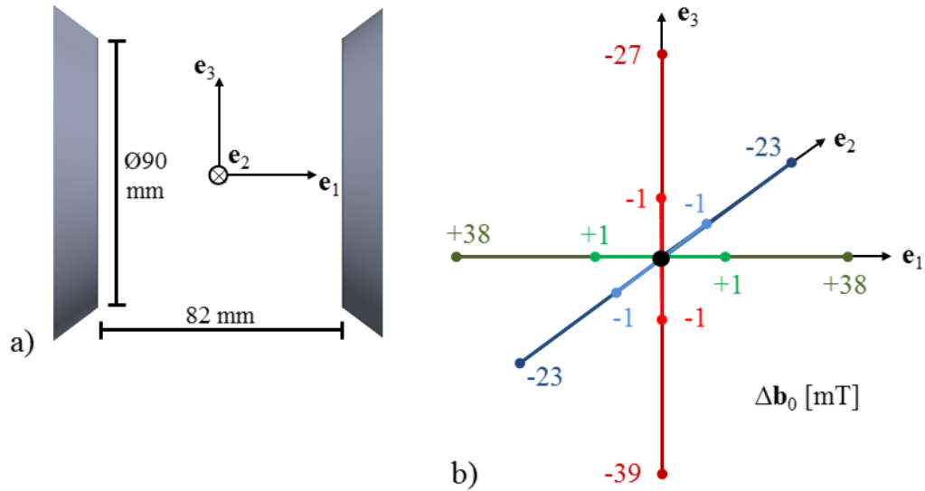
Figure 3.5: a) Sketch of the main axes centered within the poles of the magnet. b) Difference \Delta \mathbf{b}_0 [mT] from central field \mathbf{b}_0 = \mu_0 \mathbf{h}_0 = 0.8 T at 68 A on the main axes at the decisive points within the air gap: central zone ( \pm 3 mm , light colored lines), long axis of the samples in curing positions ( \pm 25 mm , dark green and dark blue line), long axis of the sample in testing direction ( \pm 25 mm , dark red line).
