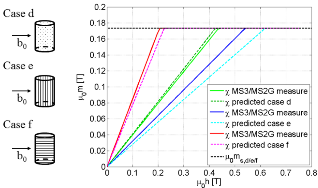
Figure 3.29: Predicted initial volume susceptibility \chi [−] SI for the isotropic 70 phr MRE (case d), the transversely isotropic 70 phr MRE with chains along direction e_3 (i.e. along the sample's axis and transverse to the applied magnetic field, case e) and the transversely isotropic 70 phr MRE with chains along direction e_1 (i.e. transverse to the sample's axis and along the applied magnetic field, case f) compared to the corresponding measurements.
