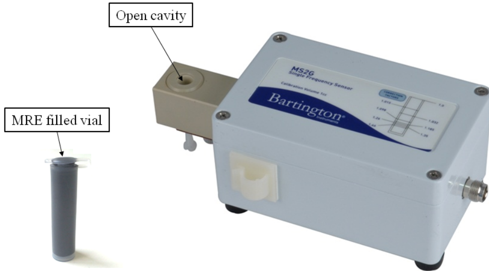
Figure 3.11: Photograph of an MRE-filled vial to be placed in the open cavity (surrounded by the coil) of the Bartington MS2G sensor to determine the initial volume susceptibility \chi of the material.
