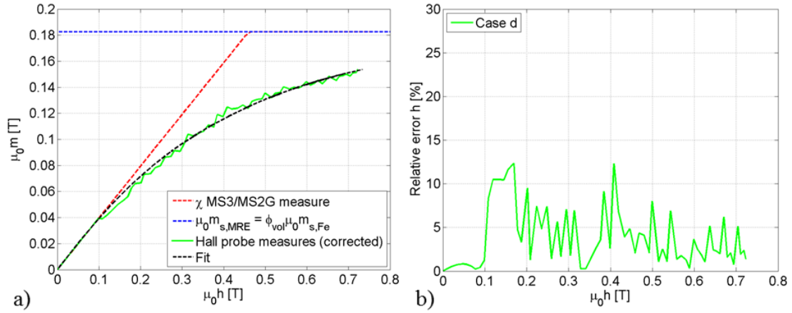
Figure 3.26: Case d for the isotropic 70 phr MRE: a) Magnetic response and least-squares fit. b) Relative error in the fit.
