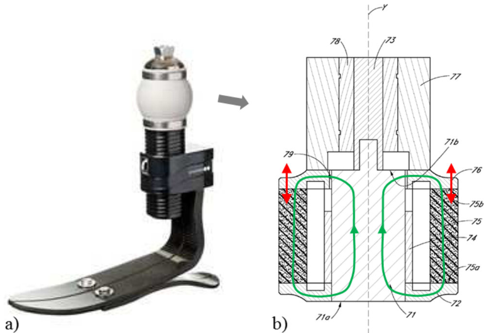
Figure 1.2: a) Picture of a smart prosthetic foot device and b) cross-section of the integrated tunable MRE spring [Tho13]. The motion (red arrows) resistance of the MRE spring (75) can be adjusted by the magnetic flux (green circuit) generated by the coil (74).
