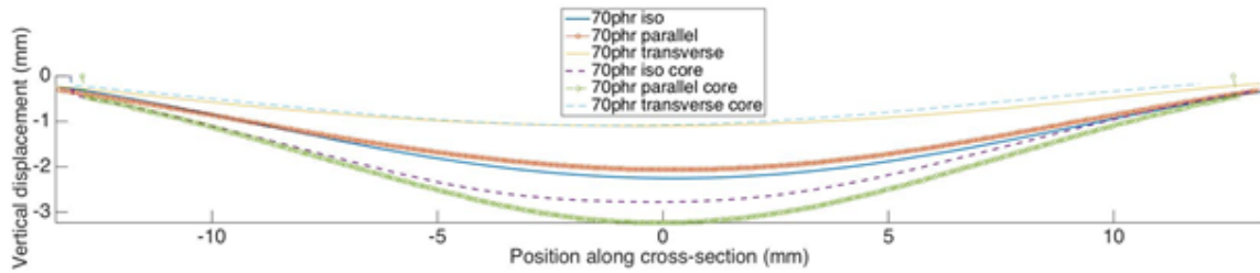
Figure 4.14: Vertical displacement profiles along the cross-section for all tested MRE disks.
