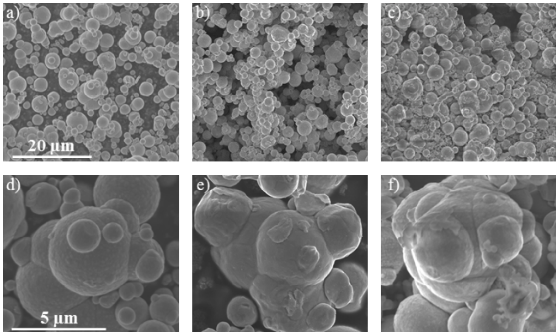
Figure 2.9: SEM micrographs of 3.5 \mu\text{m} median size carbonyl iron particles. Top: SEM micrographs ( 1,500\times ) of a) untreated particles, b) spray-coated particles and c) primer-stirred particles. Bottom: SEM micrographs ( 6,000\times ) of d) untreated particles, e) spray-coated particles and f) primer-stirred particles.
