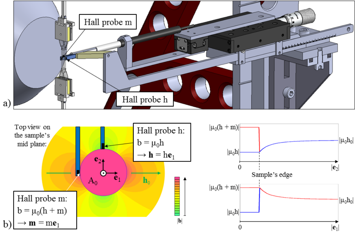
Figure 3.10: a) Stand coming from behind of the electromagnet and holding the two Hall probes h and m. b) On the left: FEM simulation (2D plane, [FEMM]) of the distribution of the magnetic field \mathbf{b} in the airgap of an electromagnet in the presence of a magnetic sample of circular cross-section having a homogeneous magnetization \mathbf{m} . On the right: evolution of the magnetic field \mathbf{b} along direction |\mathbf{e}_1| (bottom) and transverse to direction |\mathbf{e}_2| (top) covering the discontinuity interface sample/air.
