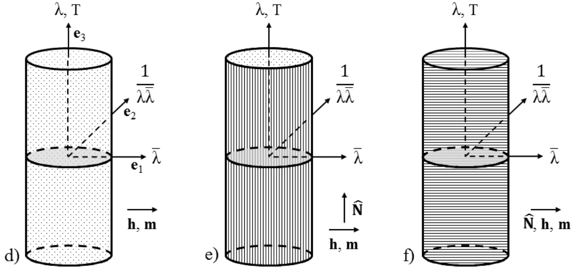
Figure 3.3: Schematic of the different test cases for the identification of the magneto-mechanical response T , h : d) isotropic MRE, e) transversely isotropic MRE with applied mechanical traction T along chain direction \widehat{\mathbf{N}} and f) transversely isotropic MRE with applied mechanical traction T transverse to chain direction \widehat{\mathbf{N}} .
