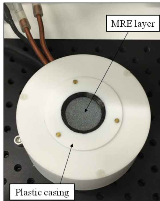
Figure 4.11: Photograph of the final prototype device showing the electromagnetic coil within an overall plastic casing and the MRE disk with applied speckle pattern installed on top of the coil at its center.
