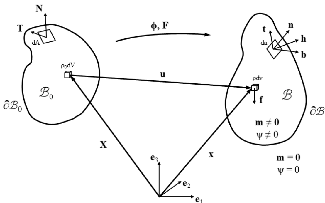
Figure 3.1: Summary schematic for the motion and deformation of an arbitrary magneto-elastic body \mathcal{B}_0 bounded by a closed surface \partial\mathcal{B}_0 in the undeformed, reference configuration into the deformed, current configuration \mathcal{B} , \partial\mathcal{B} due to the combined action of mechanical loads and a magnetic field (defined in what follows).
