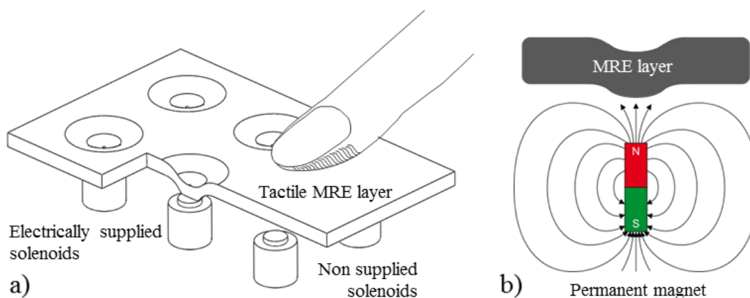
Figure 1.17: Schematics of the working principle for tactile interfaces with patterns created a) by a matrix of solenoids placed underneath a MRE layer or b) by a permanent magnet.
