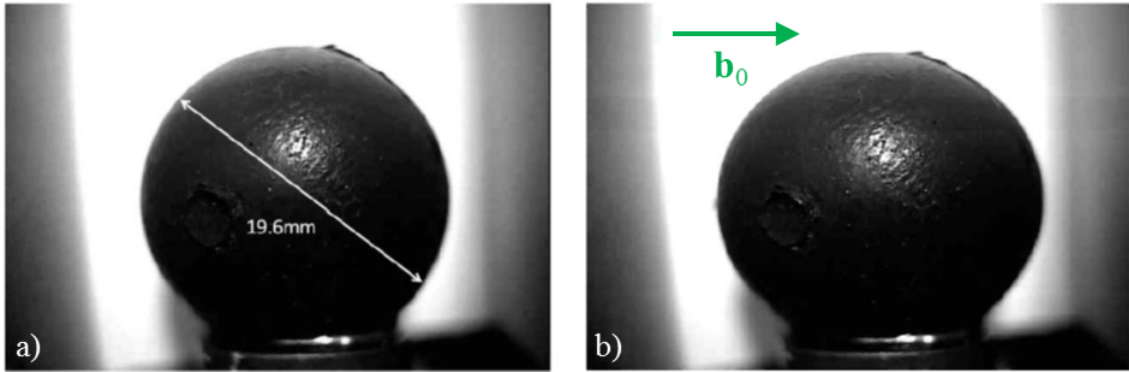
Figure 1.8: Photograph of an MRE sphere without a) and with b) an externally applied uniform field \mathbf{b}_0 = \mu_0 \mathbf{h}_0 = 1.2 T (green arrow). The applied field induces an elongation in the direction of the field of 4.8% at saturation ( E \approx 0.7 MPa ) [Dig10].
