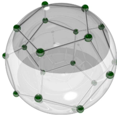
Figure 3.11: The Dodecahedron. |jD_i\rangle = \frac{1}{25^{\frac{1}{3}}} (\sqrt{187} |jS(20,0)\rangle + \sqrt{627} |jS(20,5)\rangle + \sqrt{247} |jS(20,10)\rangle + \sqrt{627} |jS(20,15)\rangle + \sqrt{187} |jS(20,20)\rangle) .
