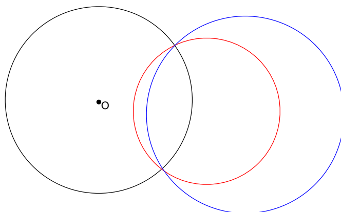
(c) A circle not through the origin (blue) is inverted to a circle not through the origin (red) and vice versa.
