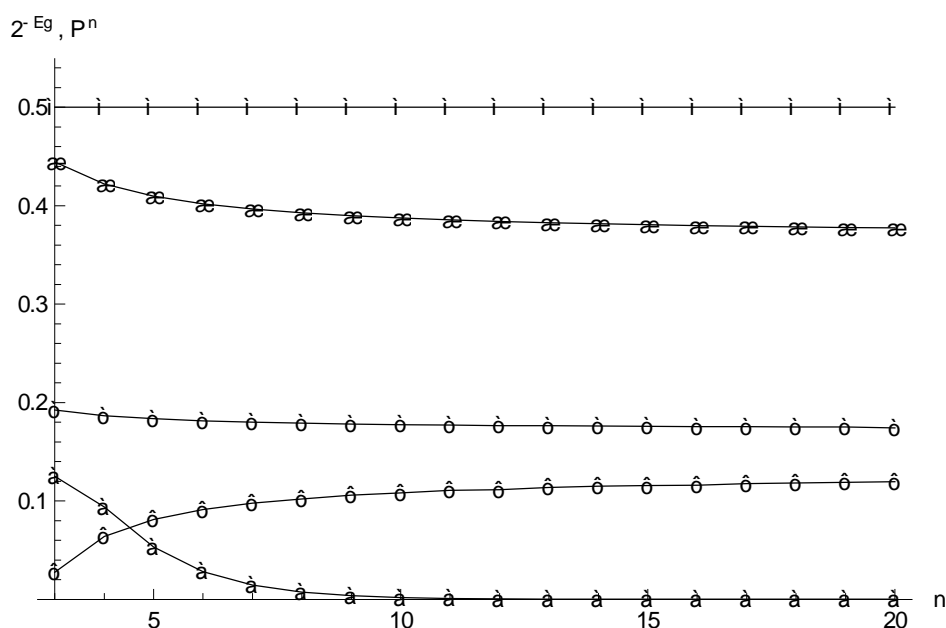
Figure 6.1: Violations of P^n by the state |jGHZ_n\rangle ( n ), with the numerical violations of P^n ( s ) and Q_{n-1}^n ( t ) of |jW_n\rangle as a function of n (number of parties), comparing to \frac{1}{2^{Eg(jW_n)}} ( l ) and \frac{1}{2^{Eg(jGHZ_n)}} ( u ).
