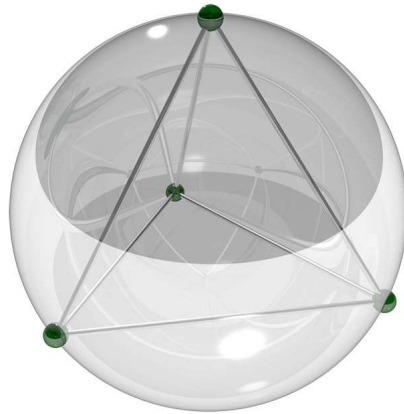
Figure 3.7: The Tetrahedron. |jT_i\rangle = \frac{\Delta}{3} |S(4,0)\rangle + \frac{\Delta}{3} |S(4,3)\rangle .
