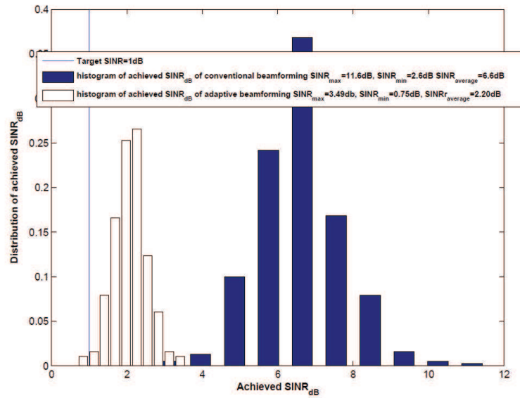
FIGURE 6.27 – Distribution of achieved SINR for adaptive beamforming and conventional beamforming. System settings : K = 380 , target SINR=1dB, \sigma_n^2 = -10 dBW, CIM=-15dB
