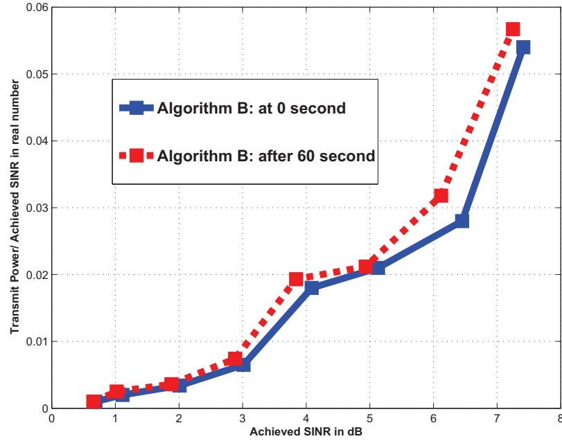
FIGURE 6.21 – Power/achieved SINR versus achieved SINR in one minute with perfect CSI at ST. System settings : K = 100 , \sigma_n^2 = -20\text{dBW} , \text{CIM} = -15\text{dB}
