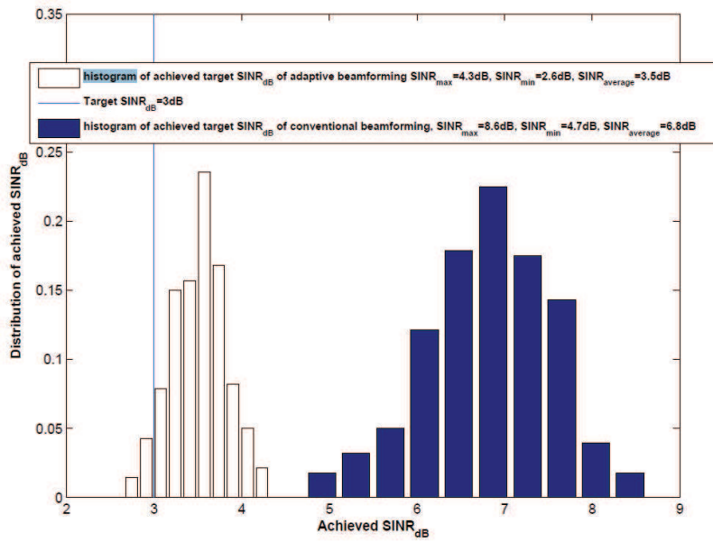
FIGURE 6.29 – Distribution of achieved SINR for adaptive beamforming and conventional beamforming. System settings : K = 280 , target SINR=3dB, \sigma_n^2 = -10 dBW, CIM=-15dB
