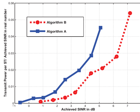
FIGURE 6.8 – Power/achieved SINR versus achieved SINR for Algorithm A and B. System settings : K = 100 , \sigma_n^2 = -20 dBW, CIM= -15 dB
