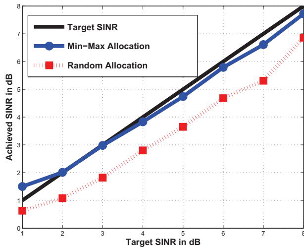
FIGURE 10.13 – Achieved SINR in dB versus target SINR in dB when applying different carrier allocation algorithms. System settings : K = 400 , \sigma_n^2 = -10\text{dBW} , CIM = -15dB, training length= 200
