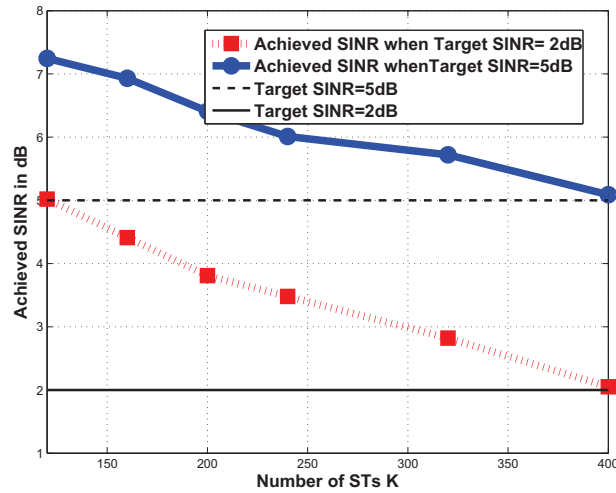
FIGURE 10.19 – Achieved SINR in dB versus number of STs K . System settings : \sigma_n^2 = -10\text{dBW} , CIM=15dB, training length= 400
