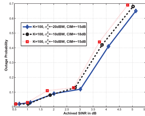
FIGURE 6.18 – The outage probability versus achieved SINR for Algorithm B for different levels of noise and intermodulation noise. System settings : K = 100
