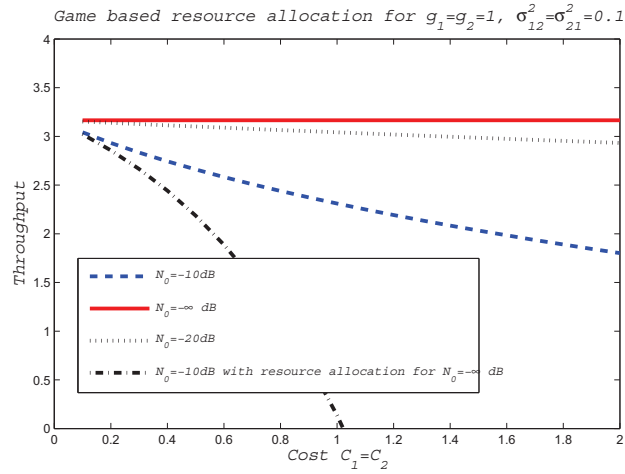
FIGURE 12.6 – Throughput attained at the Nash equilibrium versus costs C_1 = C_2 for different values of the noise.
