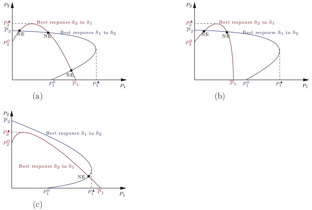
FIGURE 12.1 – Possible Nash equilibrium set for game \mathcal{G}_{\mathcal{P}}
