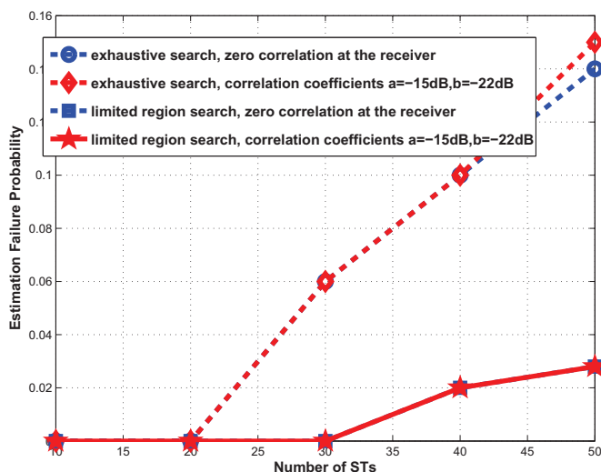
FIGURE 7.8 – Estimation failure probability versus number of STs for different correlation coefficients at the receiver with different pilot lengths and searching area. System settings : Noise= -\infty dBW, Q = 30 , pilot length=150
