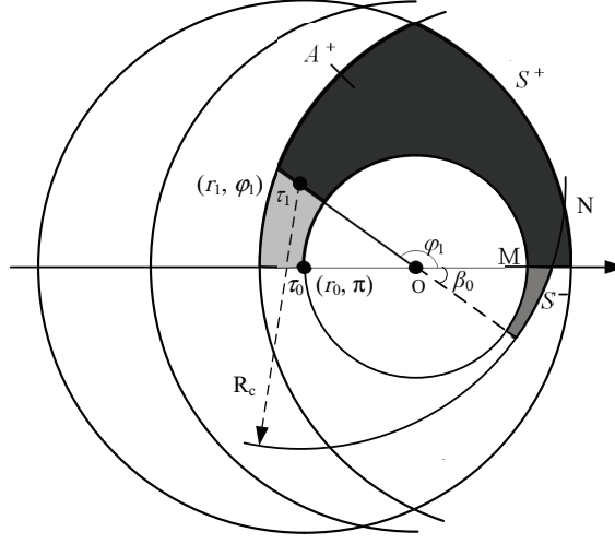
Figure A.4: Illustration of R_2(r_0, r_1, \varphi_1, 0)
