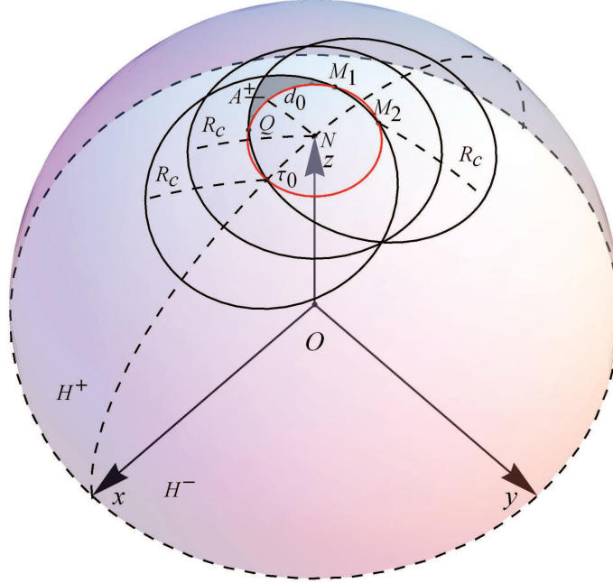
Figure 4.4: Illustration of region A^+ in the case R \arccos([3 \cos^2(R_s/R) - 1]/2) < R_c \leq 2R_s
