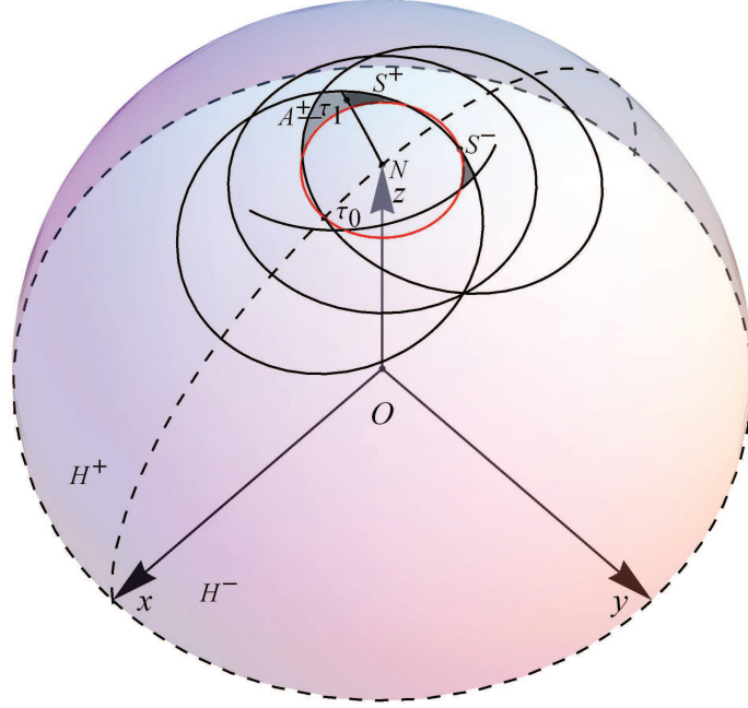
Figure 4.5: Illustration of regions S^+ and S^- in the case R \arccos([\frac{3}{2} \cos^2(R_s/R) - 1]) < R_c \leq 2R_s
