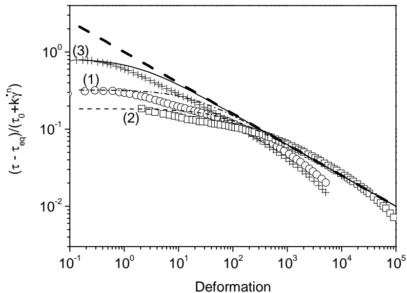
Figure 6.9. Comparison of the dimensionless shear stress between measured data (symbols) and predicted by the model (discontinuous lines) shifted for matching the initial measured stress value of each experiment protocol described in Section 5.7. The bold dashed line show the model predictions for the tests after static cooling of Section 6.4.
