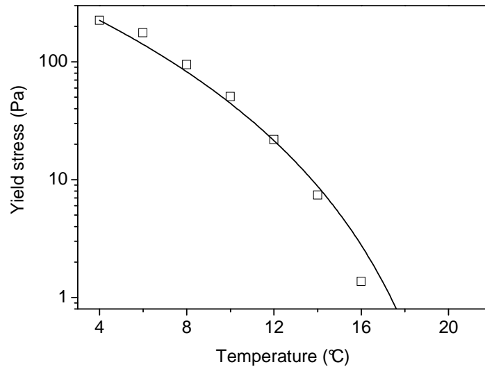
Figure 7.19. Symbols are the yield stress after cooling rate of -1 °C/min and holding time of 20 min and the line represents the respective fitting given by Eq. (7.1).
