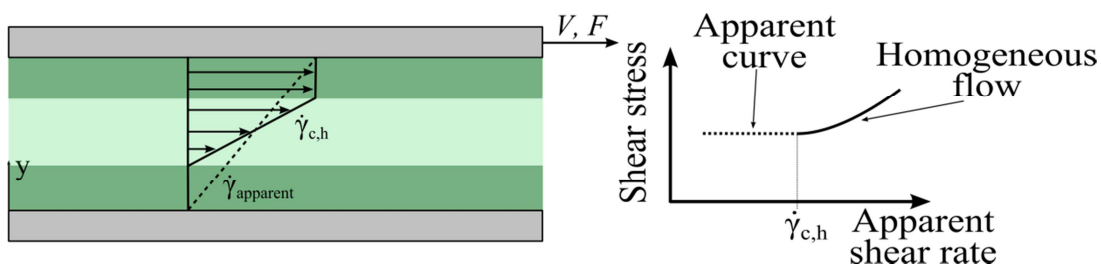
Figure 2.7. Fluids with unstable flow for an apparent shear rate below a critical shear rate \dot{\gamma}_{c,h} induce heterogeneous velocity profile, as shear banding, creating an apparent flow curve.
