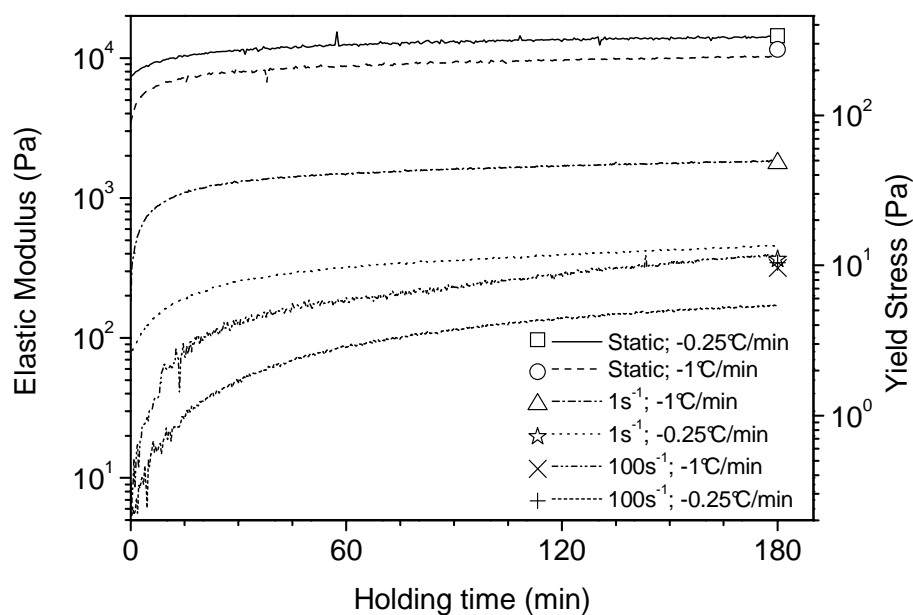
Figure 7.15. Elastic modulus evolution during holding time after cooling at 0, 1 and 100\text{ s}^{-1} and for cooling rates of -1 and -0.25\text{ }^{\circ}\text{C}/\text{min} with the respective yield stress measured in the sequence.
