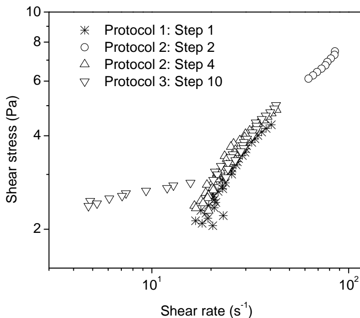
Figure 4.23. Flow curves at the starting 100 rpm steps of Protocol 1 (stars) and 2 (circles), and after high shear in Protocols 2 (up triangles) and 3 (down triangles).
