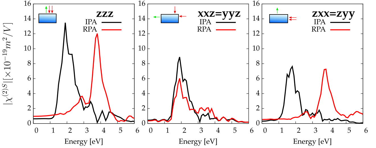
Fig. 9.4: Surface second-harmonic generation spectra of the dihydride Si(001)1x1:2H surface, for the zzz , xxz and zxx components of the \chi^{(2)S} tensor. No scissors correction is included.
