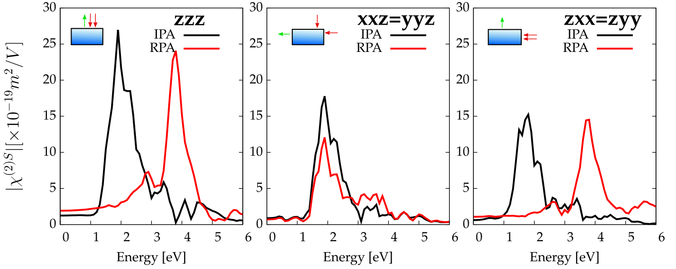
Fig. 9.4: Surface second-harmonic generation spectra of the dihydride Si(001)1×1:2H surface, for the zzz , xxz and zxx components of the \chi^{(2)S} tensor. No scissors correction is included.
