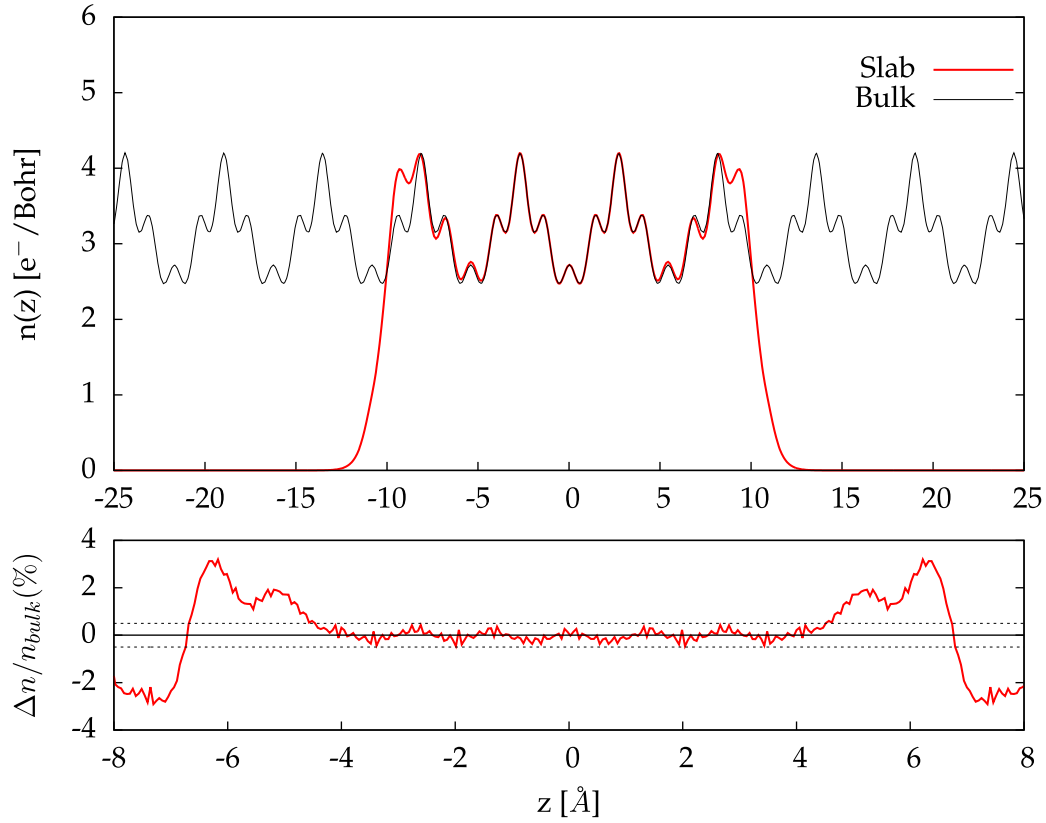
Fig. 5.9: Top panel: Variation of the number of electrons par Bohr along the z direction. This value is obtained by averaging the electronic density in the x-y plan for the entire cell. Bottom panel: relative differences between the bulk and the slab densities of the above panel. Note the change in the scale. The slab is composed of 16 atomic layers in total, with asymmetric dimers as surface reconstruction on both sides.
