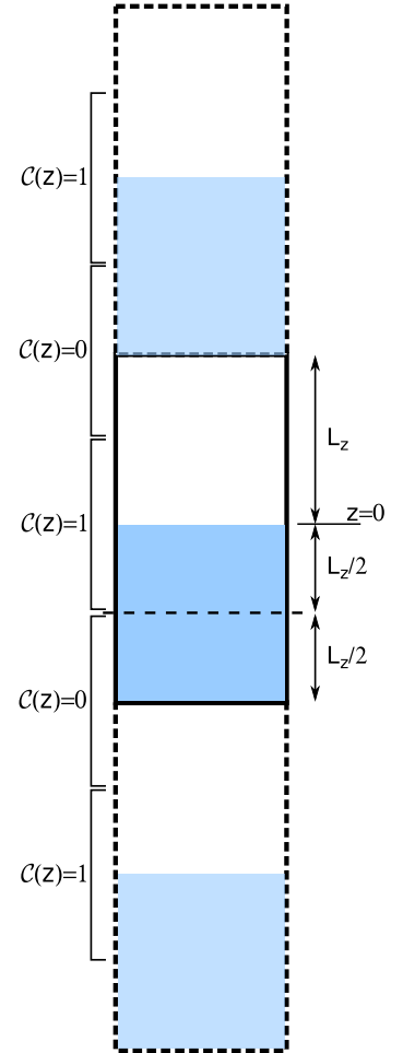
Fig. 7.1: The \mathcal{C}(z) function.
