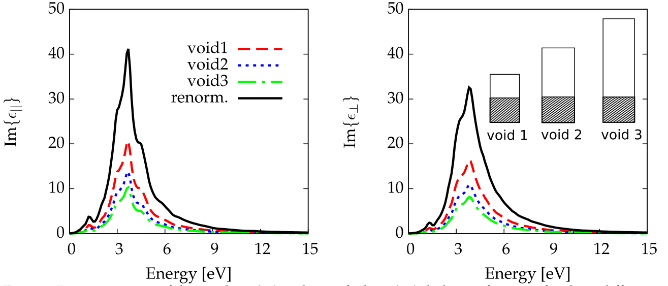
Fig. 8.2: Imaginary part of the in-plane ( \epsilon_{||} ) and out-of-plane ( \epsilon_{\perp} ) dielectric function for three different sizes of the super-cell. Local field effects are not included. The three super-cells are sketched in inset of the right panel.
