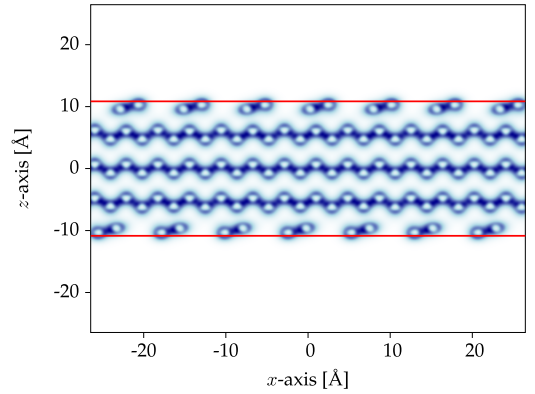
Fig. 8.1: Electronic density of a slab with two Si(001)2×1 surfaces, in the x-z plan [230].
