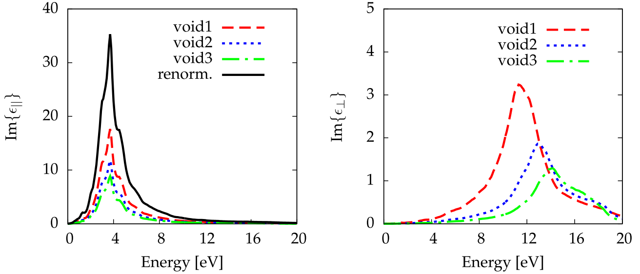
Fig. 8.3: Imaginary part of the in-plane ( \epsilon_{||} ) and out-of-plane ( \epsilon_{\perp} ) dielectric function for three different sizes of the super-cell. Local field effects are included. Note the change in the scale for the right panel.
