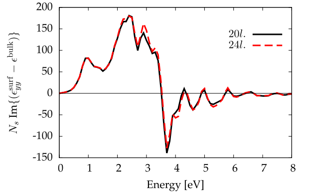
Fig. 8.12: Spectra of N_s(\epsilon_{\text{surf}}^s(\omega) - \epsilon_M^{\text{bulk}}(\omega)) for the clean surface, calculated for N = 20 layers (black solid line) and N = 24 layers (red dashed line).
