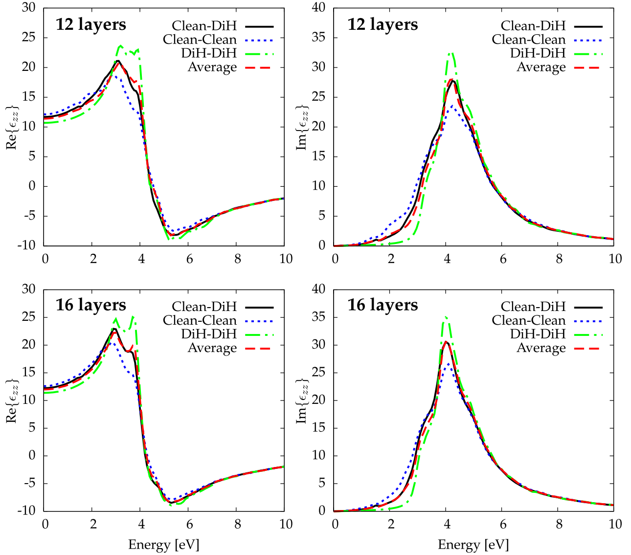
Fig. 8.9: Comparison between the real part (left panel) and imaginary part (right panel) of \epsilon_{zz} computed for the asymmetric slab (Clean-DiH; solid curve), a symmetric clean slab (Clean-Clean; blue dotted curve), a symmetric dihydride slab (DiH-DiH; green dotted dashed curve) and from the average of the two symmetric slabs (Average; dashed curve). Local field effects are included.
