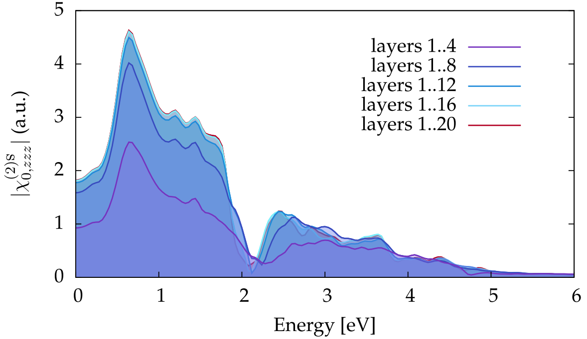
Fig. 5.8: Layer-by-layer analysis of the |\chi_{0,zzz}^{(2)S}| for the clean Si(001)2×1 surface.
