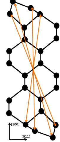
Fig. 5.2: A symmetric slab exhibits an artificial centro-symmetry
