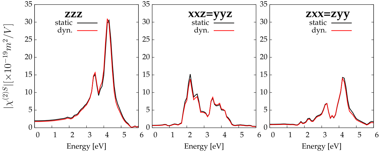
Fig. 10.4: Comparison between the effects of the static and the dynamic long-range contribution kernels on the surface second-harmonic generation of the dihydride surface. Black lines: static kernel f_{xc} = \frac{\alpha}{q^2} , with \alpha = -0.2 . Red lines: dynamic kernel f_{xc}^{\text{dyn}} = \frac{1}{q^2}(\alpha + \beta\omega^2) , with \alpha = -0.13 and \beta = -6.35 \times 10^{-3} eV.
