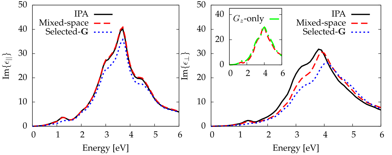
Fig. 8.7: Imaginary part of the dielectric function \epsilon_{||} with \mathbf{q} aligned along the x -axis (left panel) and \epsilon_{\perp} (right panel). Black solid curves: Independent-particle approximation (IPA). Red dashed curves: Mixed-space calculation. Blue dotted curves: Selected-G calculation. Inset: Comparison between the mixed-space and the Selected-G method, without in-plane reciprocal vectors (" G_z -only", green dotted-dashed curve).
