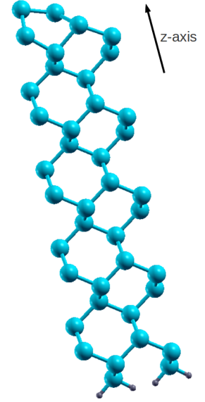
Fig. 5.3: A slab with an front clean Si(001)2×1 surface and a back dihydride surface. The dangling bonds are H (small balls) saturated. This image depicts 20 Si atomic layers with one H atomic layer.
