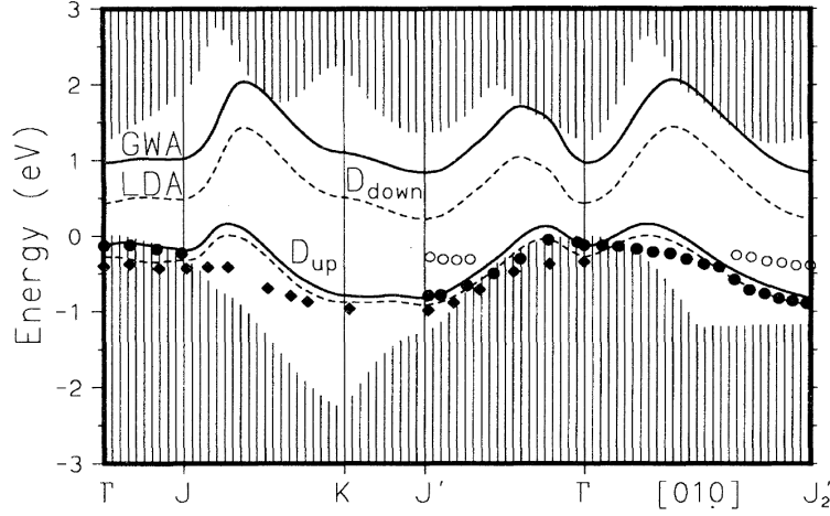
Fig. 6.1: Calculated surface states of Si(001)2×1 using LDA (dashed lines) and GW (solid lines). Symbols corresponds to photoemission experiments [215]. Reproduced from [215].
