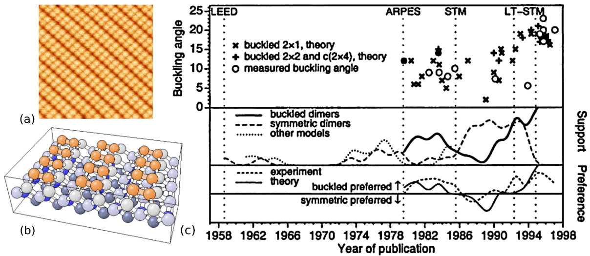
Fig. 4.3: (a) Atomic Force Microscope (AFM) image of the clean Si(001)2×1 surface, from Ref. [162]. (b) Schematic view of the Si(001)2×1 surface. Picture from NIST Surface Structure Database. (c) Evolution of opinions about the structure of clean Si(001) surface, taken from Ref. [163]. Symmetric dimers dominates between the first observation of mostly symmetric dimers at room temperature (1985) and first observation of mostly buckled dimers at low temperature (1992). In the upper panel, the value of the buckling angle obtained from theoretical and experimental studies is reported, with a clear correlation. The middle panel report the support for each model, measured by the number of published papers. The theoretical and experimental preference (lower panel) is measured by the difference between the number of papers supporting either model.
