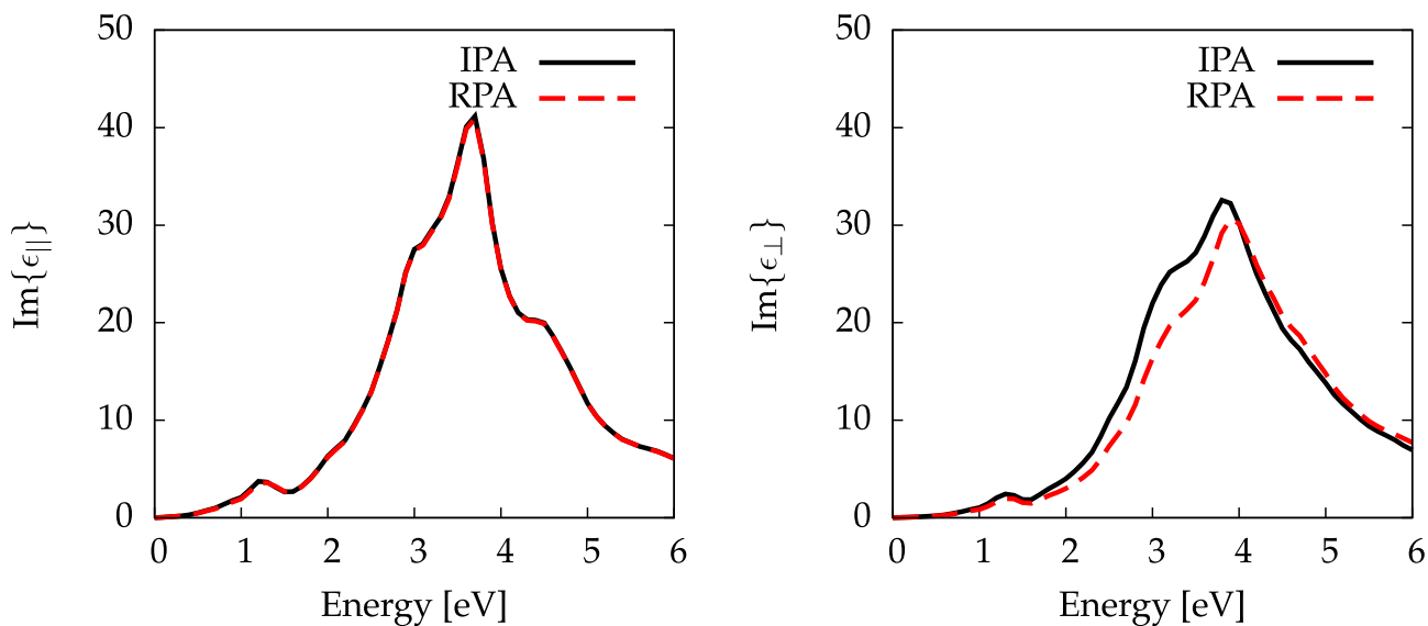
Fig. 8.5: Imaginary part of the dielectric function, computed using the mixed-space scheme. Black curves: Independent-particle approximation (IPA). Red curves: Random-phase approximation. Left panel: Imaginary part of \epsilon_{||} with \mathbf{q} align along the x -axis. Right panel: Imaginary part of \epsilon_{\perp} .
