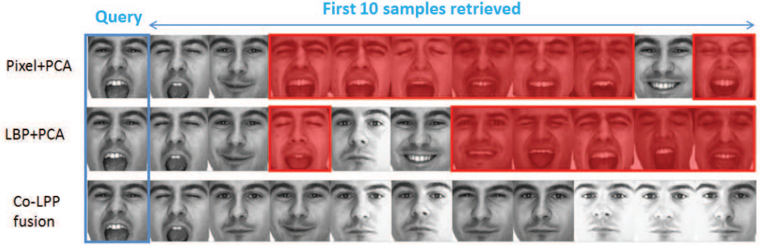
Figure 6.4: Comparison of retrieval results using only pixel features (first row), LBP features (second row) and proposed Co-LPP retrieval scheme. Faces in red indicate incorrect retrieved images.
