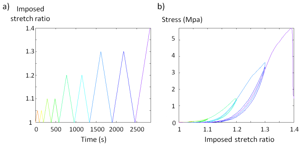
Figure III.14 – Typical cycling experiment with no SHG observation: a) loading path, b) stress/stretch curve.
