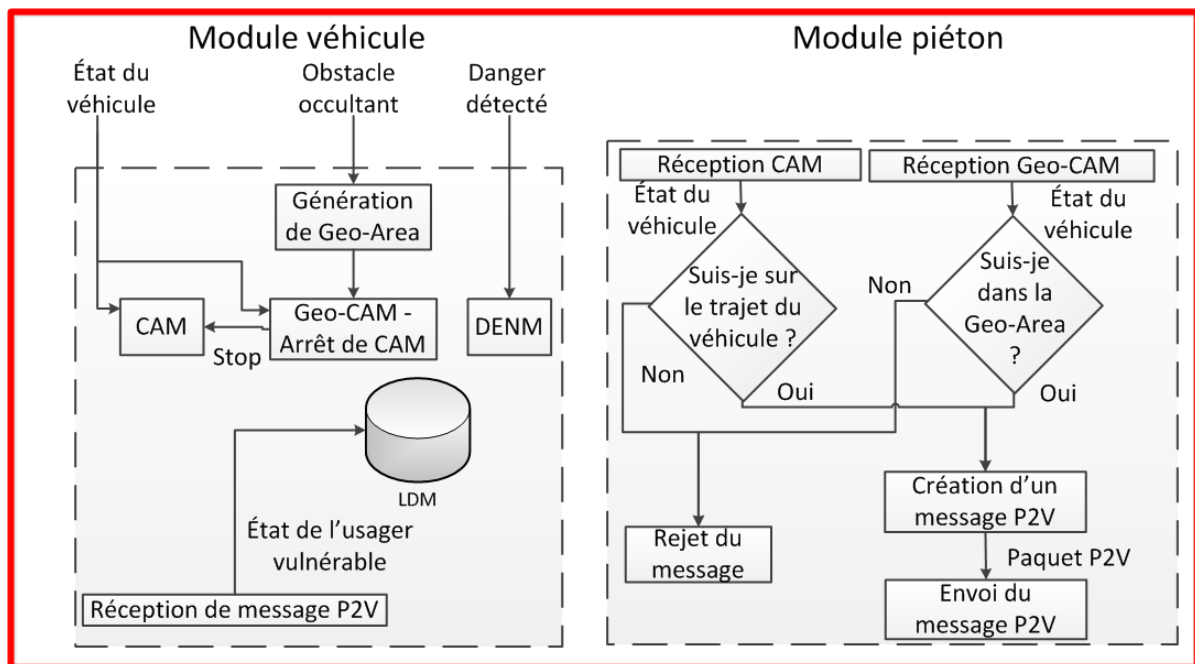
FIGURE 4.3: Architecture de la communication V2P
