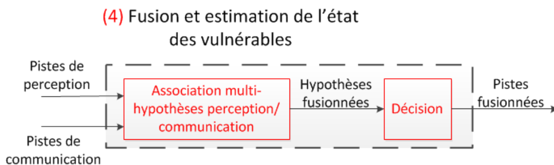
FIGURE 5.4: Architecture de la fusion d'information perception/communication
