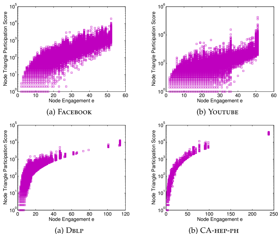
Figure 3.9: Node engagement vs. triangle participation score. Correlation of the node engagement index with the number of triangles that each node participates to.
