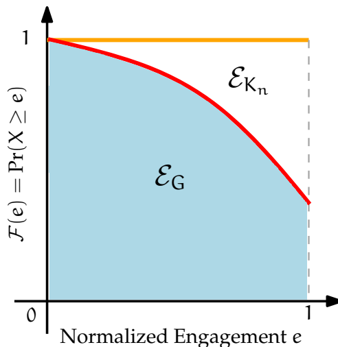
Figure 3.2: Schematic representation of the engagement index \mathcal{E}_G . The red curve shows an example of the complementary cumulative distribution function of the engagement level of the k -engagement subgraphs. The area under the curve (light blue region) captures the engagement properties of the graph. The orange colored curve shows the engagement level of the complete graph K_n .
